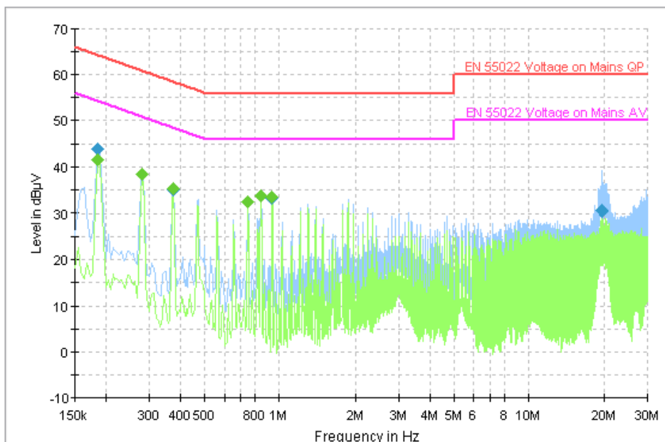
Figure A.12 Conducted Emission
