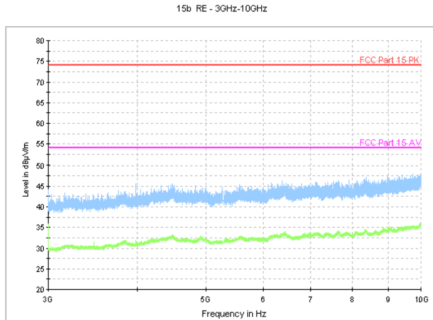
Figure A.9 Radiated Emission from 3GHz to 10GHz
