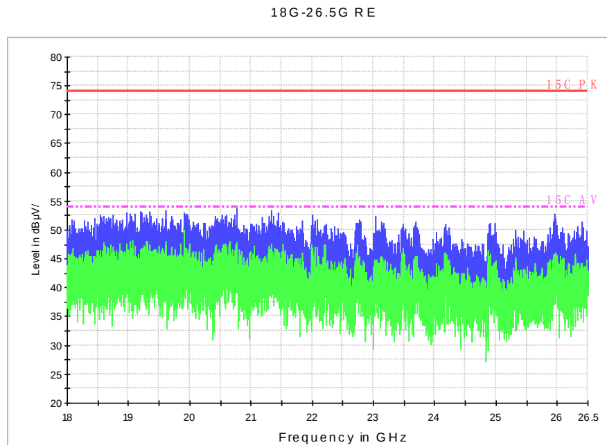
Fig. 54 Radiated Spurious Emission (802.11n-HT20, ch40, 18 GHz-26.5 GHz)
