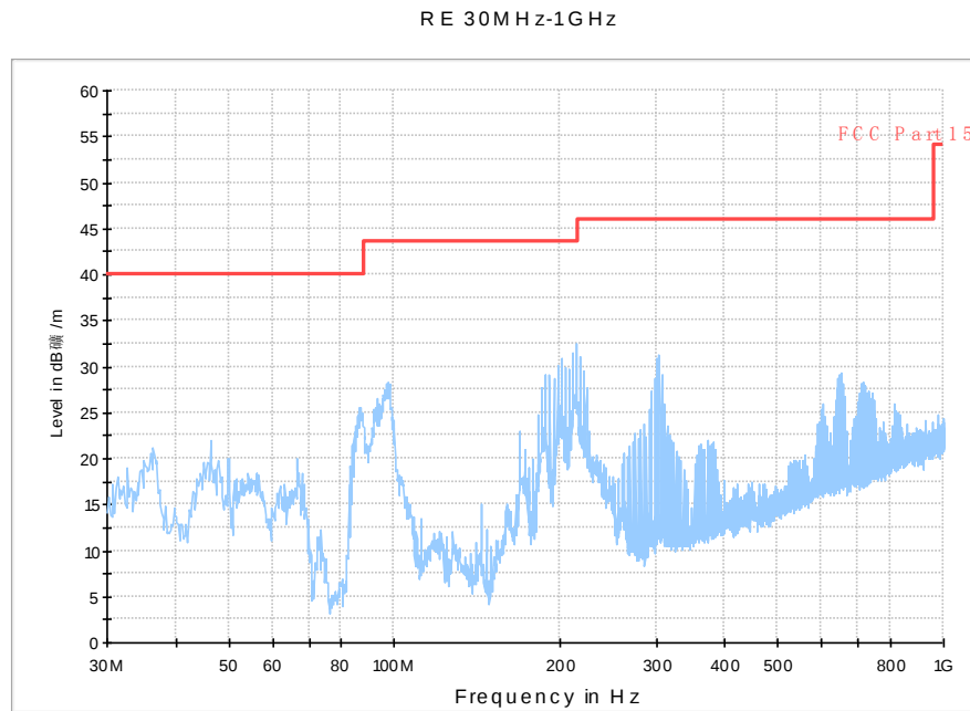
Fig. 44 Radiated Spurious Emission (802.11n-HT20, ch36, 30 MHz-1 GHz)
