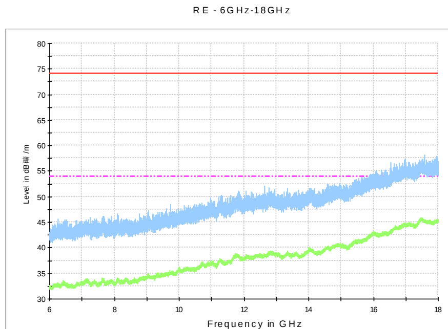
Fig. 47 Radiated Spurious Emission (802.11n-HT20, ch36, 6 GHz-18 GHz)
