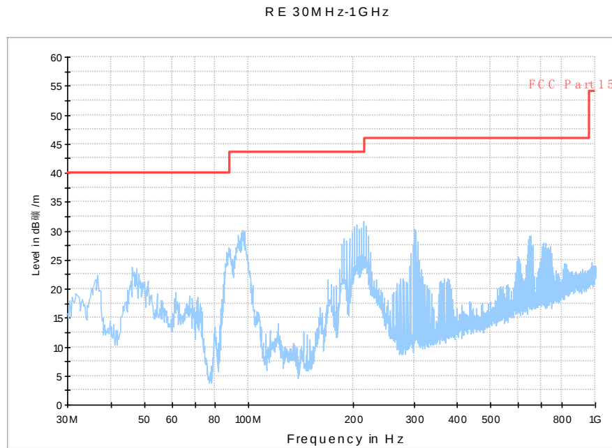
Fig. 50 Radiated Spurious Emission (802.11n-HT20, ch40, 30 MHz-1 GHz)
