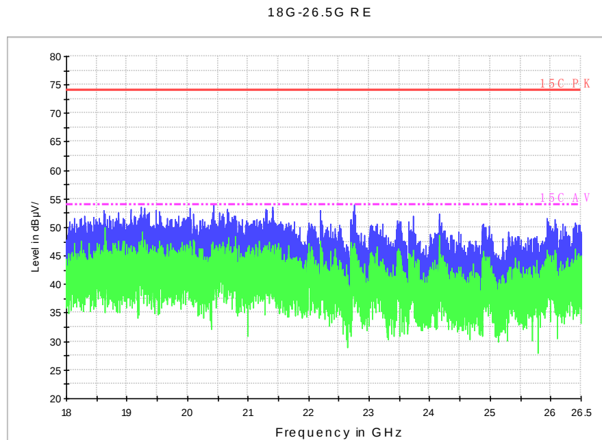
Fig. 30 Radiated Spurious Emission (802.11a, ch36, 18 GHz-26.5 GHz)
