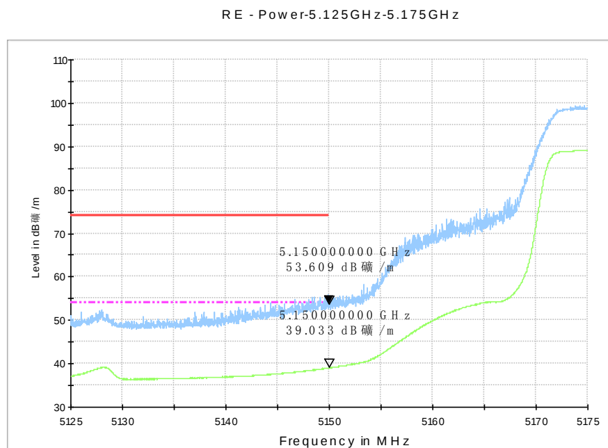
Fig. 24 Band Edges (802.11n-HT20, 5180MHz)
