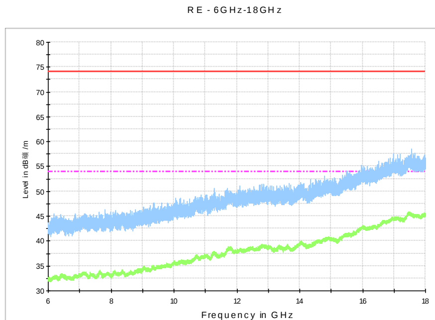
Fig. 59 Radiated Spurious Emission (802.11n-HT20, ch48, 6 GHz-18 GHz)
