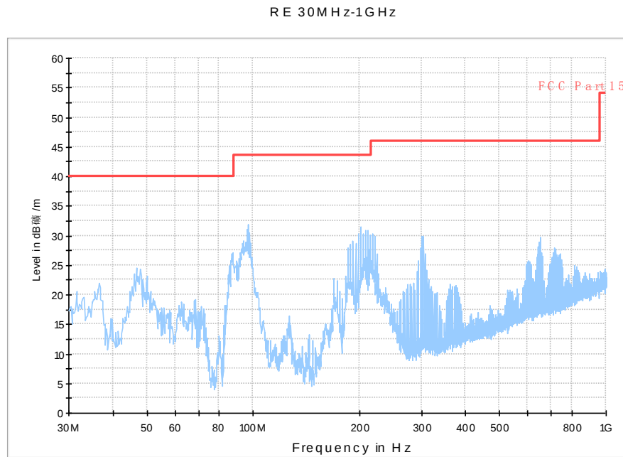
Fig. 56 Radiated Spurious Emission (802.11n-HT20, ch48, 30 MHz-1 GHz)
