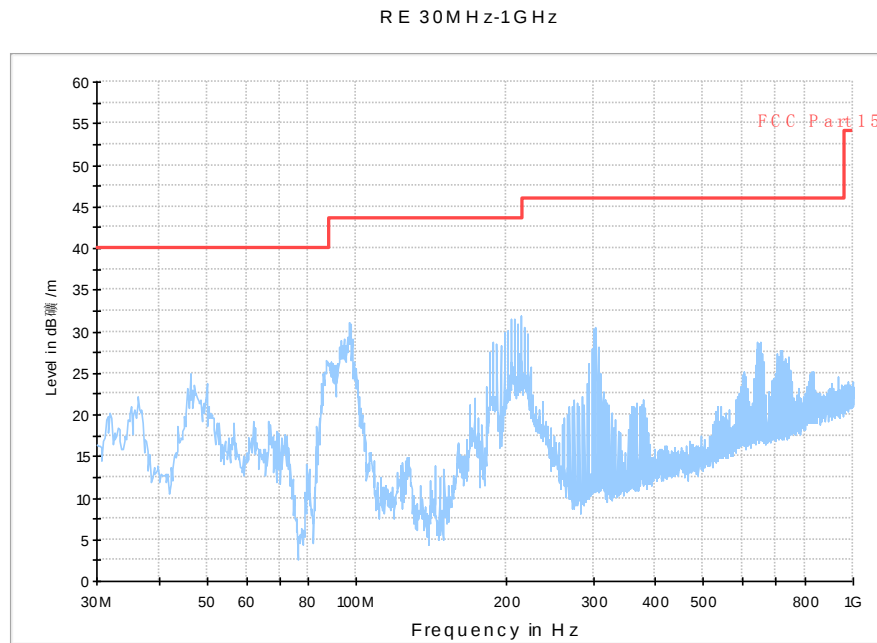
Fig. 68 Radiated Spurious Emission (802.11n-HT40, ch46, 30 MHz-1 GHz)
