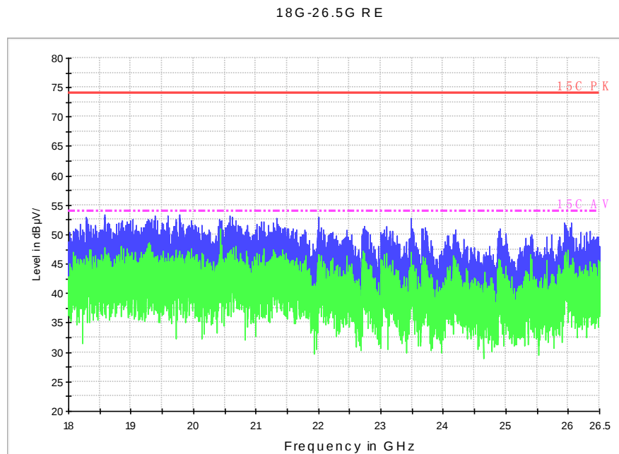
Fig. 36 Radiated Spurious Emission (802.11a, ch40, 18 GHz-26.5 GHz)
