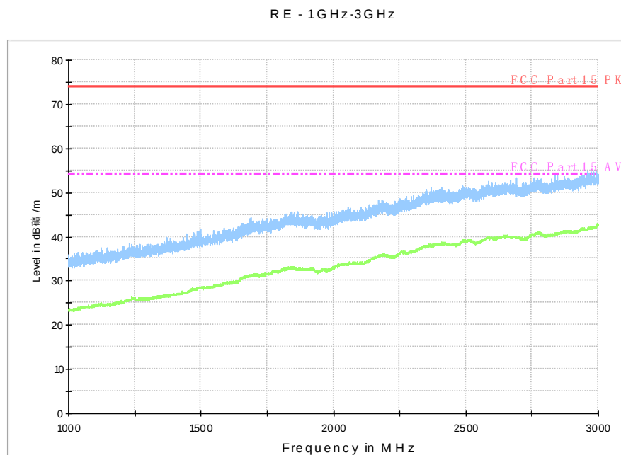
Fig. 39 Radiated Spurious Emission (802.11a, ch48, 1 GHz-3 GHz)
