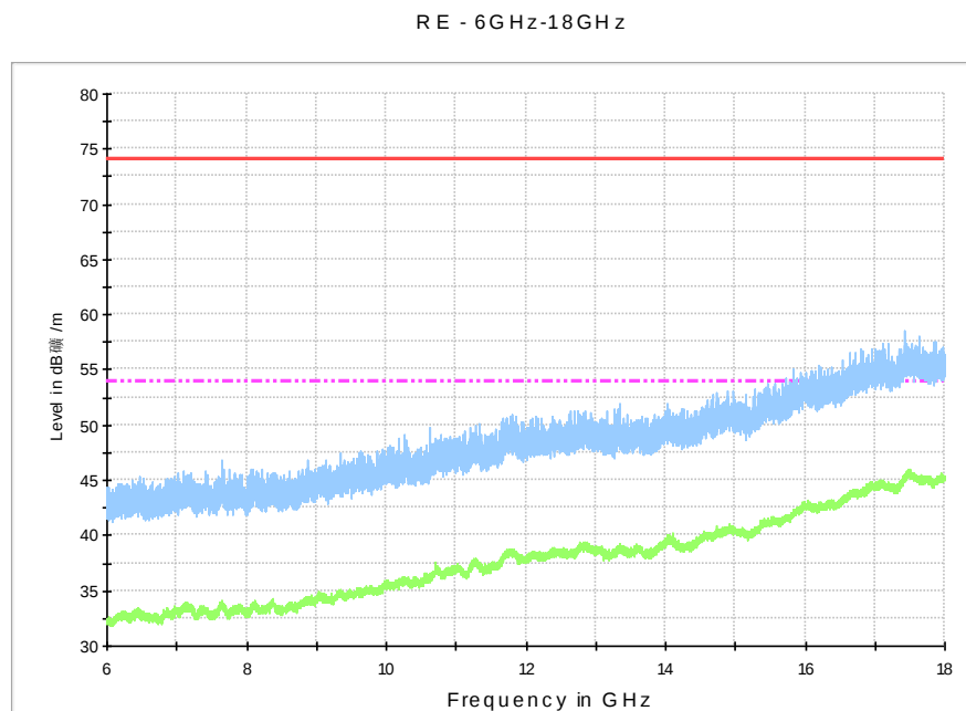
Fig. 53 Radiated Spurious Emission (802.11n-HT20, ch40, 6 GHz-18 GHz)
