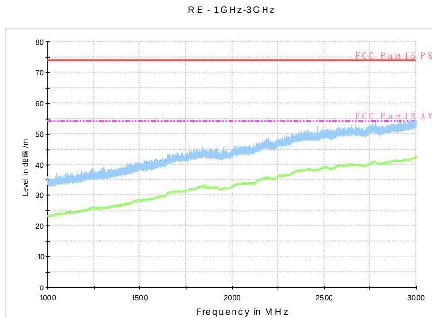
Fig. 57 Radiated Spurious Emission (802.11n-HT20, ch48, 1 GHz-3 GHz)
