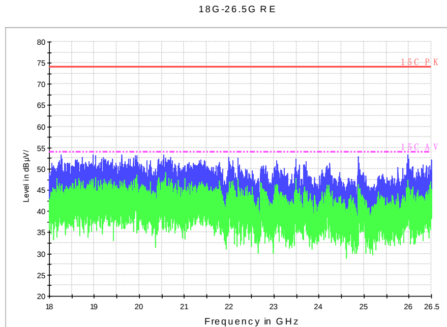
Fig. 48 Radiated Spurious Emission (802.11n-HT20, ch36, 18 GHz-26.5 GHz)
