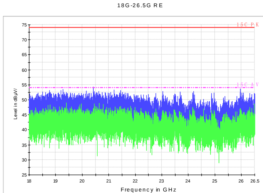
Fig. 72 Radiated Spurious Emission (802.11n-HT40, ch46, 18 GHz-26.5 GHz)
