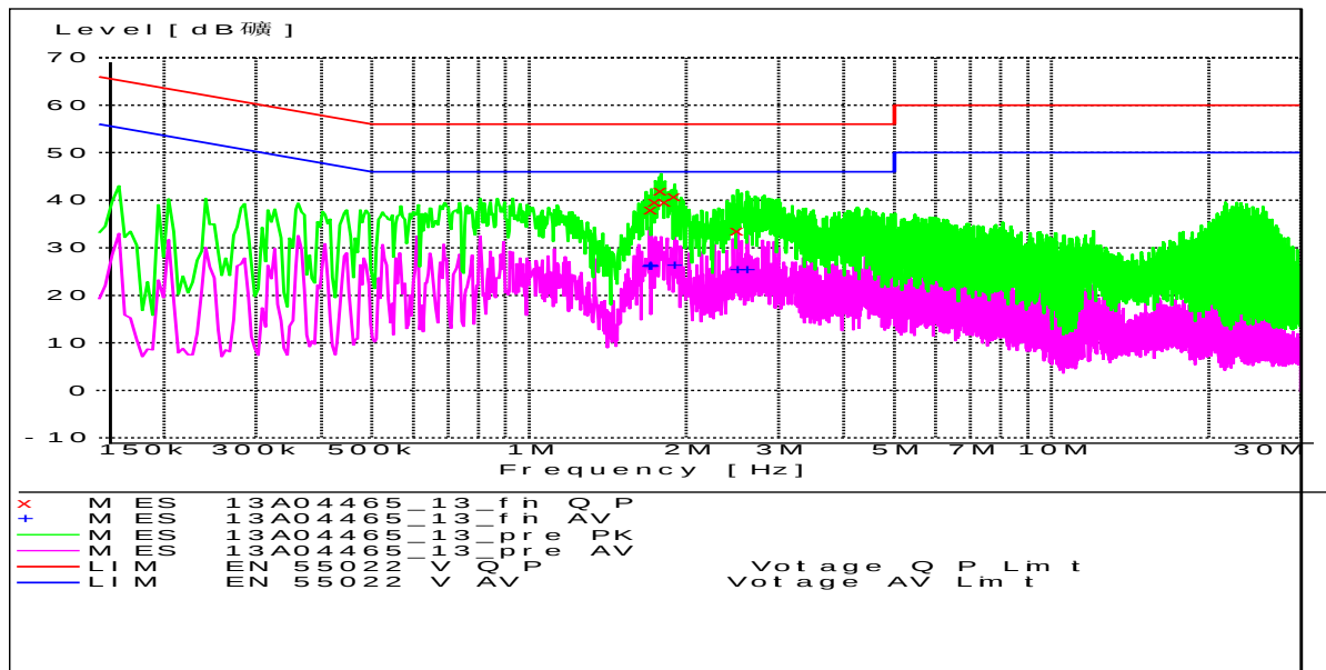
Fig. 75 Conducted Spurious Emission(802.11a, IDLE)
