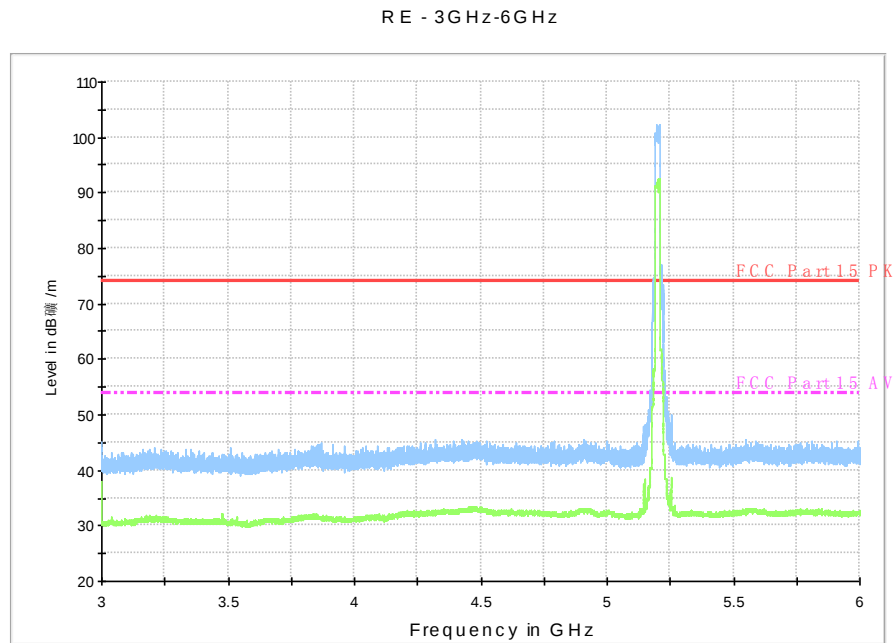
Fig. 34 Radiated Spurious Emission (802.11a, ch40, 3 GHz-6 GHz)
