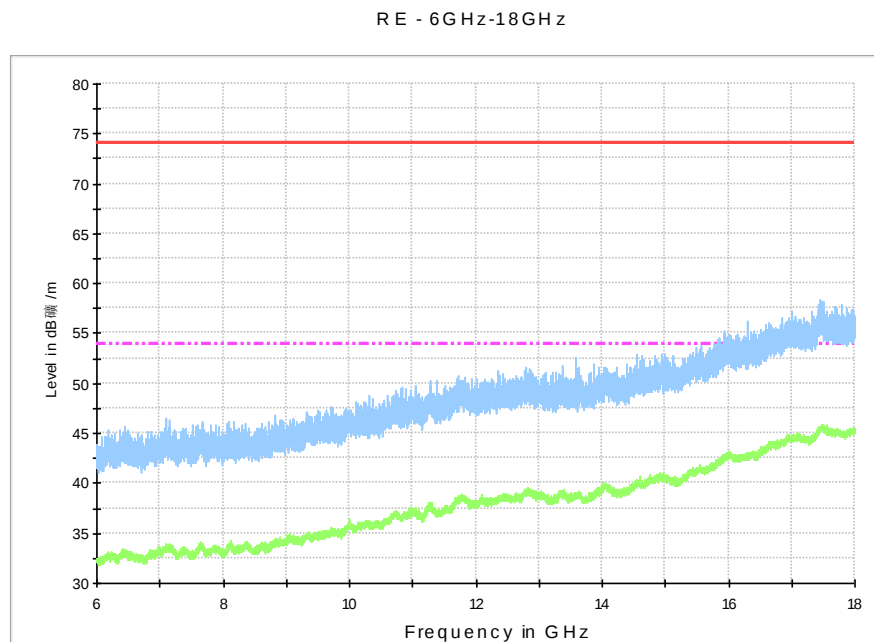
Fig. 35 Radiated Spurious Emission (802.11a, ch40, 6 GHz-18 GHz)
