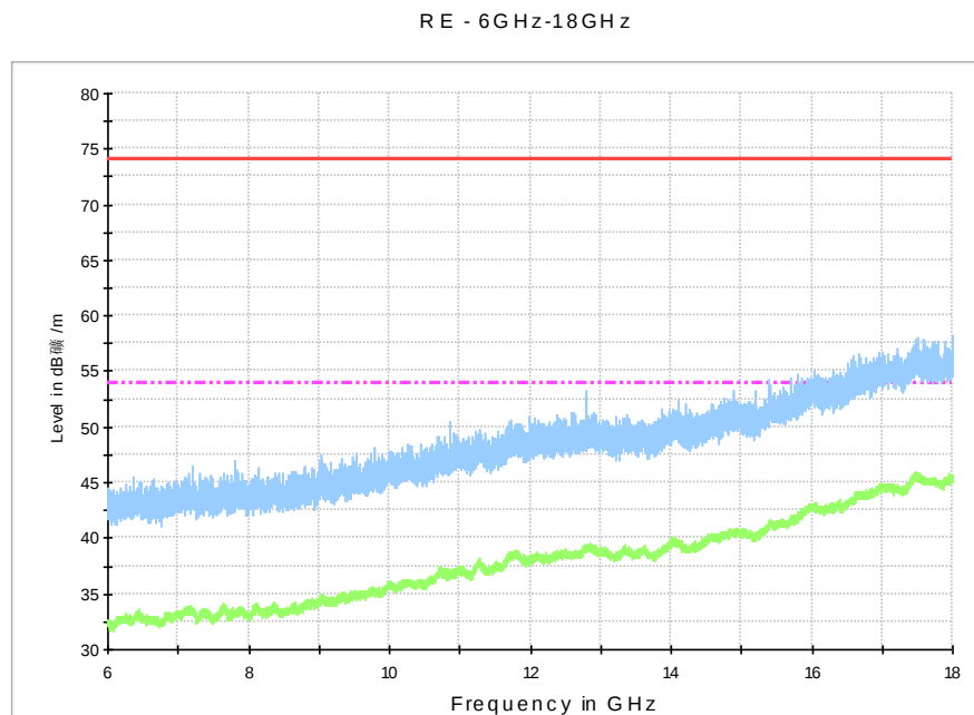
Fig. 29 Radiated Spurious Emission (802.11a, ch36, 6 GHz-18 GHz)
