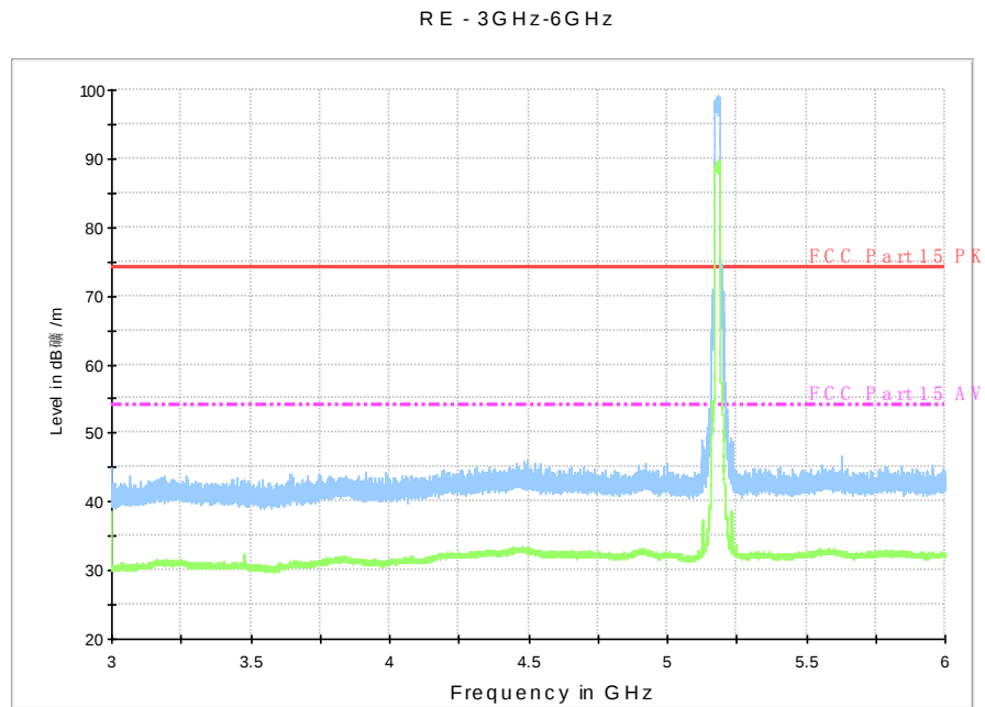
Fig. 46 Radiated Spurious Emission (802.11n-HT20, ch36, 3 GHz-6 GHz)
