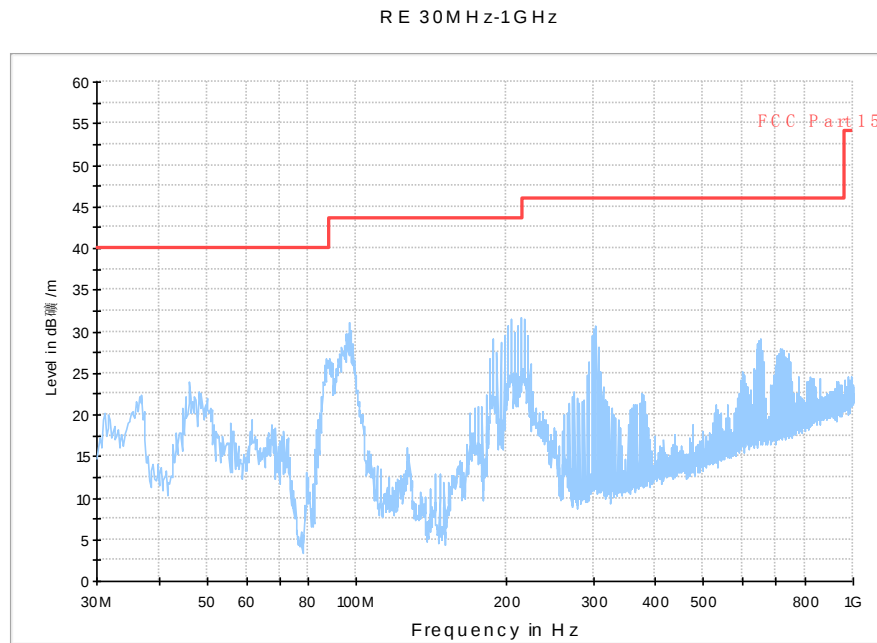
Fig. 62 Radiated Spurious Emission (802.11n-HT40, ch38, 30 MHz-1 GHz)
