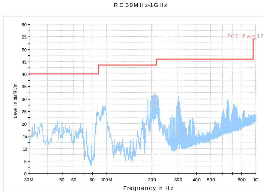
Fig. 26 Radiated Spurious Emission (802.11a, ch36, 30 MHz-1 GHz)
