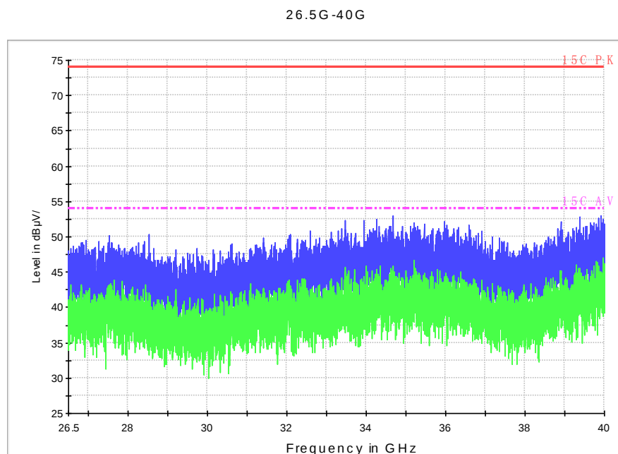
Fig. 61 Radiated Spurious Emission (802.11n-HT20, ch48, 26.5 GHz-40 GHz)
