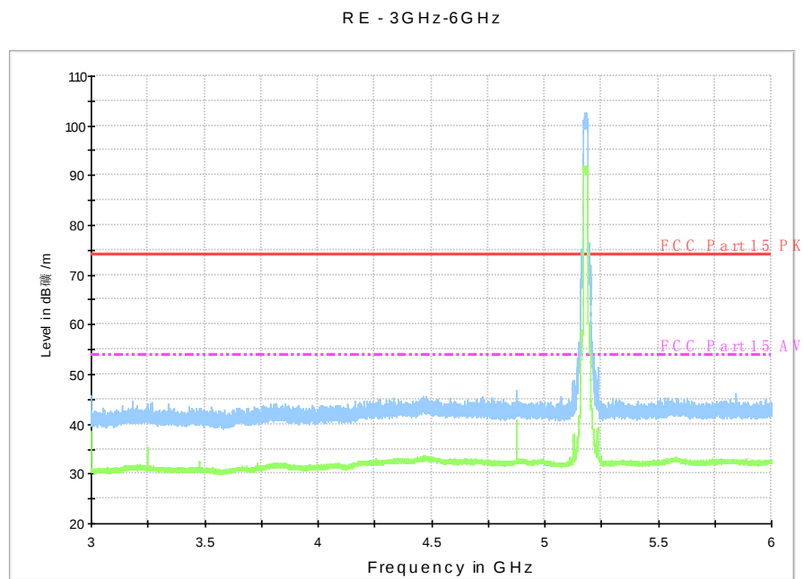
Fig. 28 Radiated Spurious Emission (802.11a, ch36, 3 GHz-6 GHz)
