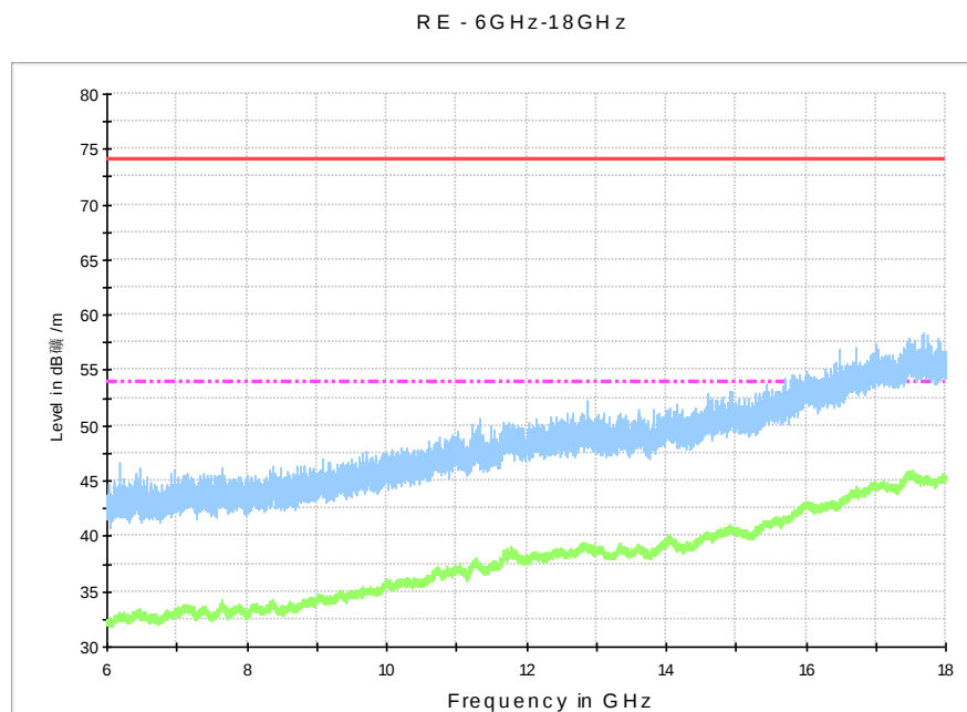
Fig. 41 Radiated Spurious Emission (802.11a, ch48, 6 GHz-18 GHz)
