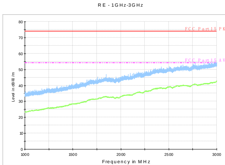
Fig. 33 Radiated Spurious Emission (802.11a, ch40, 1 GHz-3 GHz)
