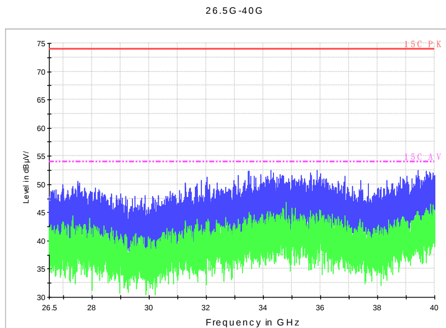
Fig. 49 Radiated Spurious Emission (802.11n-HT20, ch36, 26.5 GHz-40 GHz)
