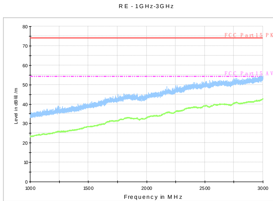
Fig. 51 Radiated Spurious Emission (802.11n-HT20, ch40, 1 GHz-3 GHz)
