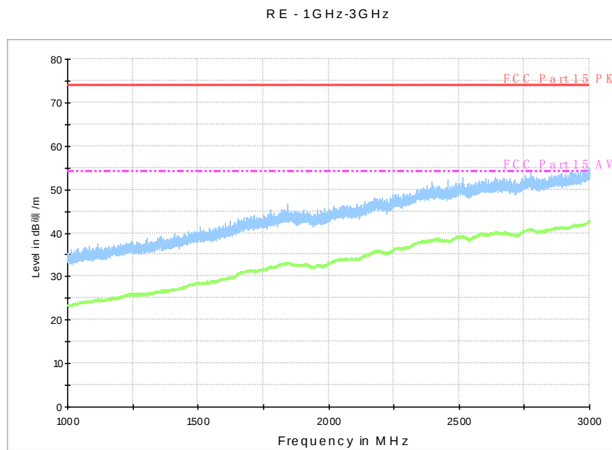
Fig. 69 Radiated Spurious Emission (802.11n-HT40, ch46, 1 GHz-3 GHz)
