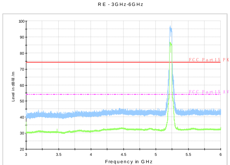
Fig. 70 Radiated Spurious Emission (802.11n-HT40, ch46, 3 GHz-6 GHz)
