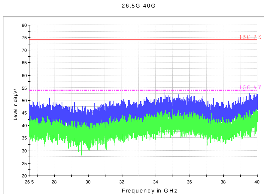
Fig. 31 Radiated Spurious Emission (802.11a, ch36, 26.5 GHz-40 GHz)
