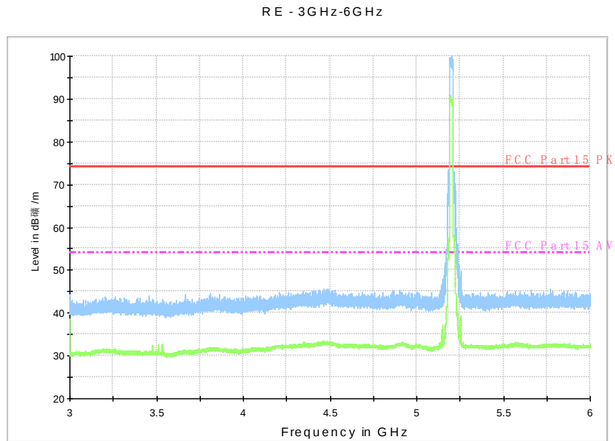
Fig. 52 Radiated Spurious Emission (802.11n-HT20, ch40, 3 GHz-6 GHz)
