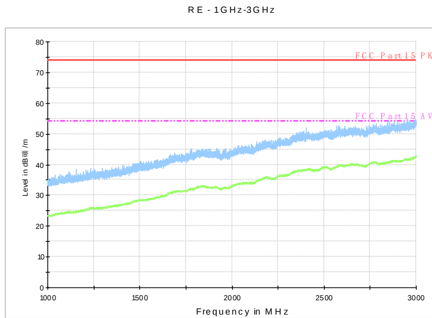
Fig. 45 Radiated Spurious Emission (802.11n-HT20, ch36, 1 GHz-3 GHz)
