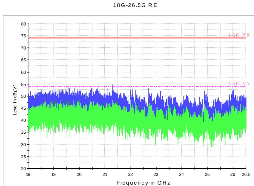
Fig. 66 Radiated Spurious Emission (802.11n-HT40, ch38, 18 GHz-26.5 GHz)
