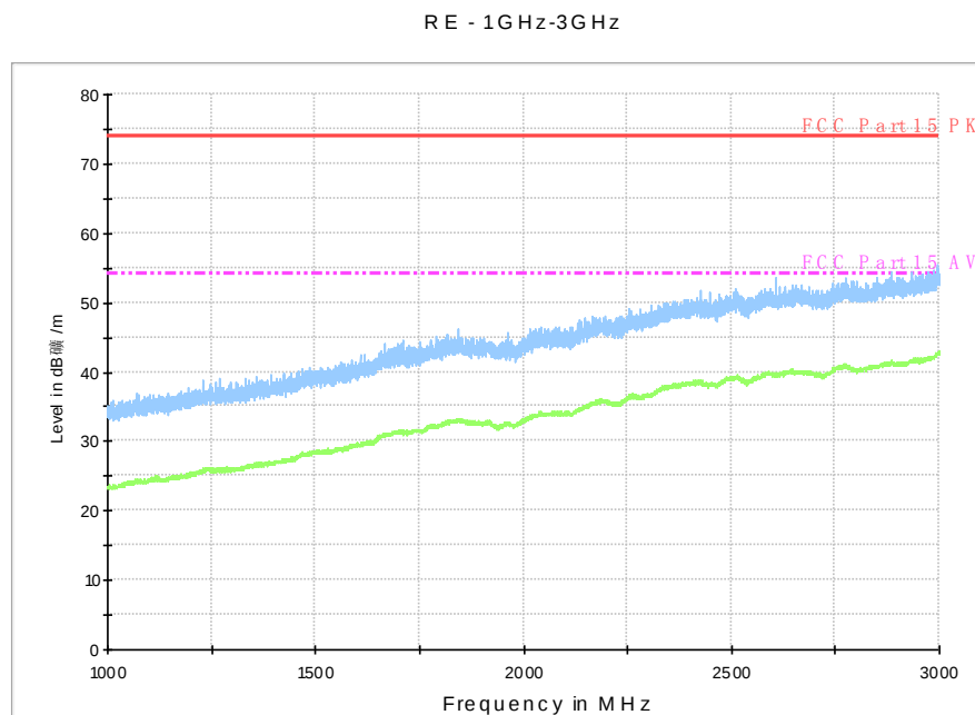
Fig. 27 Radiated Spurious Emission (802.11a, ch36, 1 GHz-3 GHz)
