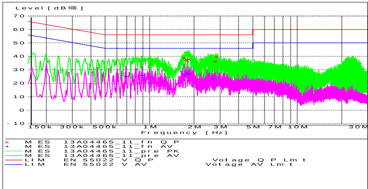
Fig. 74 Conducted Spurious Emission(802.11a, TX)
