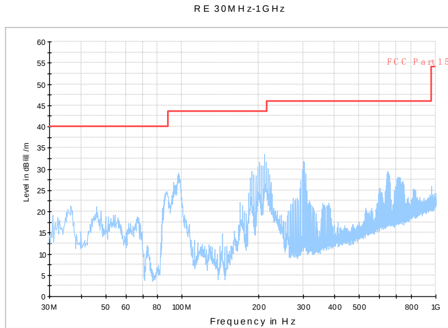
Fig. 38 Radiated Spurious Emission (802.11a, ch48, 30 MHz-1 GHz)
