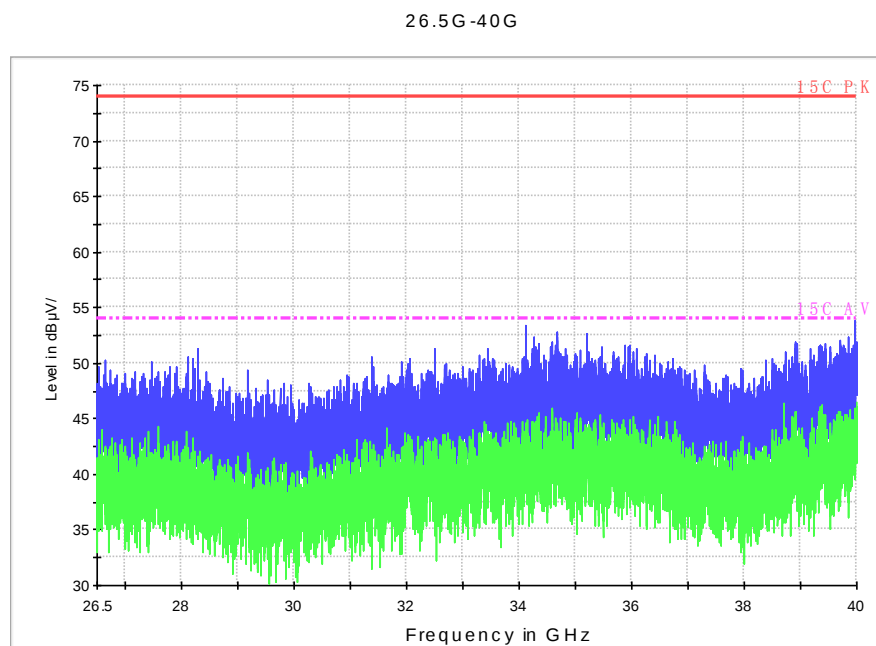
Fig. 43 Radiated Spurious Emission (802.11a, ch48, 26.5 GHz-40 GHz)
