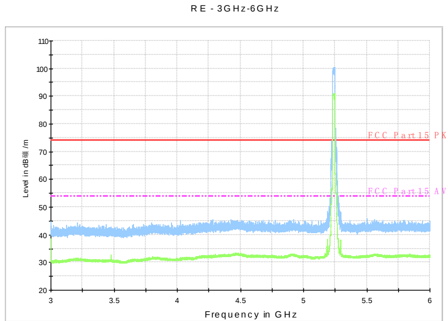
Fig. 58 Radiated Spurious Emission (802.11n-HT20, ch48, 3 GHz-6 GHz)
