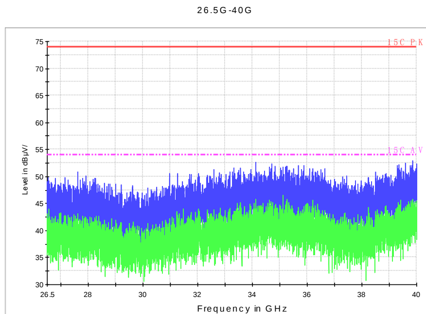
Fig. 37 Radiated Spurious Emission (802.11a, ch40, 26.5 GHz-40 GHz)
