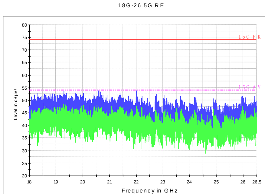
Fig. 42 Radiated Spurious Emission (802.11a, ch48, 18 GHz-26.5 GHz)
