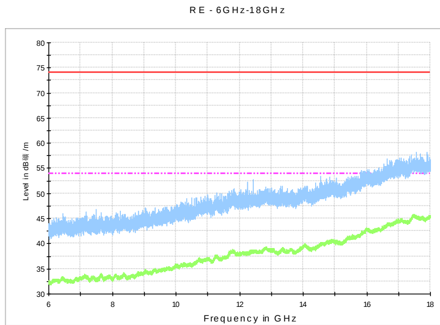
Fig. 71 Radiated Spurious Emission (802.11n-HT40, ch46, 6 GHz-18 GHz)
