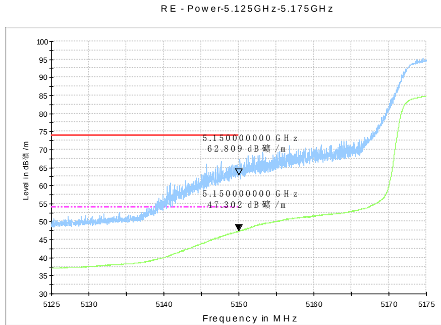
Fig. 25 Band Edges (802.11n-HT40, 5190MHz)
