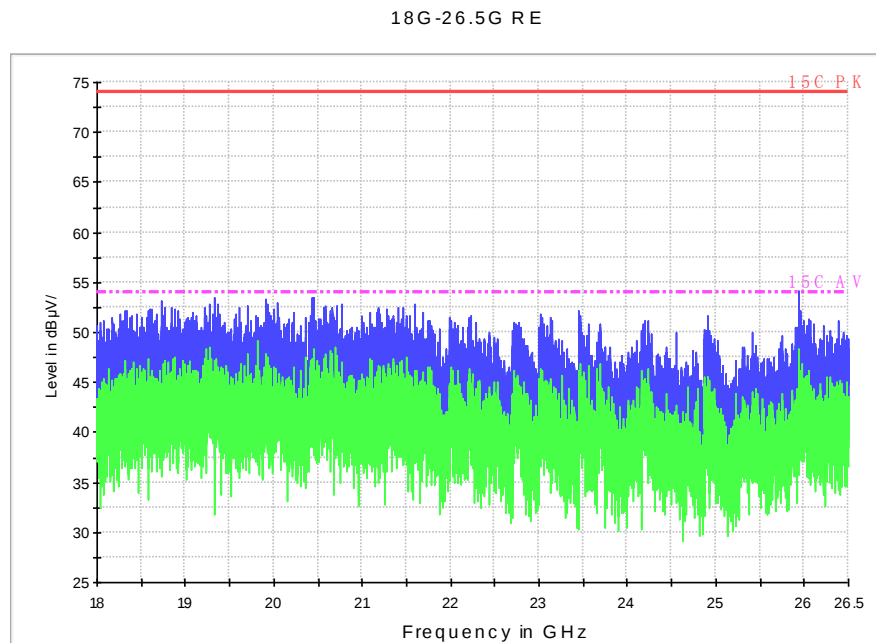
Fig. 60 Radiated Spurious Emission (802.11n-HT20, ch48, 18 GHz-26.5 GHz)
