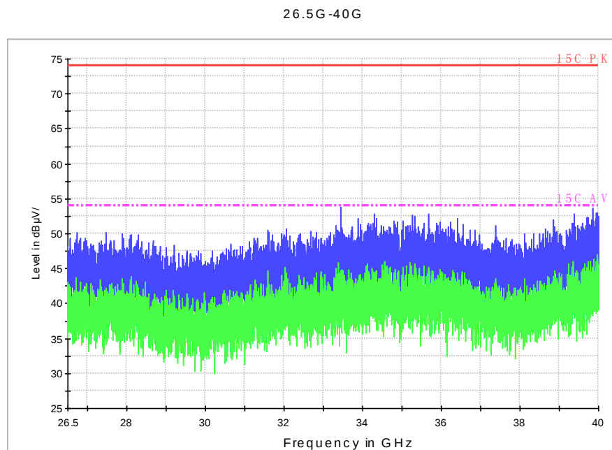
Fig. 73 Radiated Spurious Emission (802.11n-HT40, ch46, 26.5 GHz-40 GHz)
