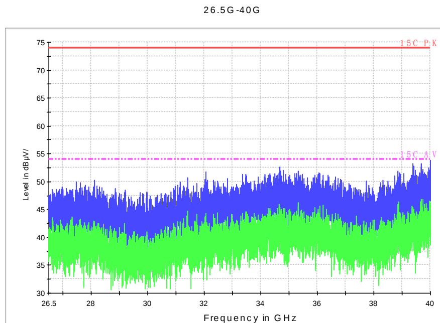
Fig. 67 Radiated Spurious Emission (802.11n-HT40, ch38, 26.5 GHz-40 GHz)
