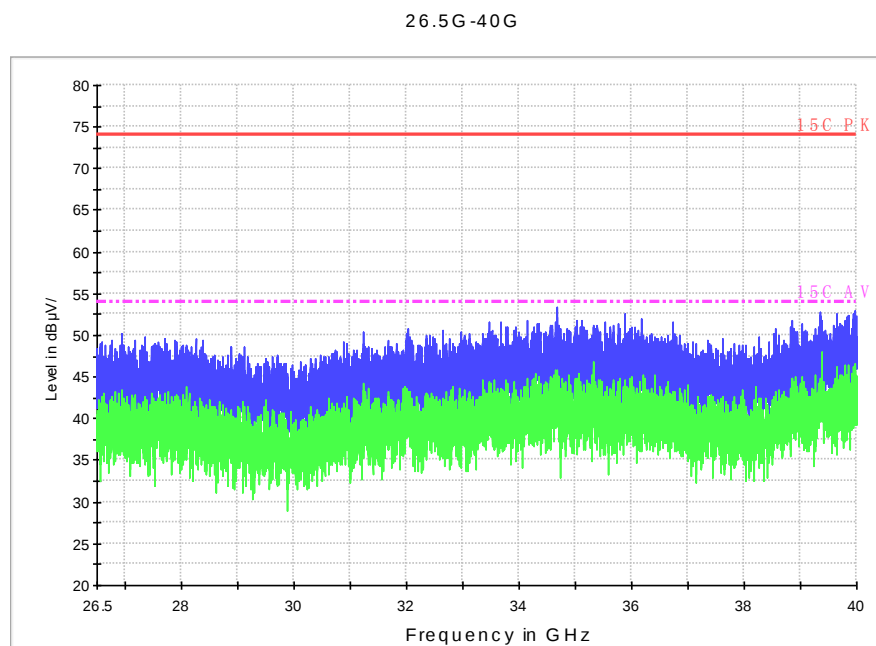
Fig. 55 Radiated Spurious Emission (802.11n-HT20, ch40, 26.5 GHz-40 GHz)
