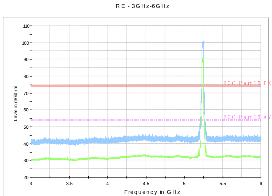
Fig. 40 Radiated Spurious Emission (802.11a, ch48, 3 GHz-6 GHz)
