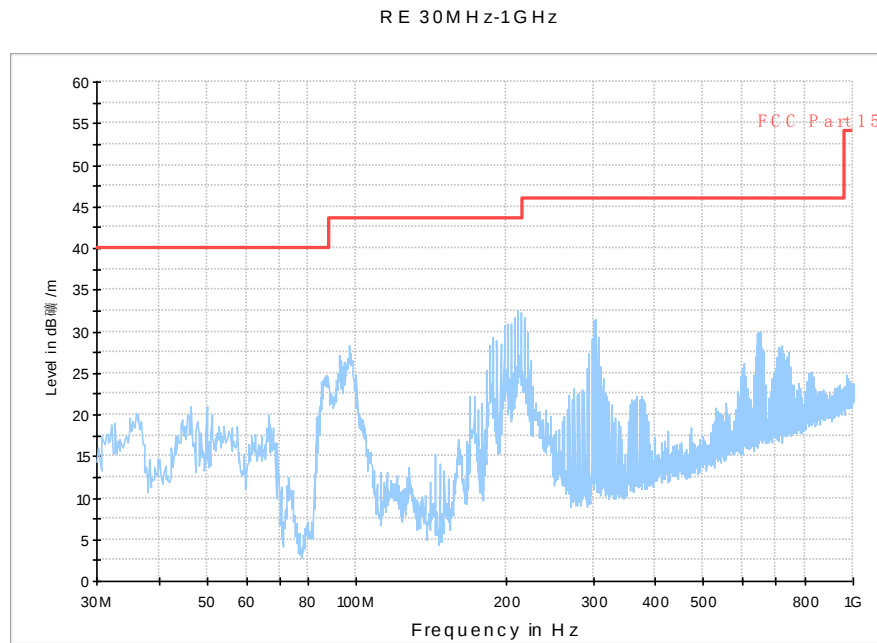
Fig. 32 Radiated Spurious Emission (802.11a, ch40, 30 MHz-1 GHz)
