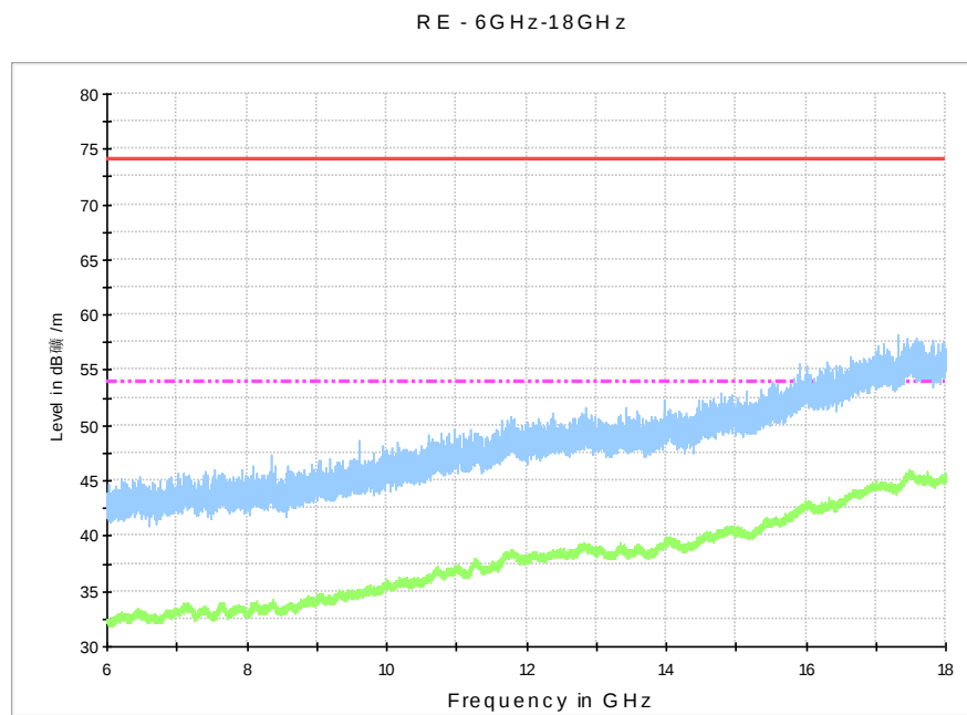
Fig. 65 Radiated Spurious Emission (802.11n-HT40, ch38, 6 GHz-18 GHz)
