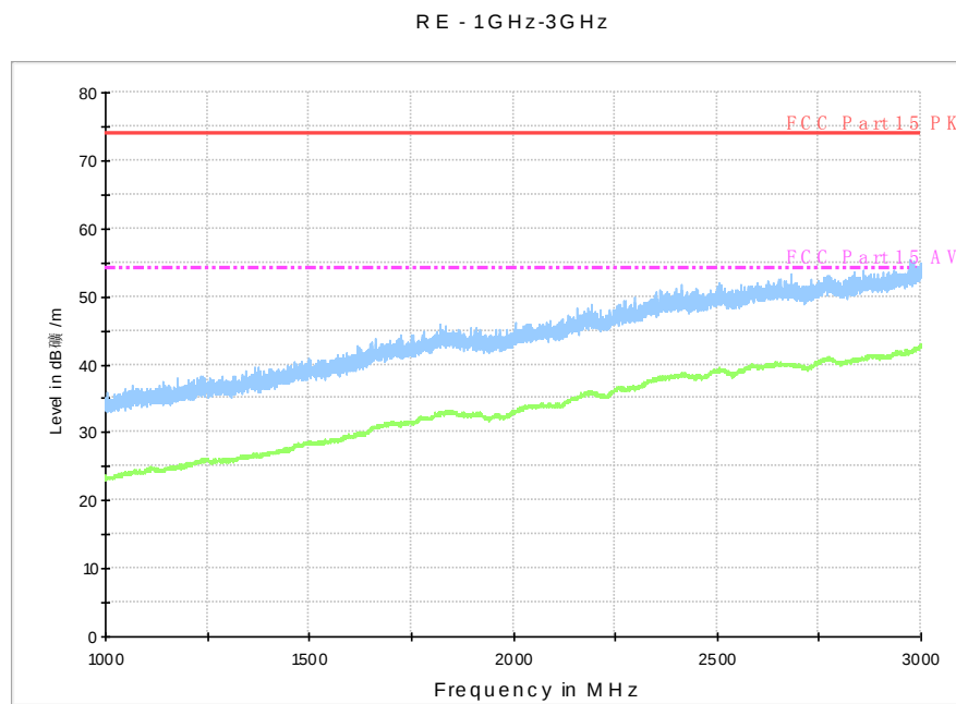
Fig. 63 Radiated Spurious Emission (802.11n-HT40, ch38, 1 GHz-3 GHz)
