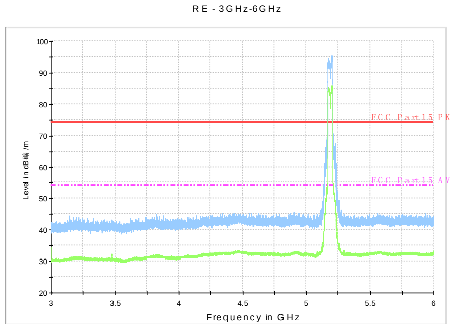
Fig. 64 Radiated Spurious Emission (802.11n-HT40, ch38, 3 GHz-6 GHz)
