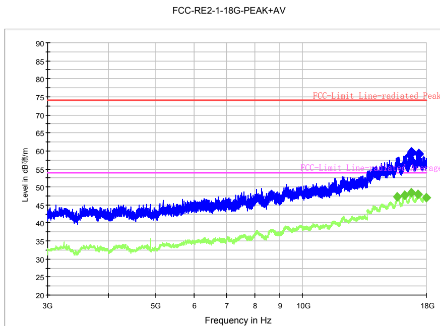
Fig. 68 Radiated Spurious Emission (8DPSK, Ch39, 3 GHz ~18 GHz)
