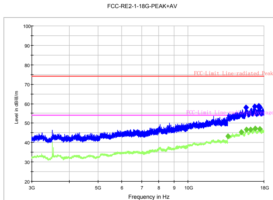
Fig. 71 Radiated Spurious Emission (8DPSK, Ch78, 3 GHz ~18 GHz)
