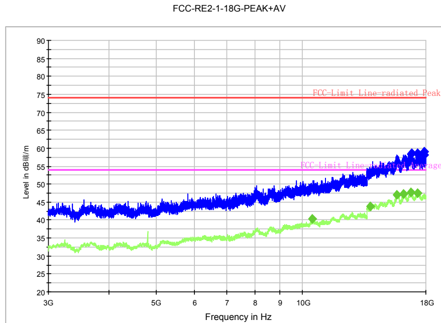
Fig. 65 Radiated Spurious Emission (8DPSK, Ch0, 3 GHz ~18 GHz)
