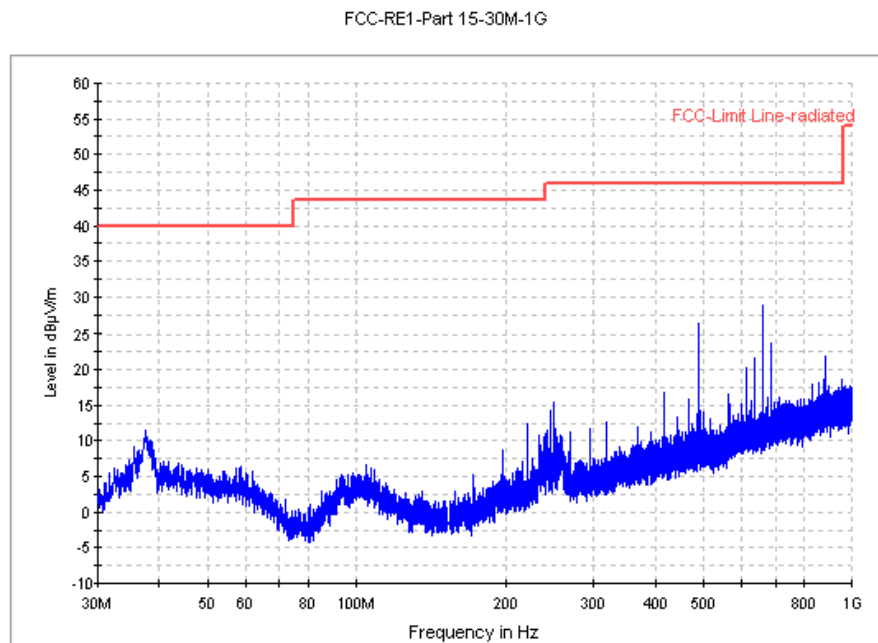
Fig. 66 Radiated Spurious Emission (8DPSK, Ch39, 30 MHz ~1 GHz)
