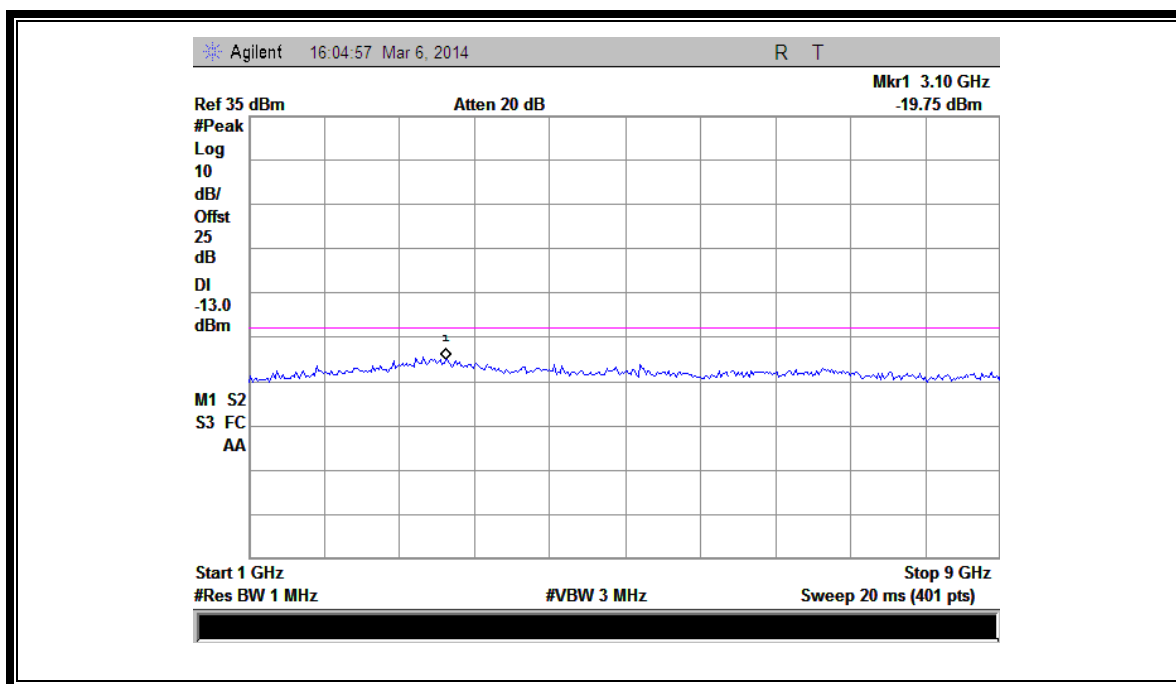
(Plot G1.1: HSDPA850MHz Channel = 4132, 1GHz to 9GHz)
