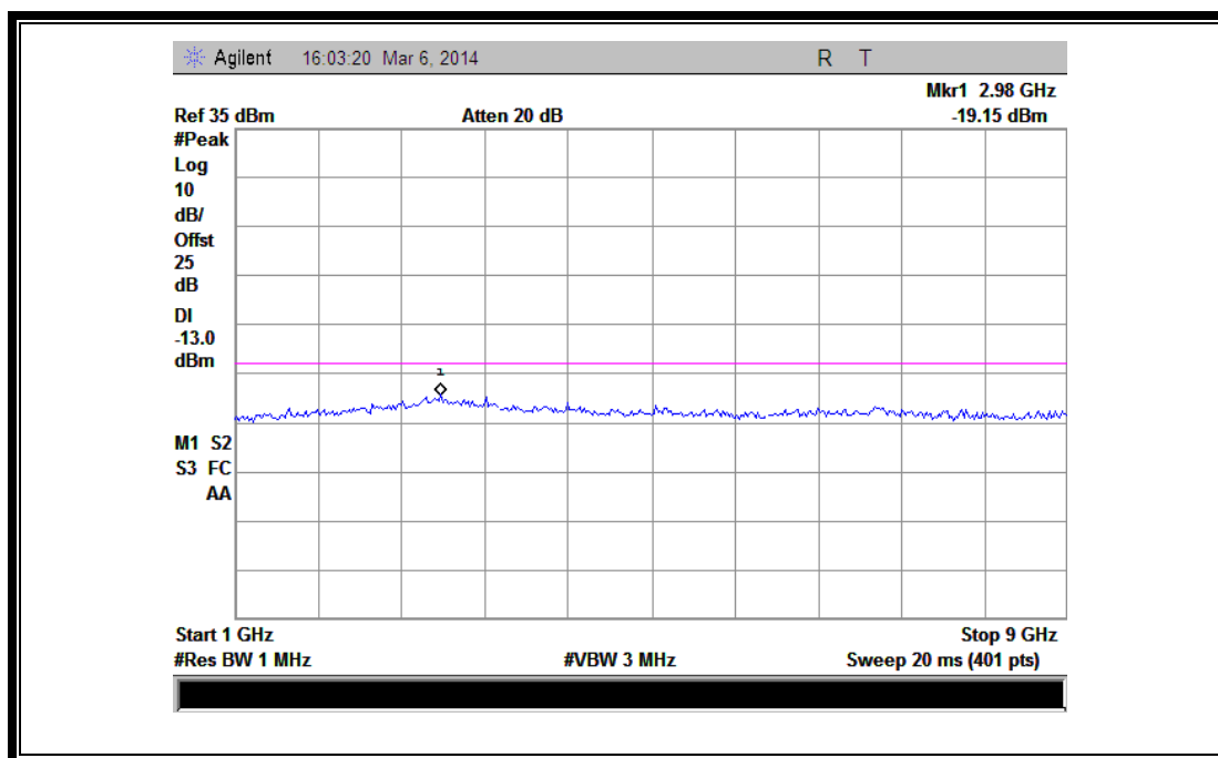
(Plot I2.1: HSUPA850MHz Channel = 4175, 1GHz to 9GHz)
