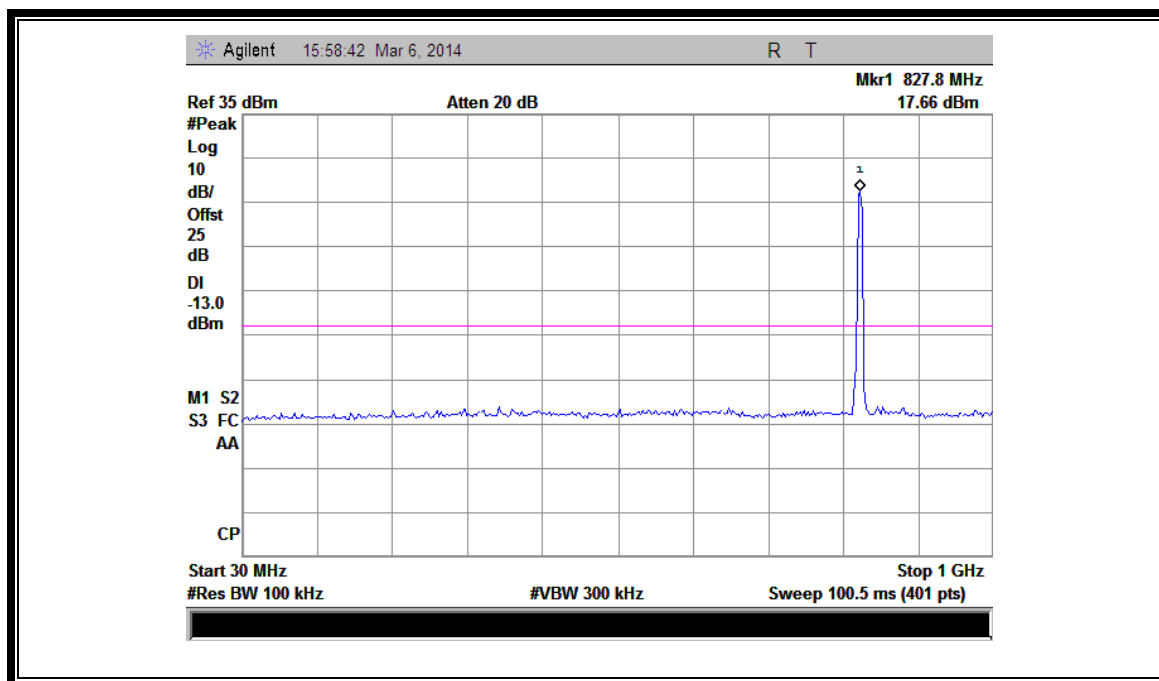
(Plot G1: HSDPA850MHz Channel = 4132, 30MHz to 1GHz)
