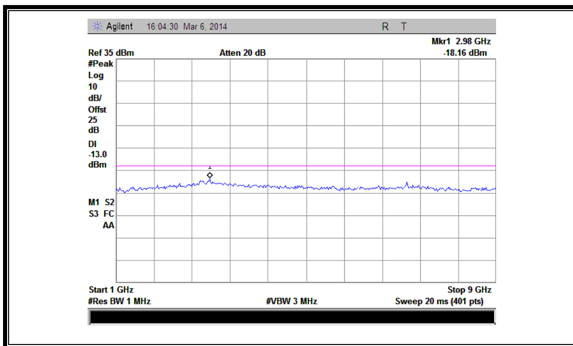
(Plot II.1: HSUPA850MHz Channel = 4132, 1GHz to 9GHz)
