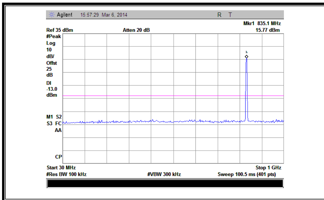
(Plot I 2: HSUPA850MHz Channel = 4175, 30MHz to 1GHz)
