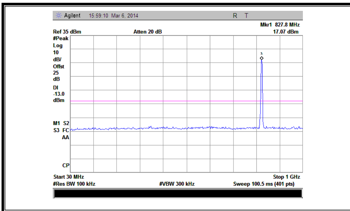
(Plot I 1: HSUPA850MHz Channel = 4132, 30MHz to 1GHz)
