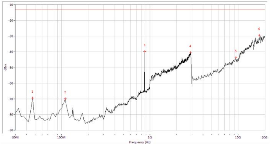
(Plot A.6: GSM 850MHz Channel = 251, Test Antenna Vertical)
