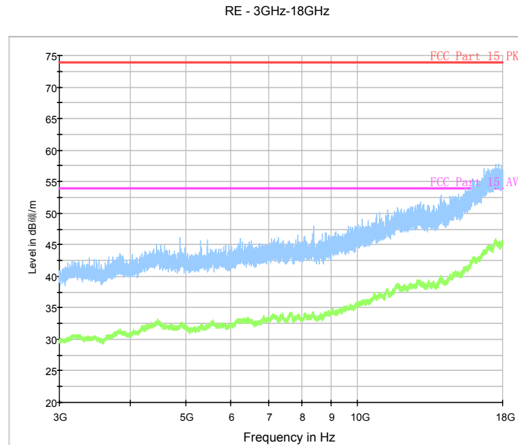
Fig.74. Radiated emission: \pi/4 DQPSK, Channel 0, 3 GHz - 18 GHz
