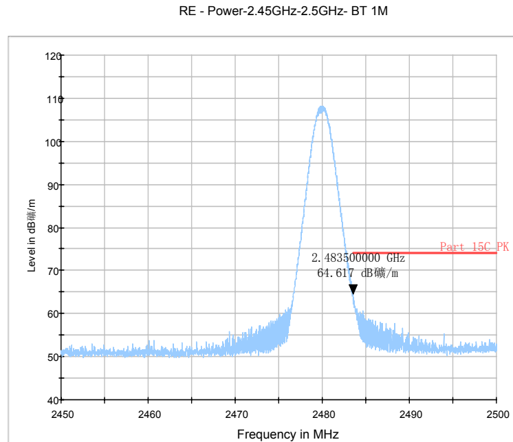
Fig.98. Radiated emission (Power): 8DPSK, high channel(VBW=1MHz)
