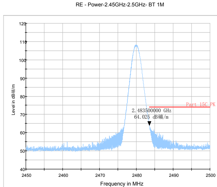
Fig.84. Radiated emission (Power): \pi/4 DQPSK, high channel(VBW=1MHz)
