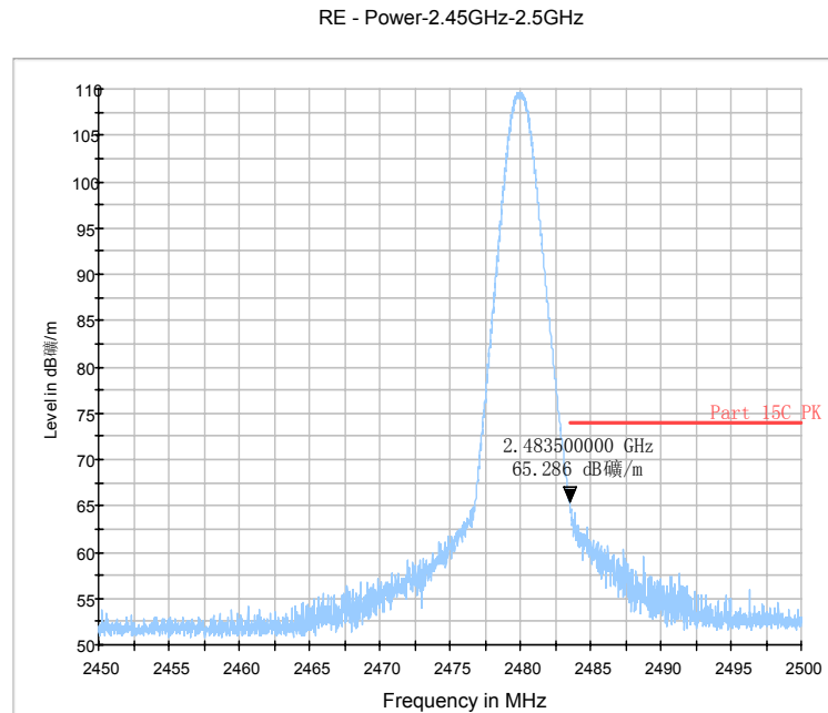
Fig.70. Radiated emission (Power) GFSK, high channel(VBW=1MHz)
