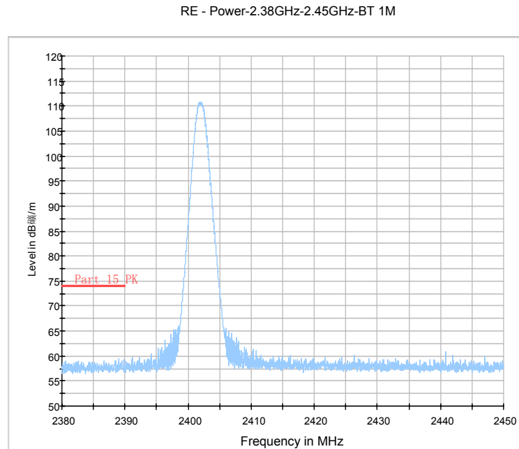
Fig.68. Radiated emission (Power): GFSK, low channel(VBW=1MHz)
