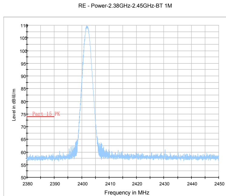
Fig.82. Radiated emission (Power): \pi/4 DQPSK, low channel(VBW=1MHz)
