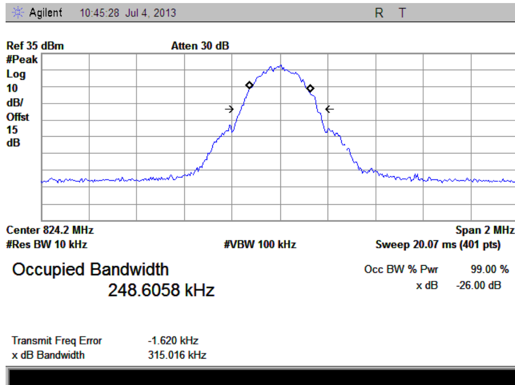
(Plot W1: GPRS 850MHz Channel = 128)
