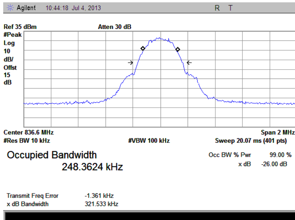
(Plot X1: GPRS 850MHz Channel = 190)
