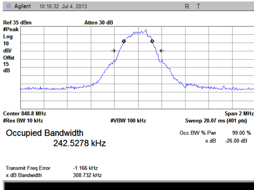
(Plot G1: GSM 850MHz Channel = 251)
