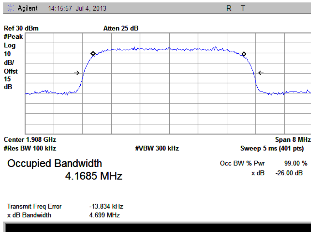
(Plot D1: HSPA+1900 MHz Channel = 9538)
