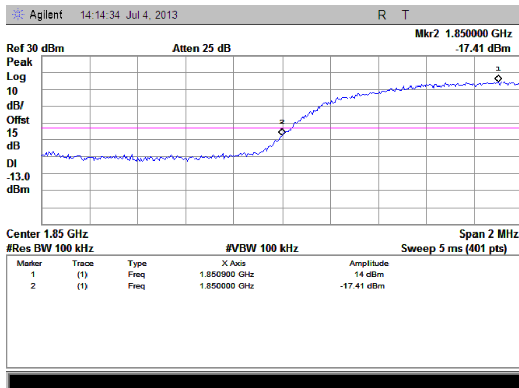
(Plot W: HSPA+ 1900 Channel = 9262)
