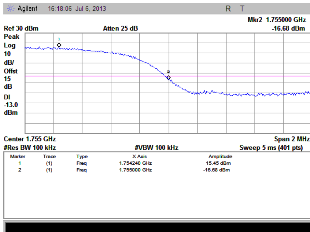
(Plot B1: HSDPA 1700 Channel = 1513)
