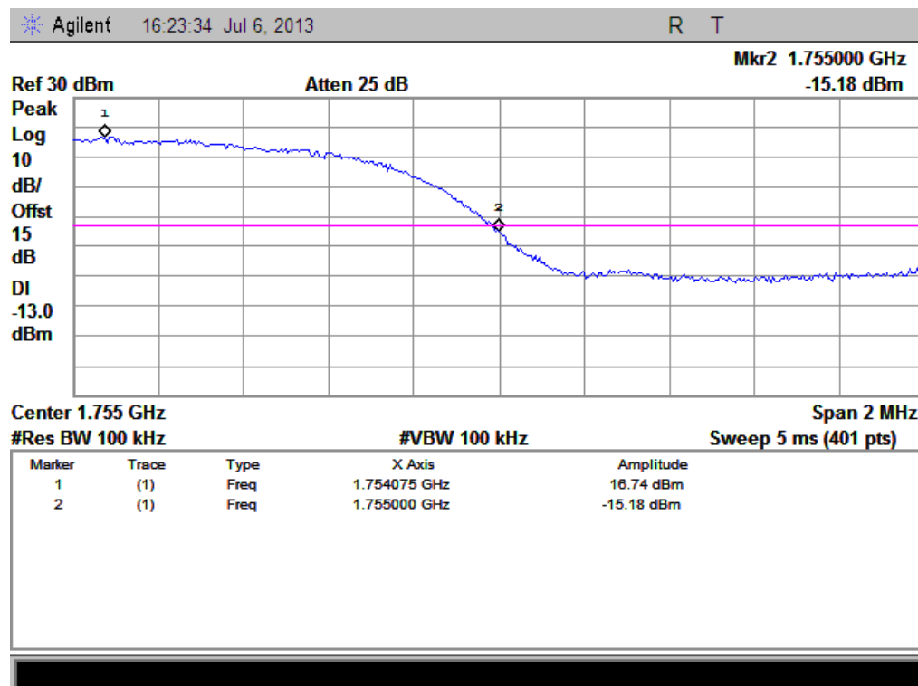
(Plot D1: HSUPA1700 Channel = 1513)
