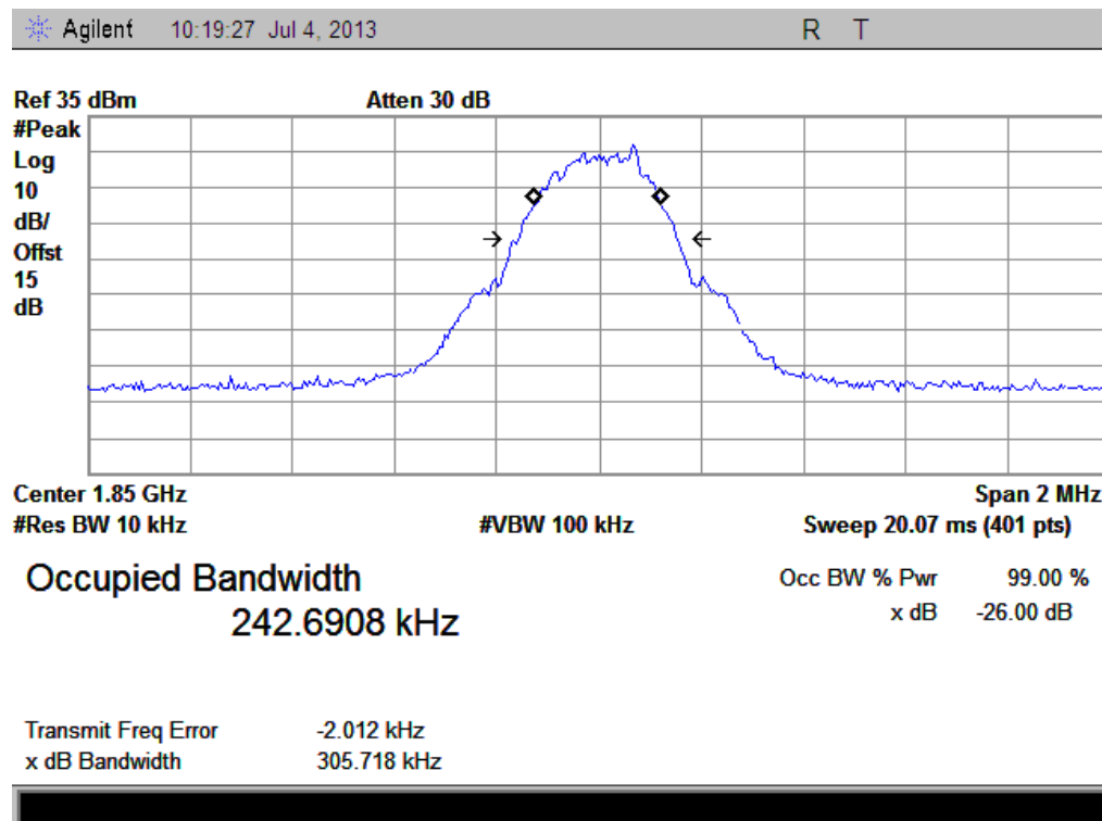
(Plot H1: GSM 1900MHz Channel = 512)
