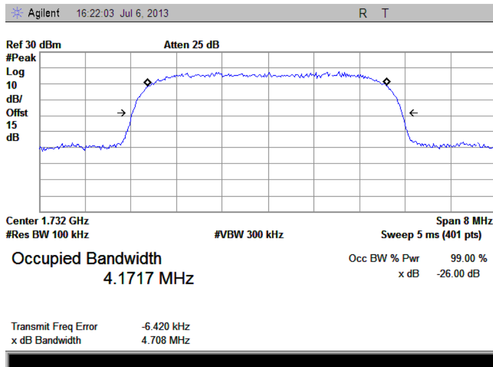
(Plot R1: HSUPA1700 MHz Channel = 1412)
