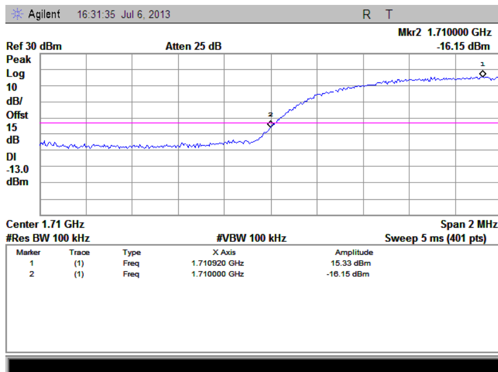
(Plot E1: HSPA+ 1700 Channel = 1312)
