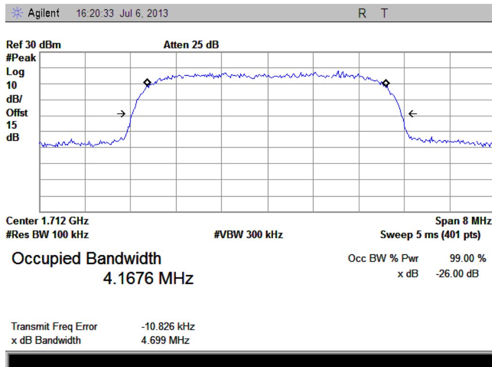
(Plot N1: HSDPA 1700MHz Channel = 1312)
