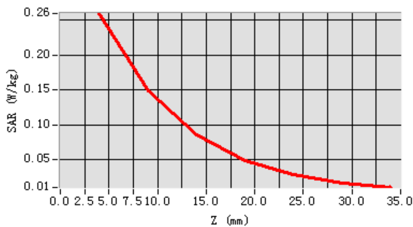
SAR, Z Axis Scan (X = 9, Y = -27)
