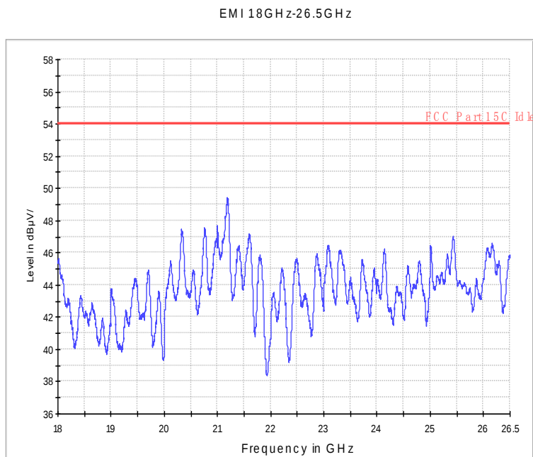
Fig.94. Radiated emission: 8DPSK, 18 GHz - 26 GHz
