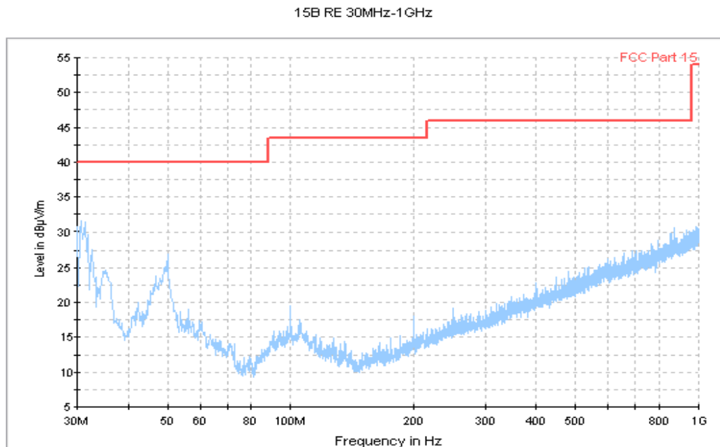
Figure A.7 Radiated Emission from 30MHz to 1GHz (Set.3, Charging mode)
