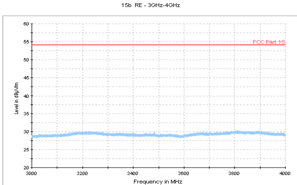
Figure A.9 Radiated Emission from 3GHz to 4GHz (Set.3, Charging mode)
