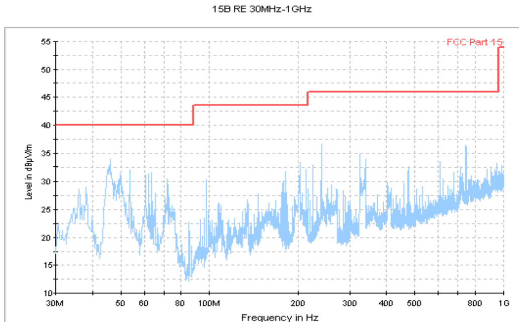
Figure A.1 Radiated Emission from 30MHz to 1GHz (Set.1, USB mode)
