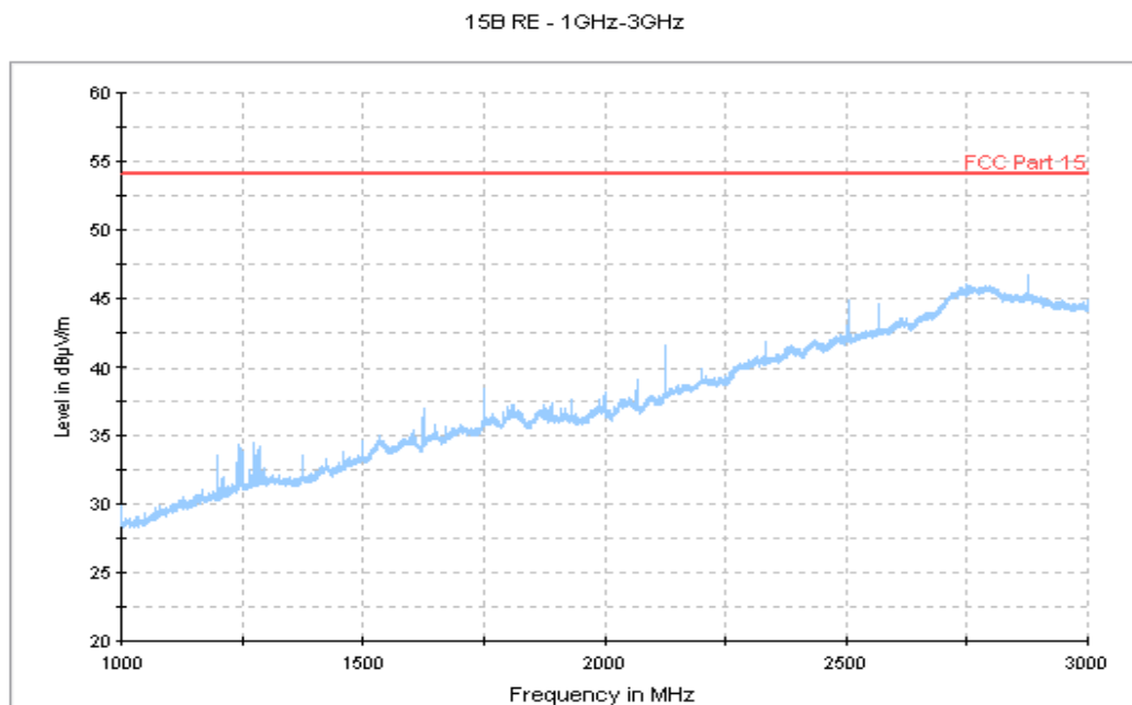
Figure A.8 Radiated Emission from 1GHz to 3GHz (Set.3, Charging mode)
