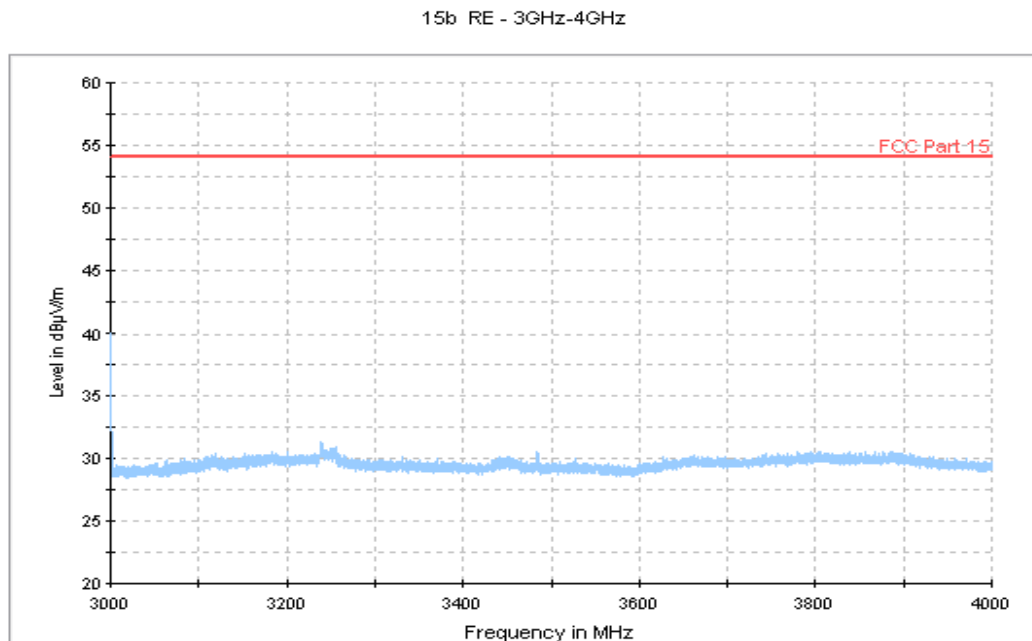
Figure A.3 Radiated Emission from 3GHz to 4GHz (Set.1, USB mode)
