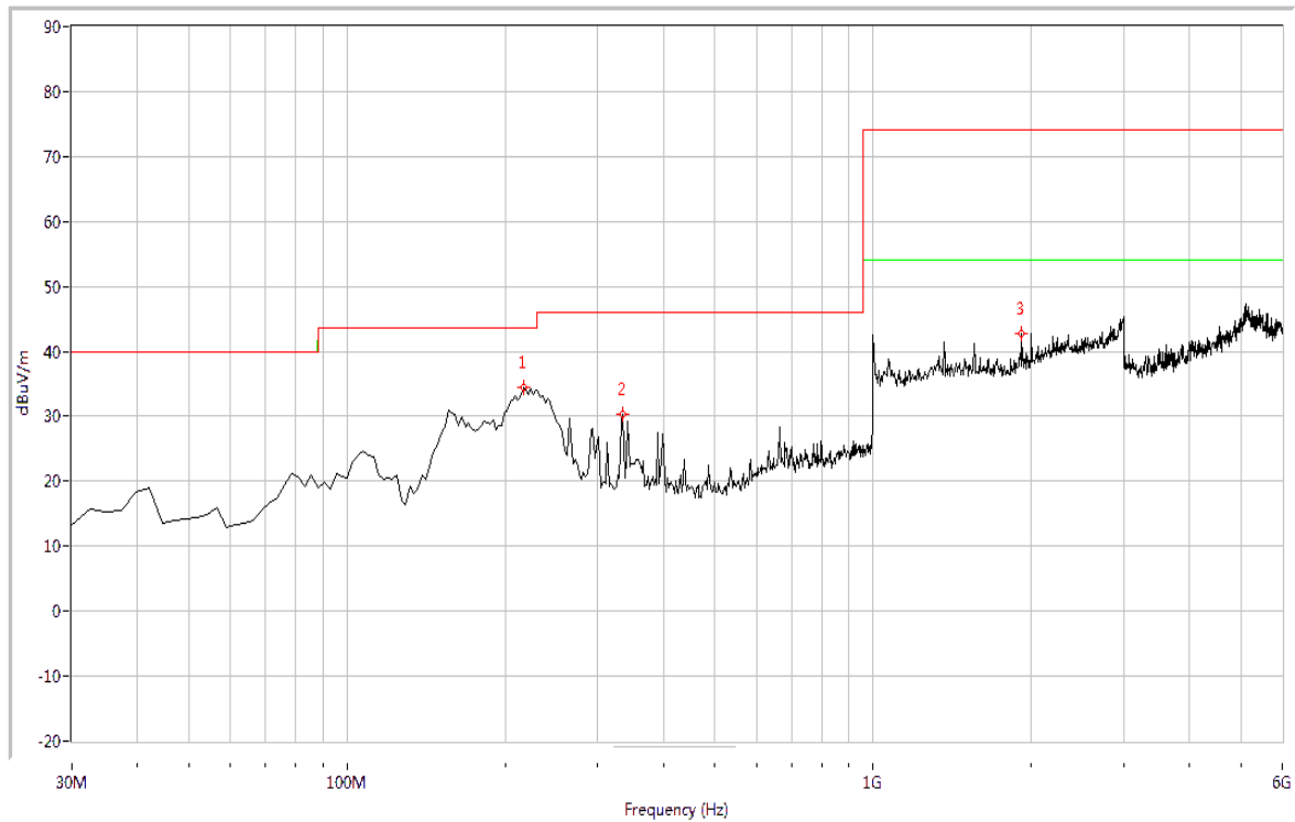
(Plot C: 30MHz – 6GHz, Test Antenna Horizontal)
