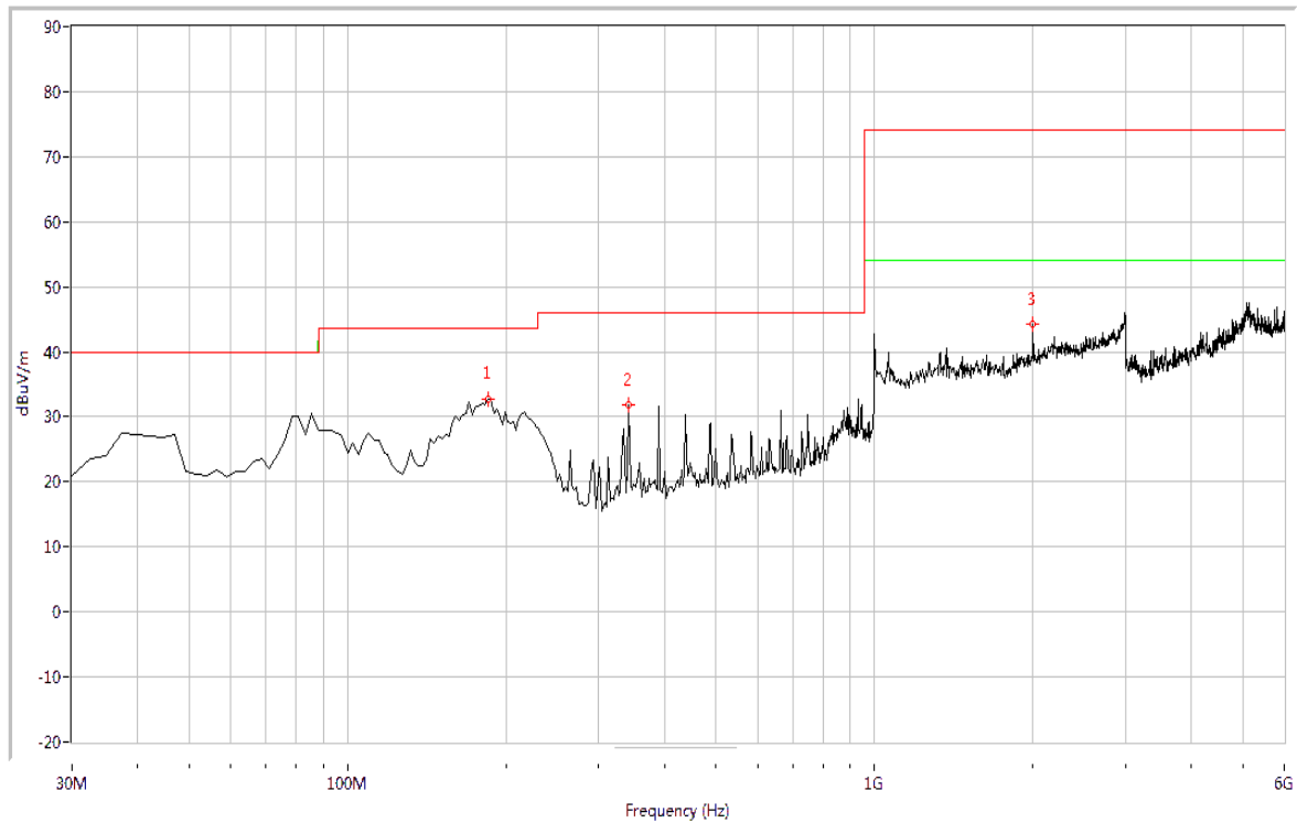
(Plot B: 30MHz – 6GHz, Test Antenna Vertical)
