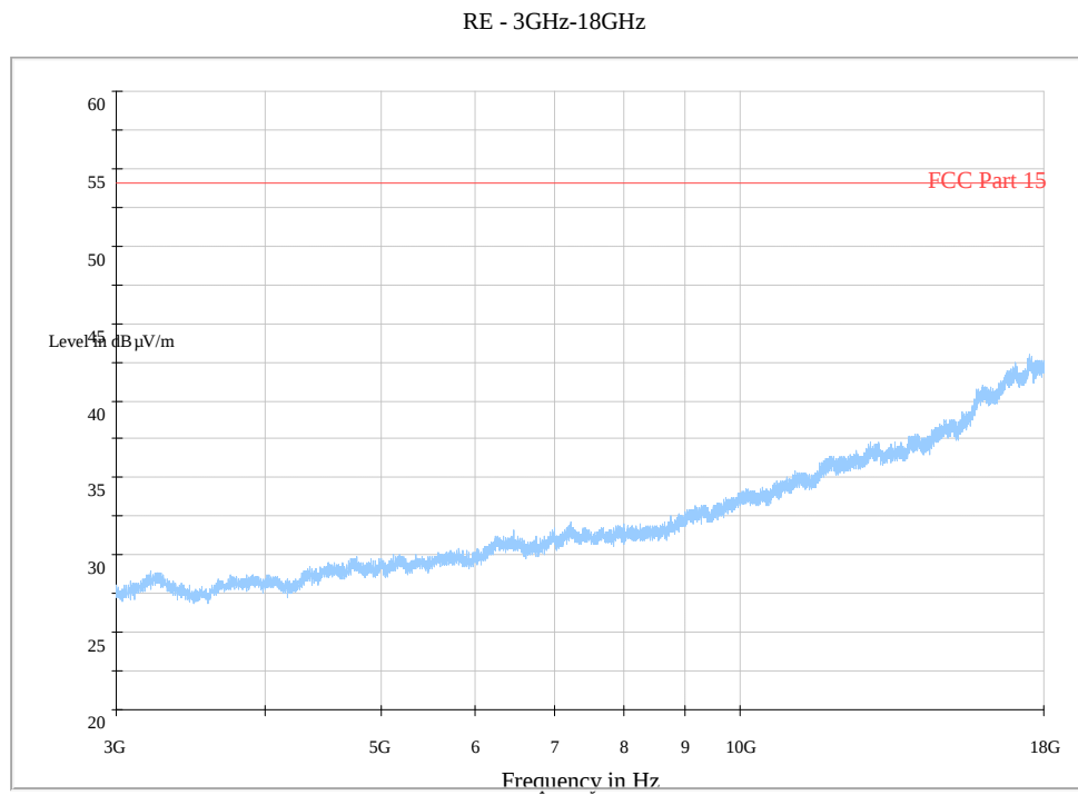
Fig. 154 Radiated Spurious Emission (802.11n-20MHz, Ch1, 3 GHz-18 GHz)
