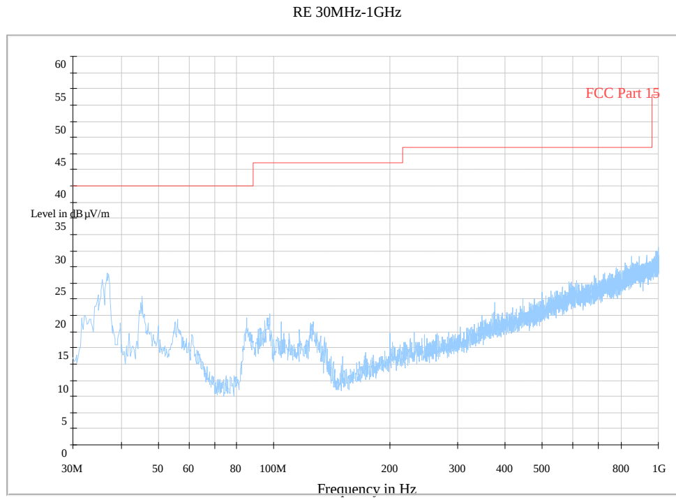
Fig. 159 Radiated Spurious Emission (802.11n-20MHz, Ch11, 30 MHz-1 GHz)
