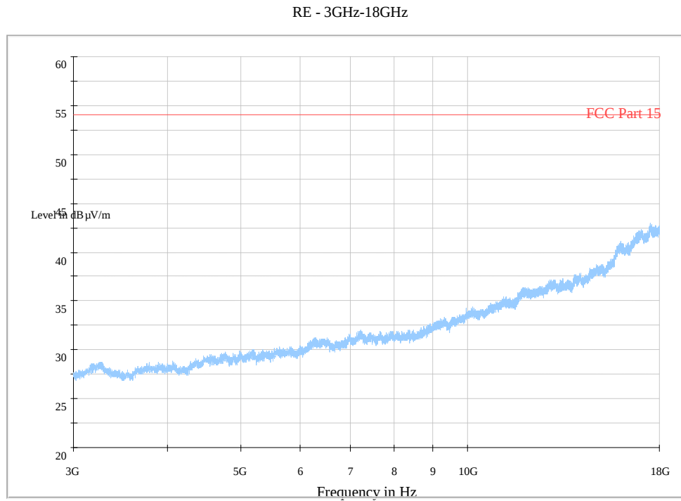
Fig. 161 Radiated Spurious Emission (802.11n-20MHz, Ch11, 3 GHz-18 GHz)
