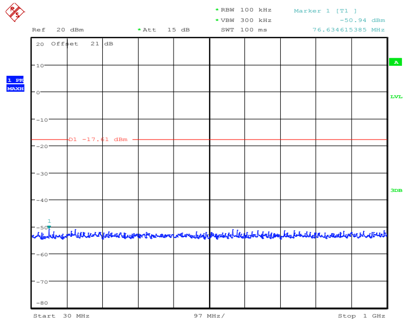
Fig. 121 Conducted Spurious Emission (802.11n-HT40, Ch9, Center Frequency)
