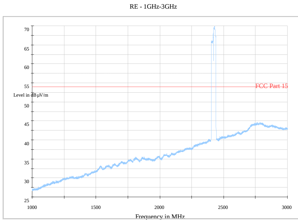
Fig. 164 Radiated Spurious Emission (802.11n-40MHz, Ch3, 1 GHz-3 GHz)
