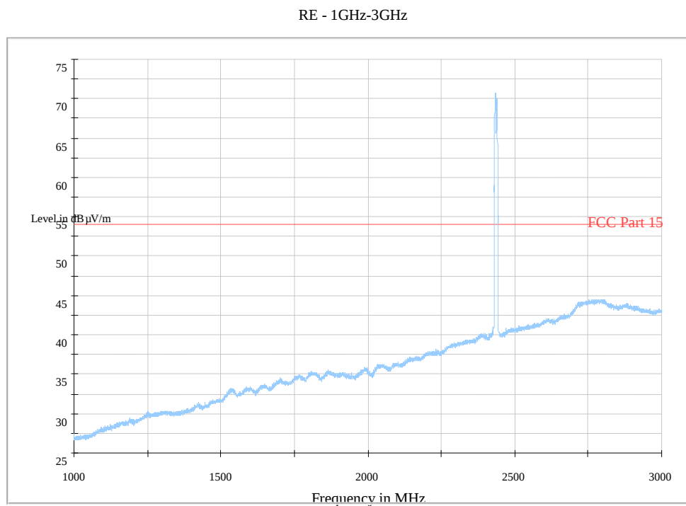
Fig. 134 Radiated Spurious Emission (802.11b, Ch6, 1 GHz-3 GHz)
