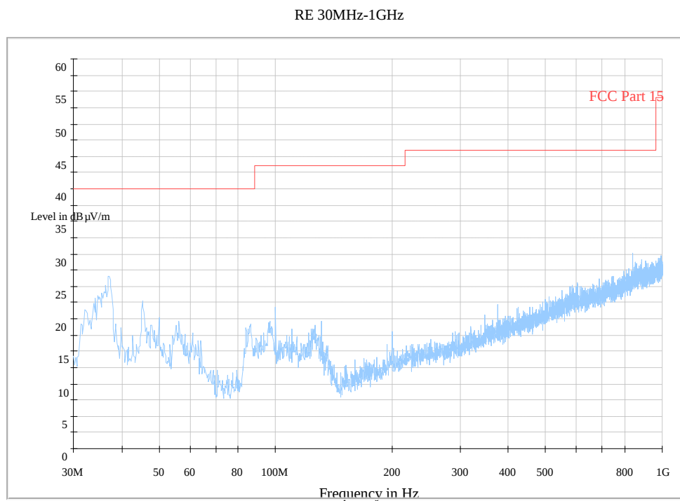
Fig. 152 Radiated Spurious Emission (802.11n-20MHz, Ch1, 30 MHz-1 GHz)
