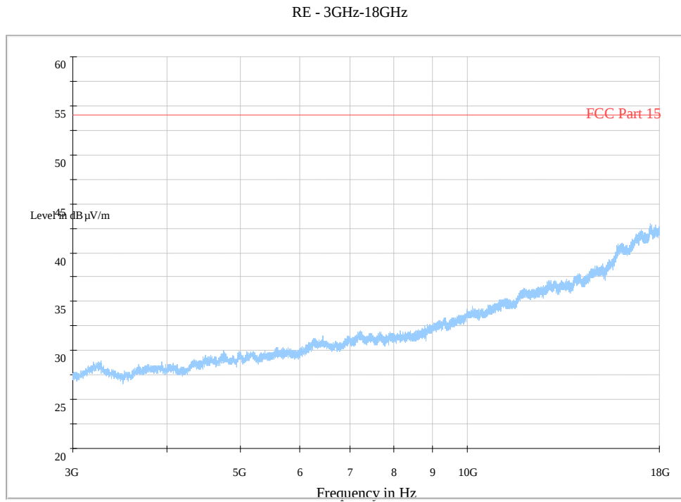
Fig. 139 Radiated Spurious Emission (802.11b, Ch11, 3 GHz-18 GHz)
