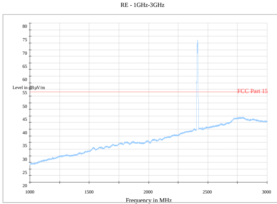
Fig. 131 Radiated Spurious Emission (802.11b, Ch1, 1 GHz-3 GHz)
