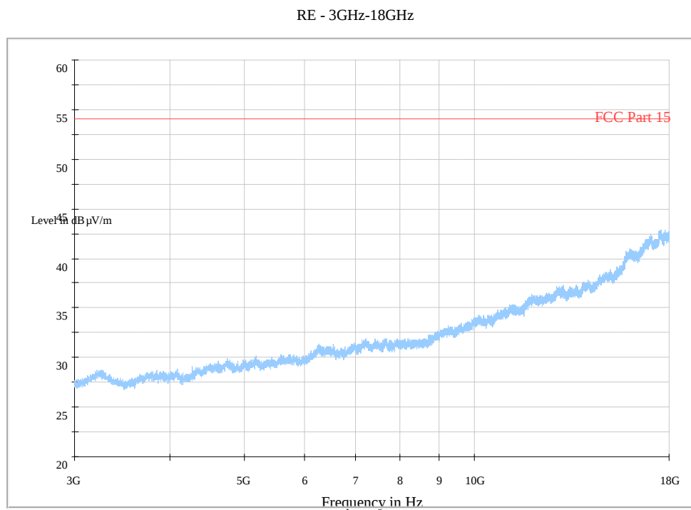
Fig. 172 Radiated Spurious Emission (802.11n-40MHz, Ch9, 3 GHz-18 GHz)
