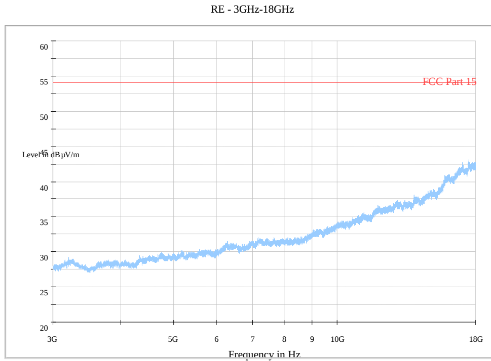
Fig. 132 Radiated Spurious Emission (802.11b, Ch1, 3 GHz-18 GHz)
