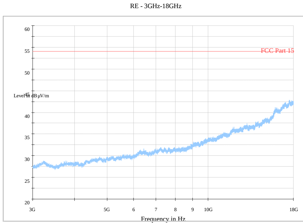
Fig. 150 Radiated Spurious Emission (802.11g, Ch11, 3 GHz-18 GHz)
