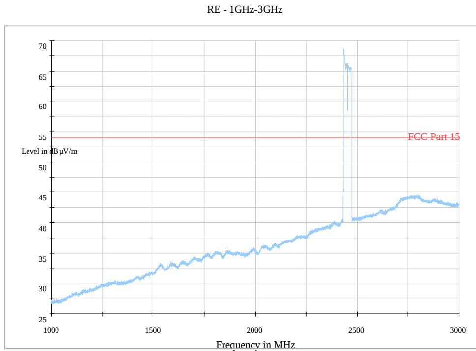
Fig. 171 Radiated Spurious Emission (802.11n-40MHz, Ch9, 1 GHz-3 GHz)
