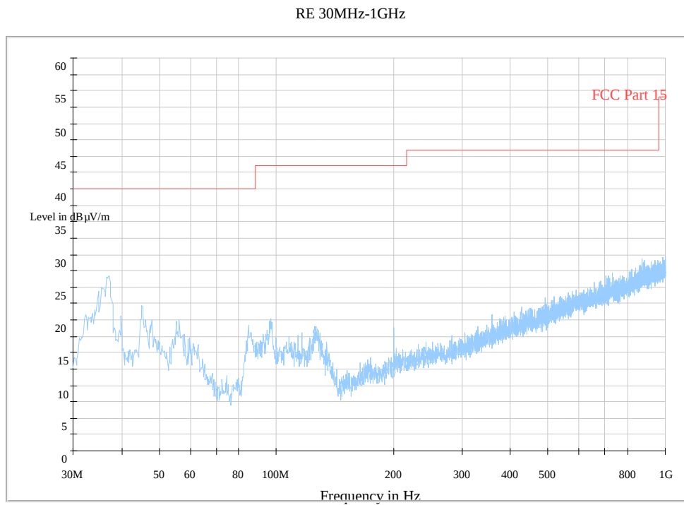
Fig. 166 Radiated Spurious Emission (802.11n-40MHz, Ch6, 30 MHz-1 GHz)
