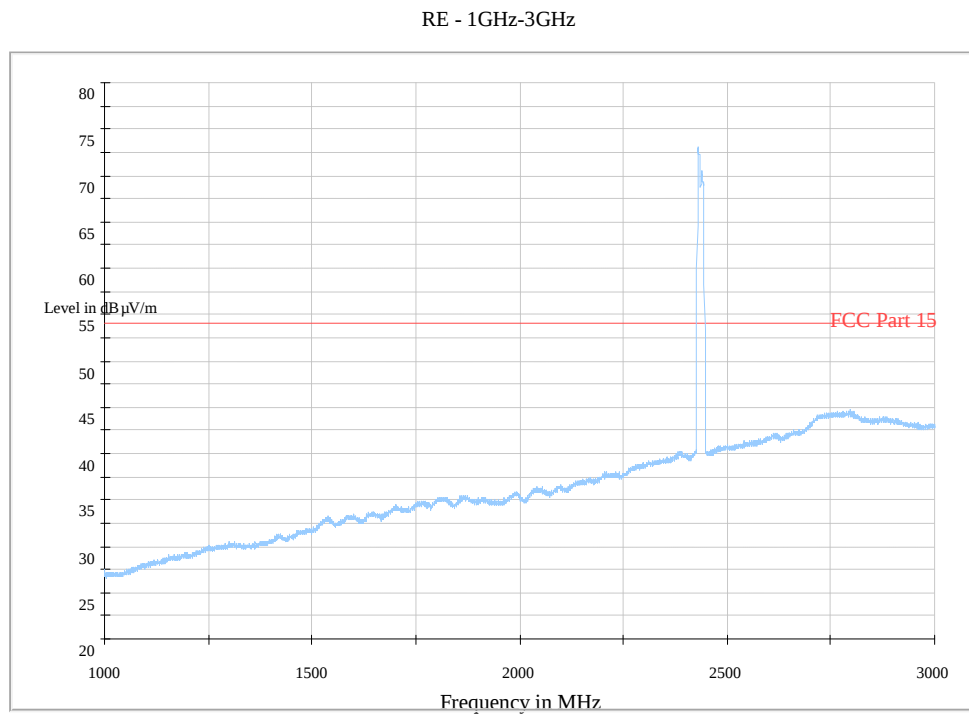
Fig. 145 Radiated Spurious Emission (802.11g, Ch6, 1 GHz-3 GHz)
