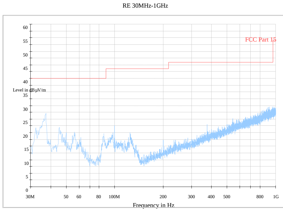
Fig. 163 Radiated Spurious Emission (802.11n-40MHz, Ch3, 30 MHz-1 GHz)
