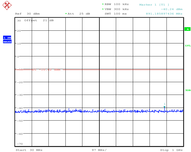
Fig. 49 Conducted Spurious Emission (802.11b, Ch11, Center Frequency)
