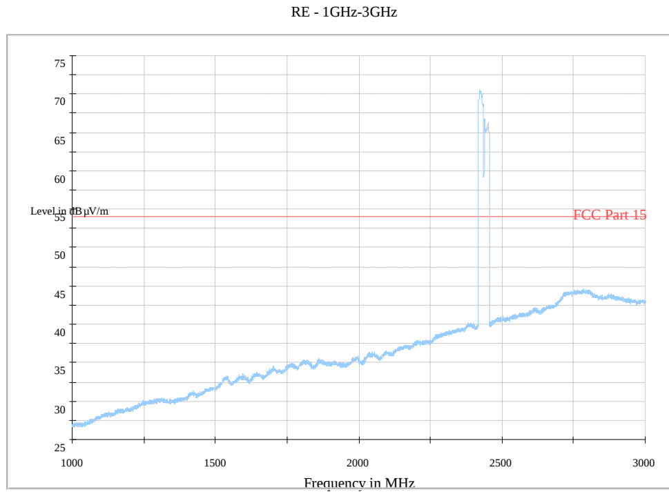
Fig. 167 Radiated Spurious Emission (802.11n-40MHz, Ch6, 1 GHz-3 GHz)
