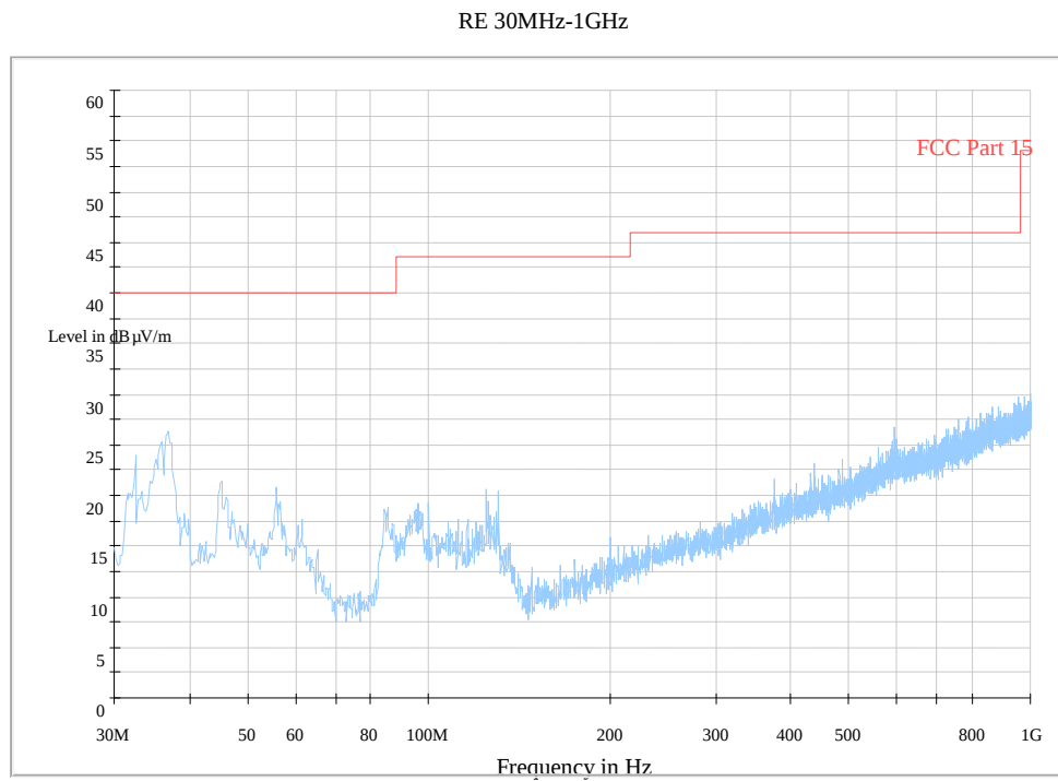
Fig. 137 Radiated Spurious Emission (802.11b, Ch11, 30 MHz-1 GHz)
