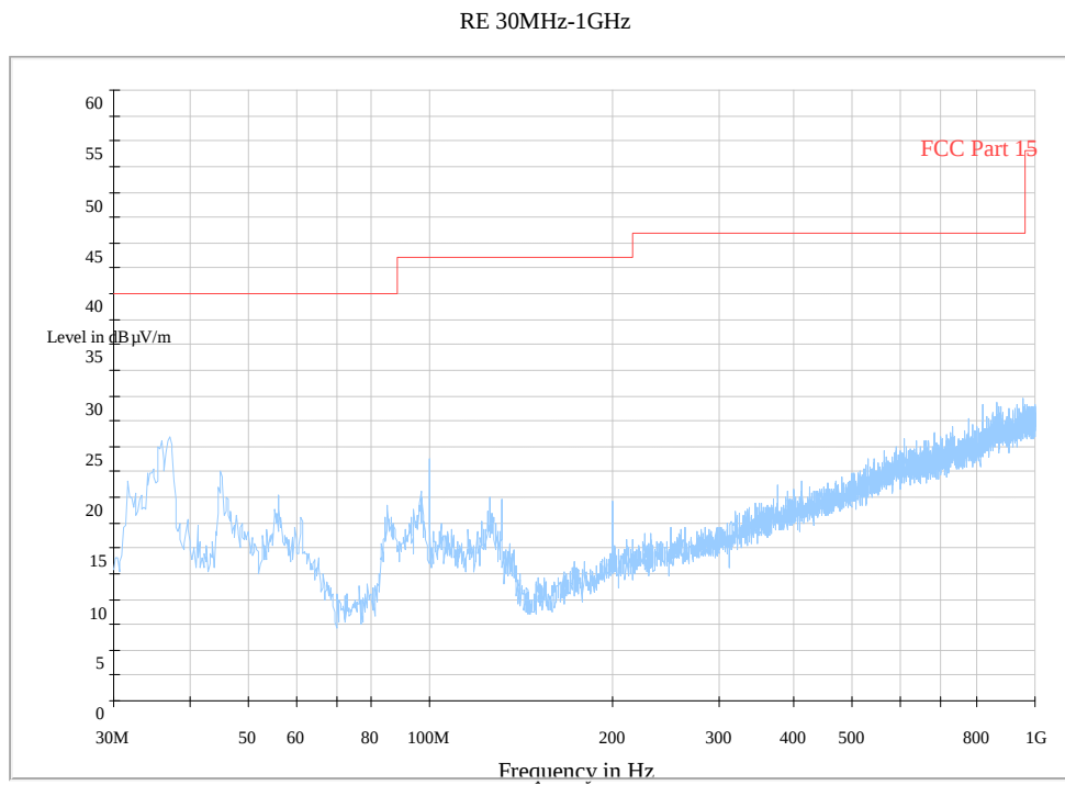
Fig. 144 Radiated Spurious Emission (802.11g, Ch6, 30 MHz-1 GHz)
