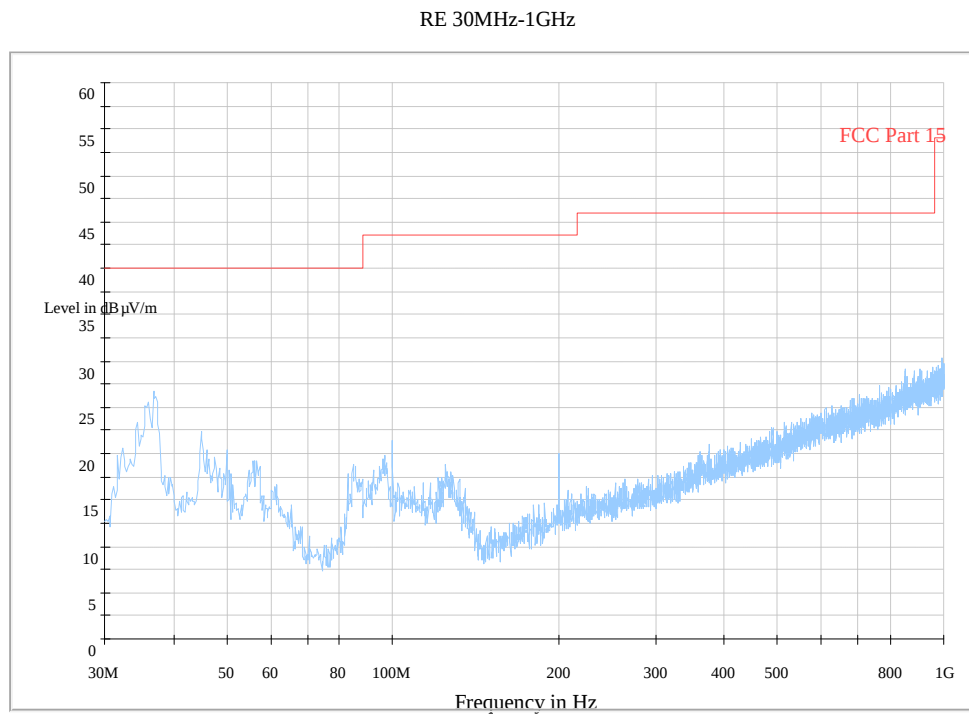
Fig. 133 Radiated Spurious Emission (802.11b, Ch6, 30 MHz-1 GHz)
