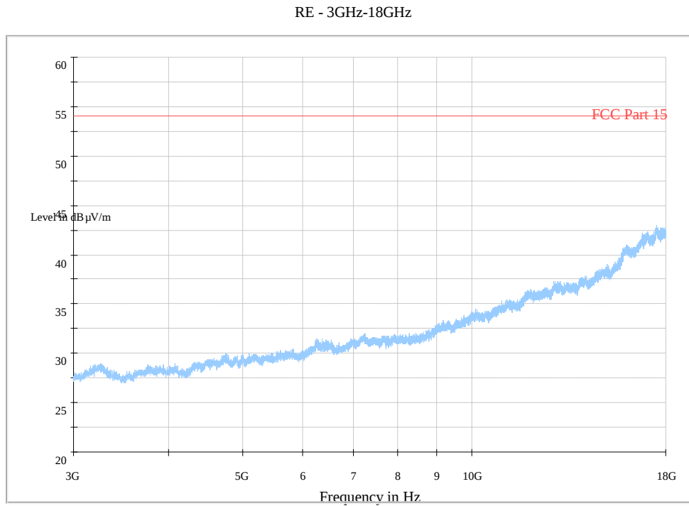
Fig. 143 Radiated Spurious Emission (802.11g, Ch1, 3 GHz-18 GHz)
