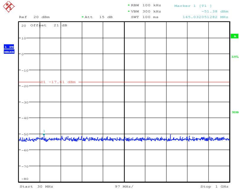
Fig. 113 Conducted Spurious Emission (802.11n-HT40, Ch6, Center Frequency)
