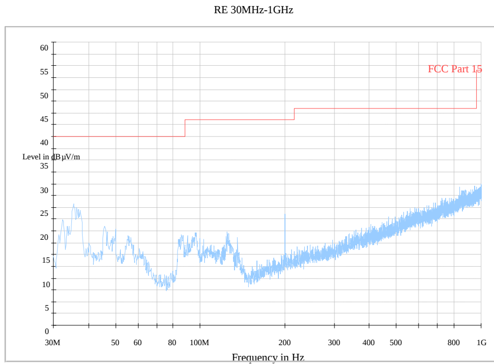
Fig. 141 Radiated Spurious Emission (802.11g, Ch1, 30 MHz-1 GHz)
