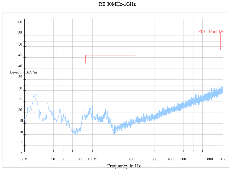
Fig. 155 Radiated Spurious Emission (802.11n-20MHz, Ch6, 30 MHz-1 GHz)
