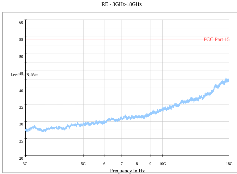
Fig. 135 Radiated Spurious Emission (802.11b, Ch6, 3 GHz-18 GHz)
