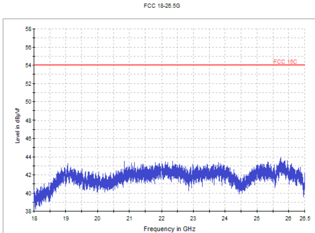
Fig. 173 Radiated Spurious Emission (All channels): 18GHz – 26.5GHz
