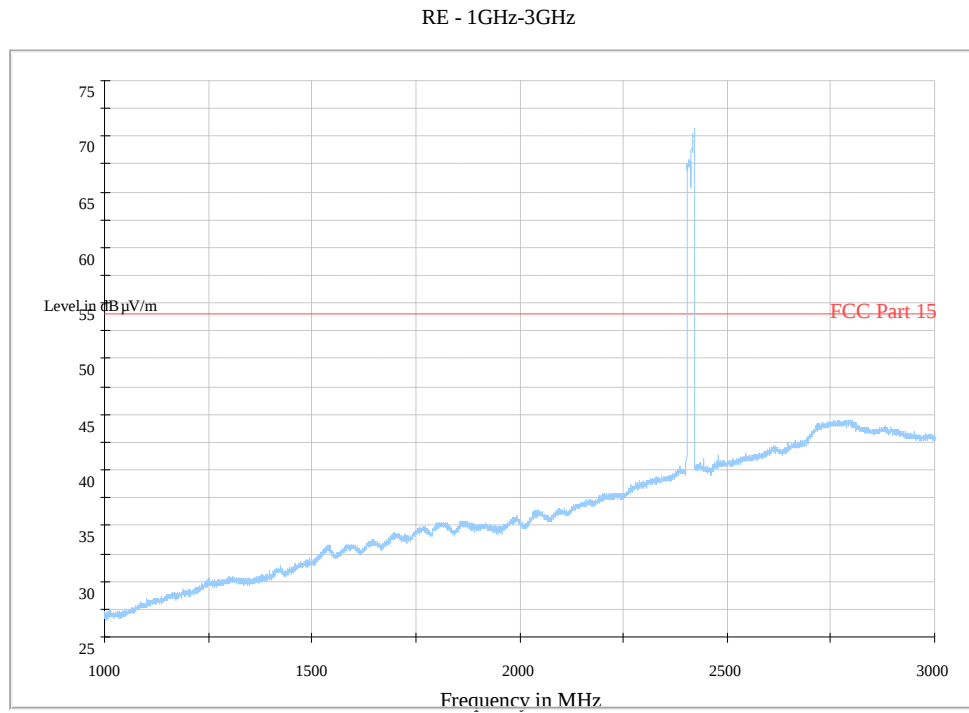
Fig. 153 Radiated Spurious Emission (802.11n-20MHz, Ch1, 1 GHz-3 GHz)
