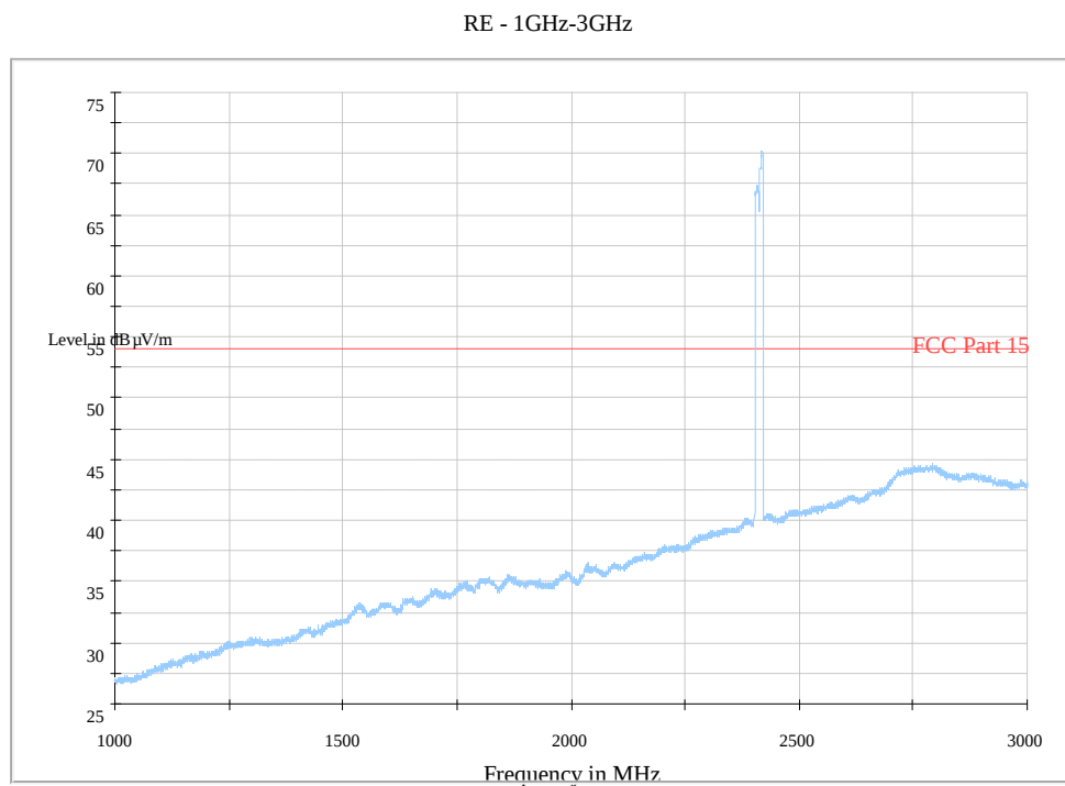
Fig. 142 Radiated Spurious Emission (802.11g, Ch1, 1 GHz-3 GHz)
