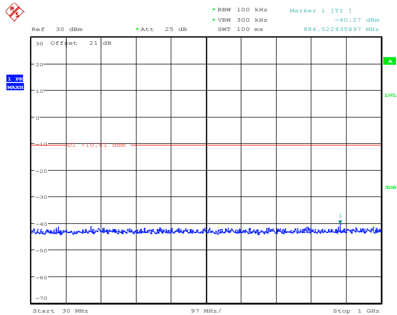
Fig. 41 Conducted Spurious Emission (802.11b, Ch6, Center Frequency)
