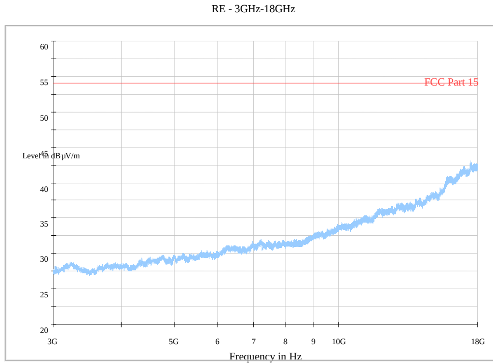
Fig. 157 Radiated Spurious Emission (802.11n-20MHz, Ch6, 3 GHz-18 GHz)
