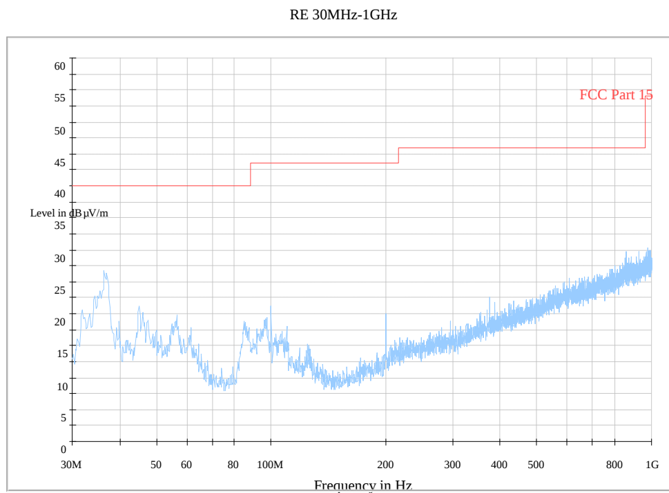
Fig. 148 Radiated Spurious Emission (802.11g, Ch11, 30 MHz-1 GHz)
