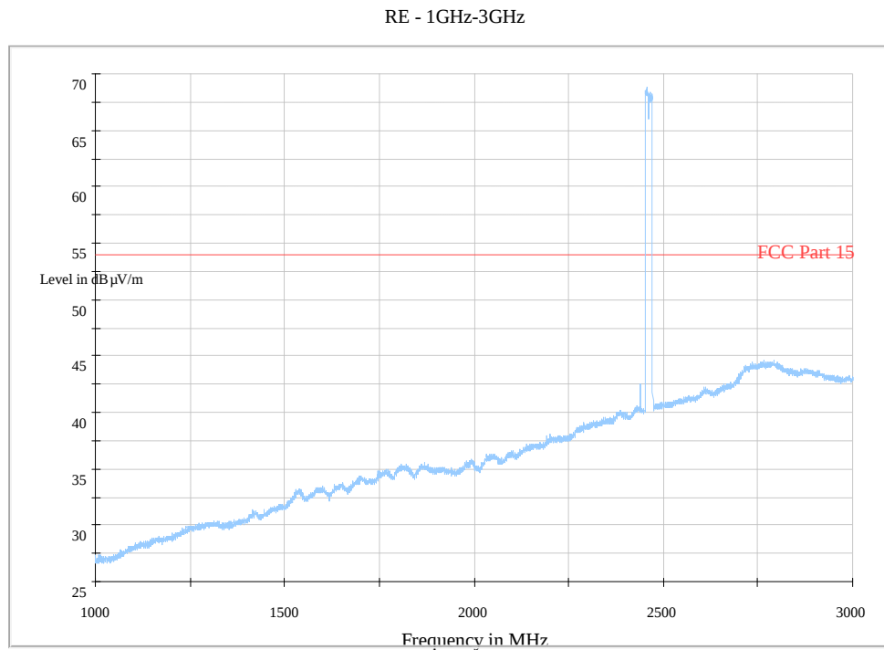
Fig. 160 Radiated Spurious Emission (802.11n-20MHz, Ch11, 1 GHz-3 GHz)
