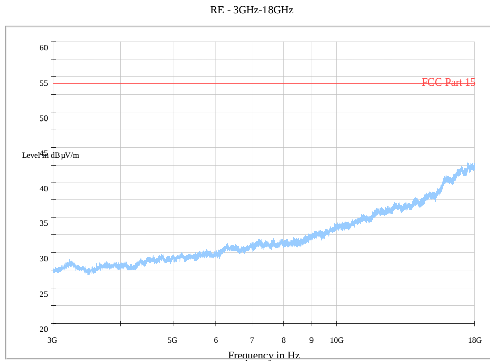
Fig. 168 Radiated Spurious Emission (802.11n-40MHz, Ch6, 3 GHz-18 GHz)
