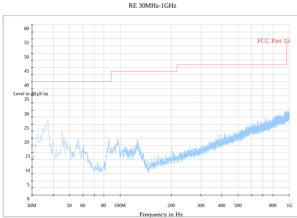
Fig. 130 Radiated Spurious Emission (802.11b, Ch1, 30 MHz-1 GHz)
