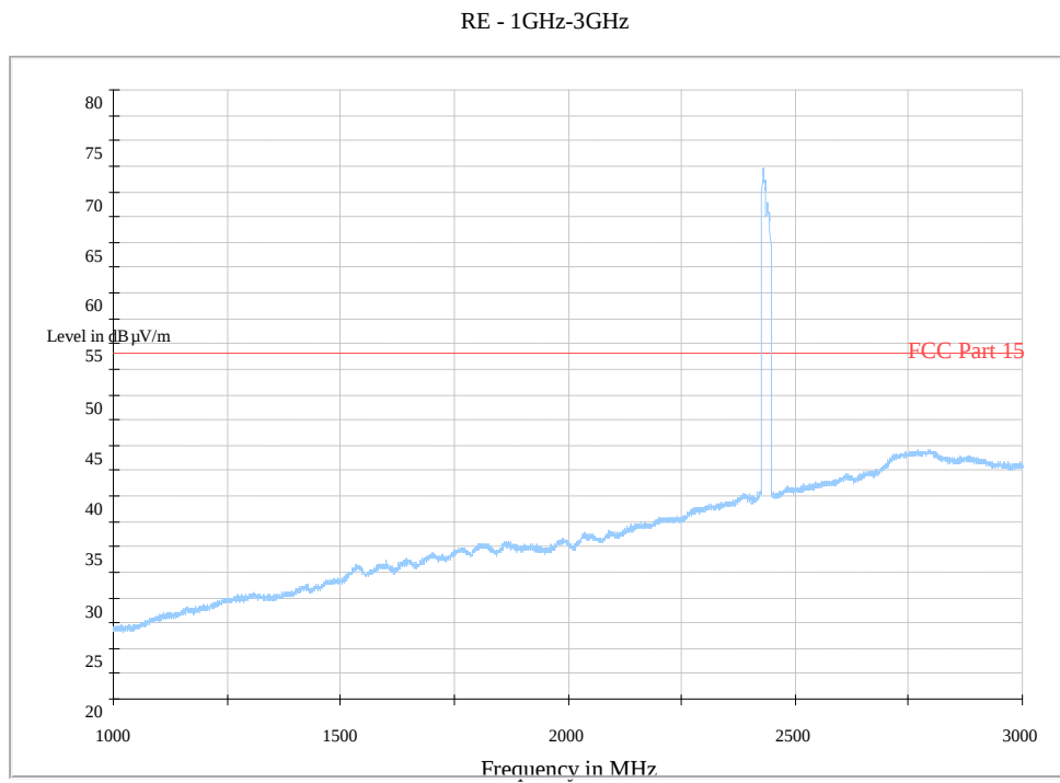
Fig. 156 Radiated Spurious Emission (802.11n-20MHz, Ch6, 1 GHz-3 GHz)
