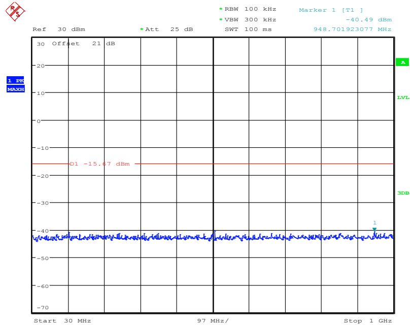
Fig. 73 Conducted Spurious Emission (802.11g, Ch11, Center Frequency)
