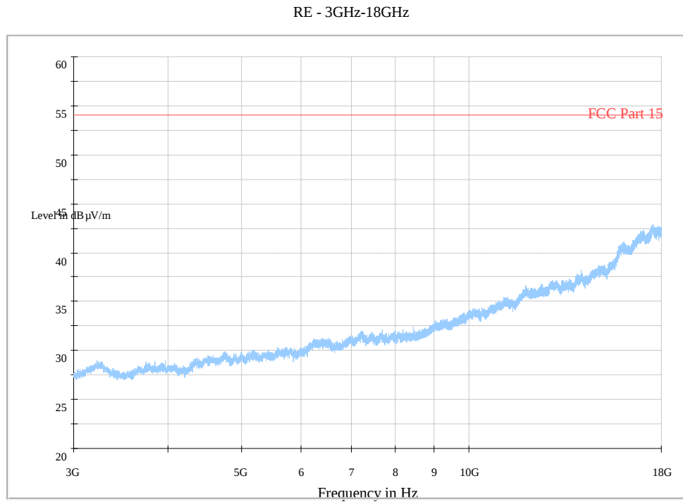
Fig. 165 Radiated Spurious Emission (802.11n-40MHz, Ch3, 3 GHz-18 GHz)
