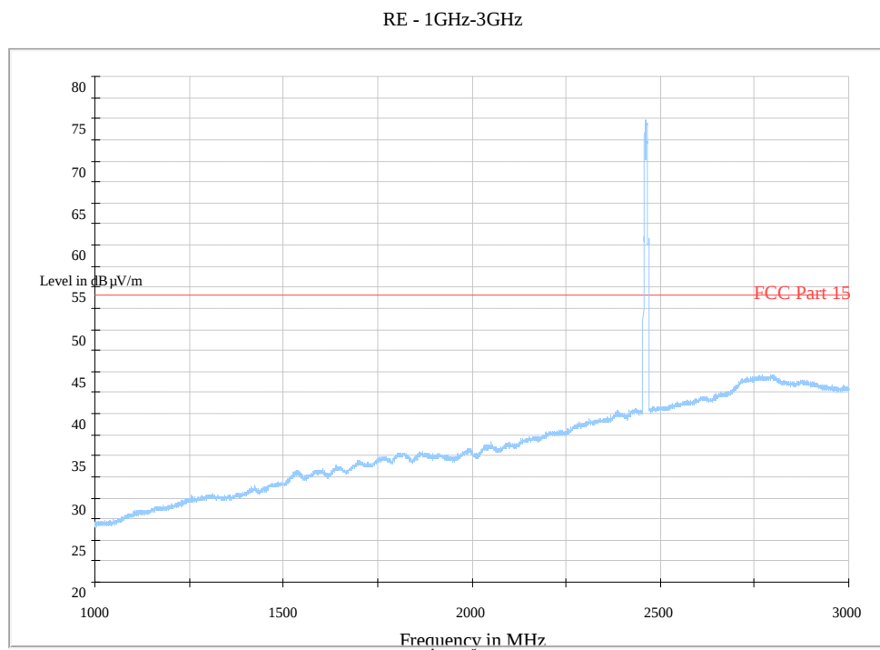
Fig. 138 Radiated Spurious Emission (802.11b, Ch11, 1 GHz-3 GHz)
