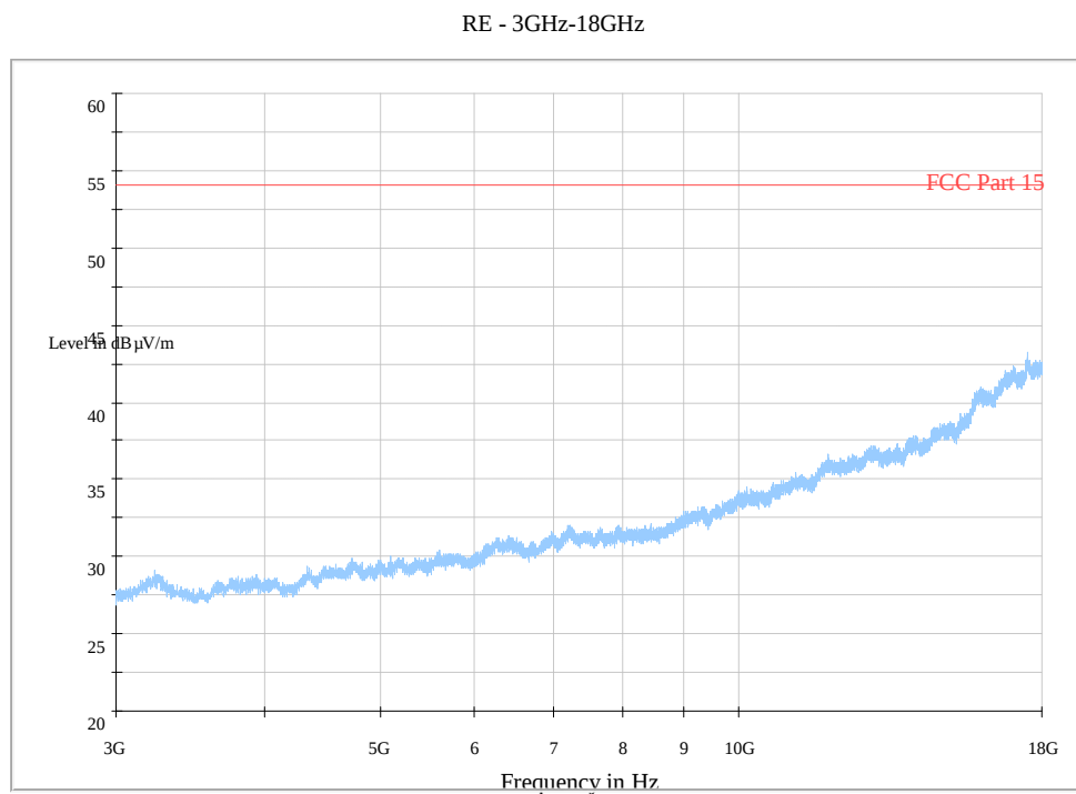
Fig. 146 Radiated Spurious Emission (802.11g, Ch6, 3 GHz-18 GHz)
