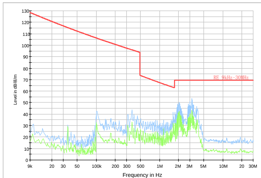
RE 9kHz-30MHz
