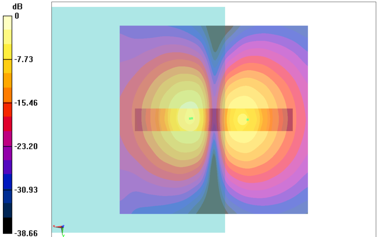
Fig B.1 T-Coil GSM 850
