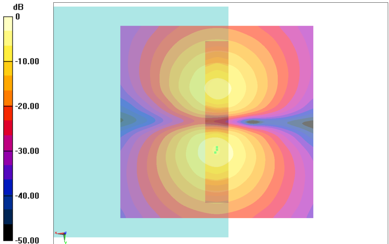
Fig B.2 T-Coil GSM 850
