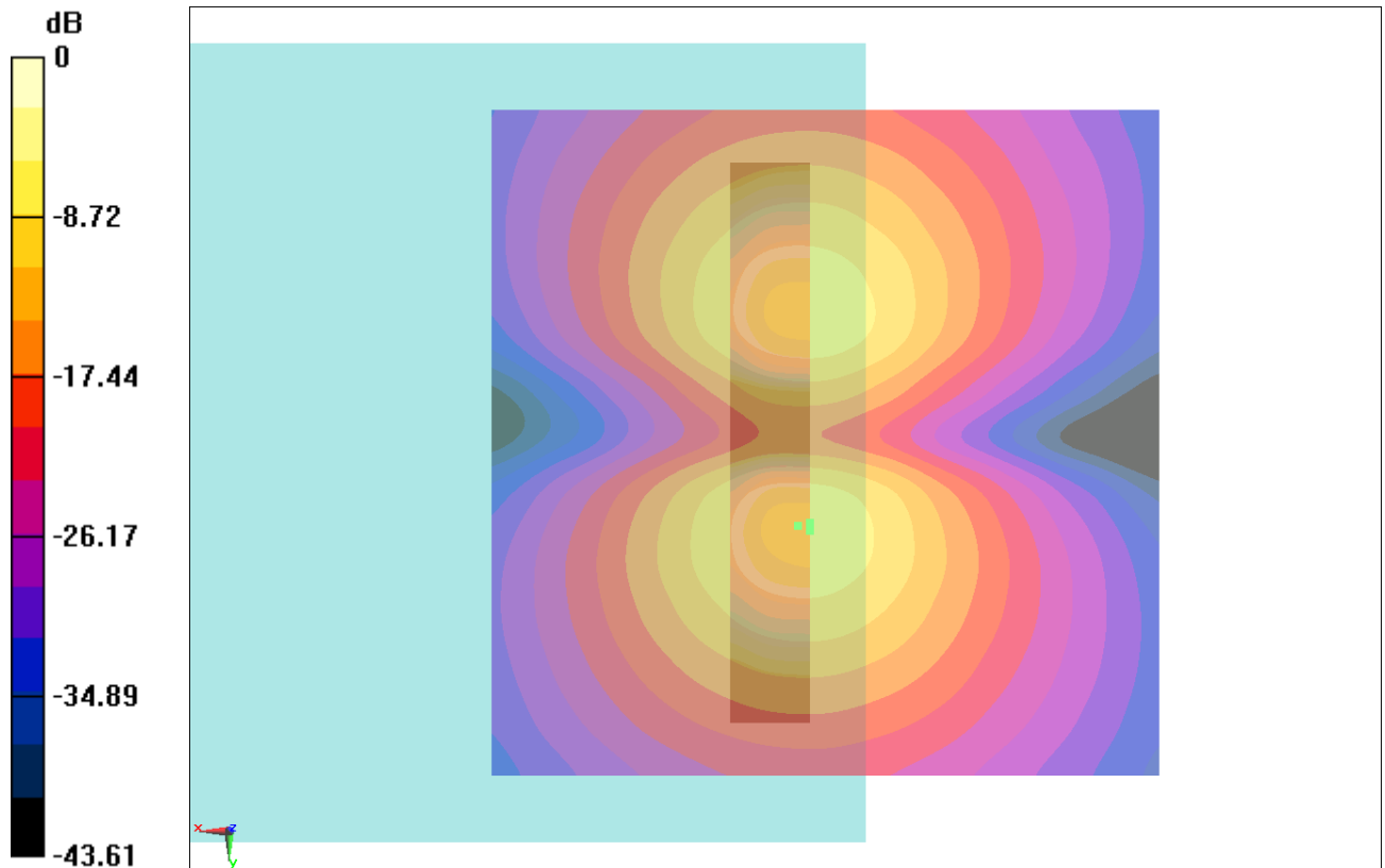
Fig B.5 T-Coil GSM 1900
