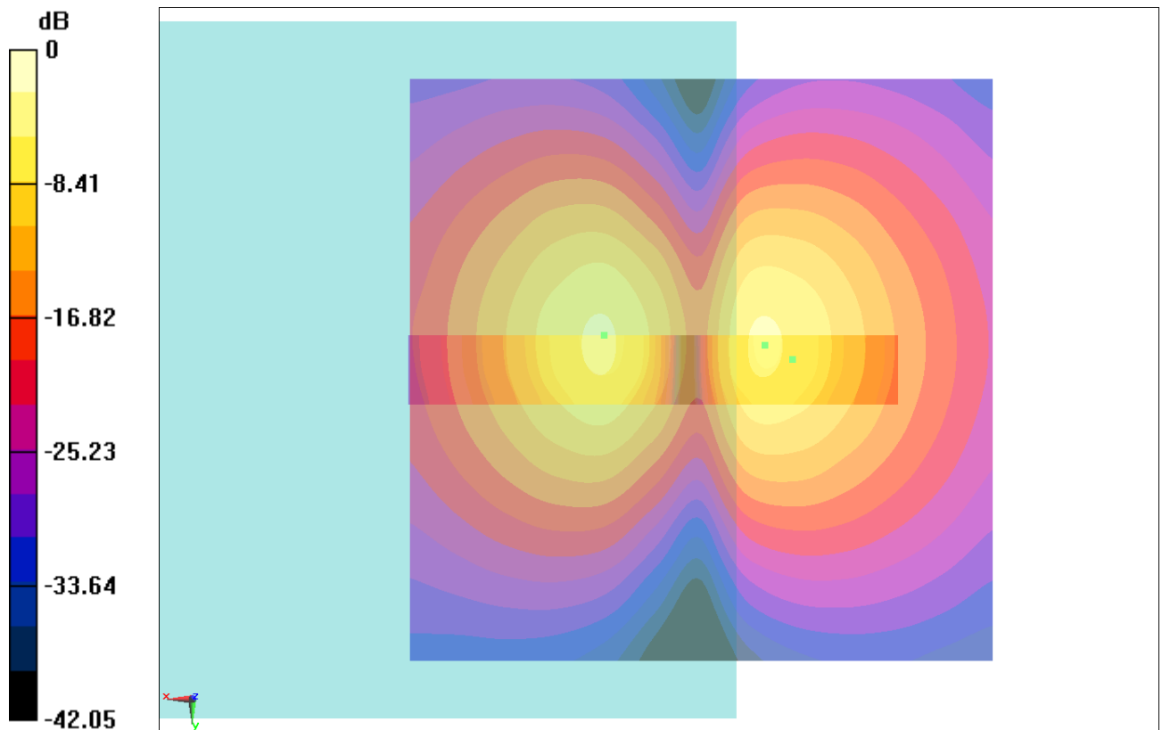
Fig B.4 T-Coil GSM 1900
