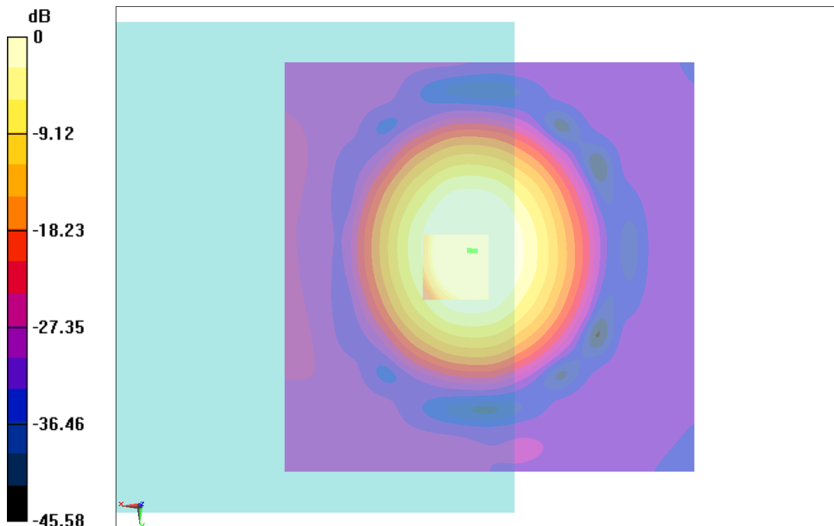
Fig B.6 T-Coil GSM 1900
