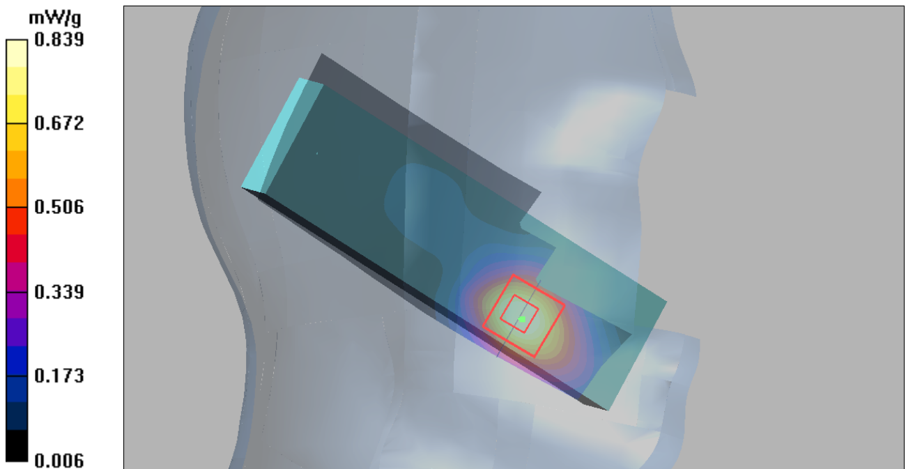
Figure 40 Left Hand Touch Cheek GSM 1900 Channel 512
