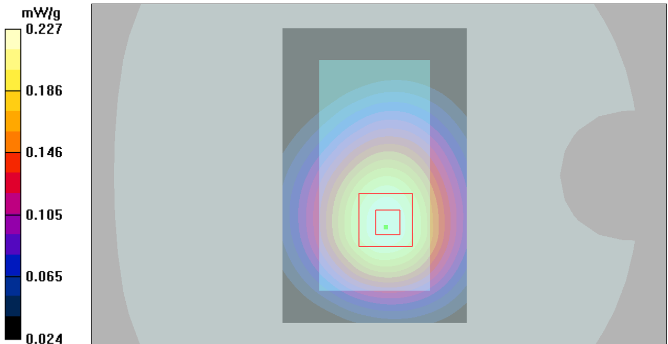
Figure 30 Body, Towards Phantom, GSM 850 Channel 251
