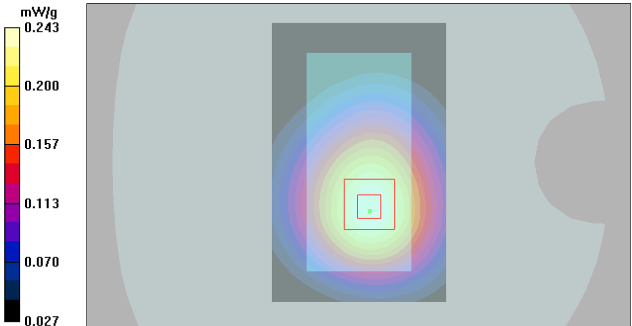
Figure 31 Body, Towards Phantom, GSM 850 Channel 190
