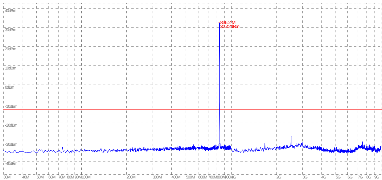
(Plot C2: EDGE 850MHz Channel = 190, 30MHz to 10GHz)
