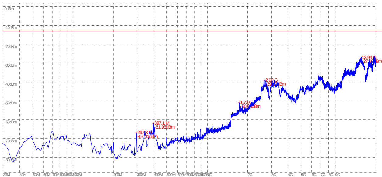
(Plot H.5: HSDPA 1900MHz Channel = 9938, Test Antenna Horizontal)
