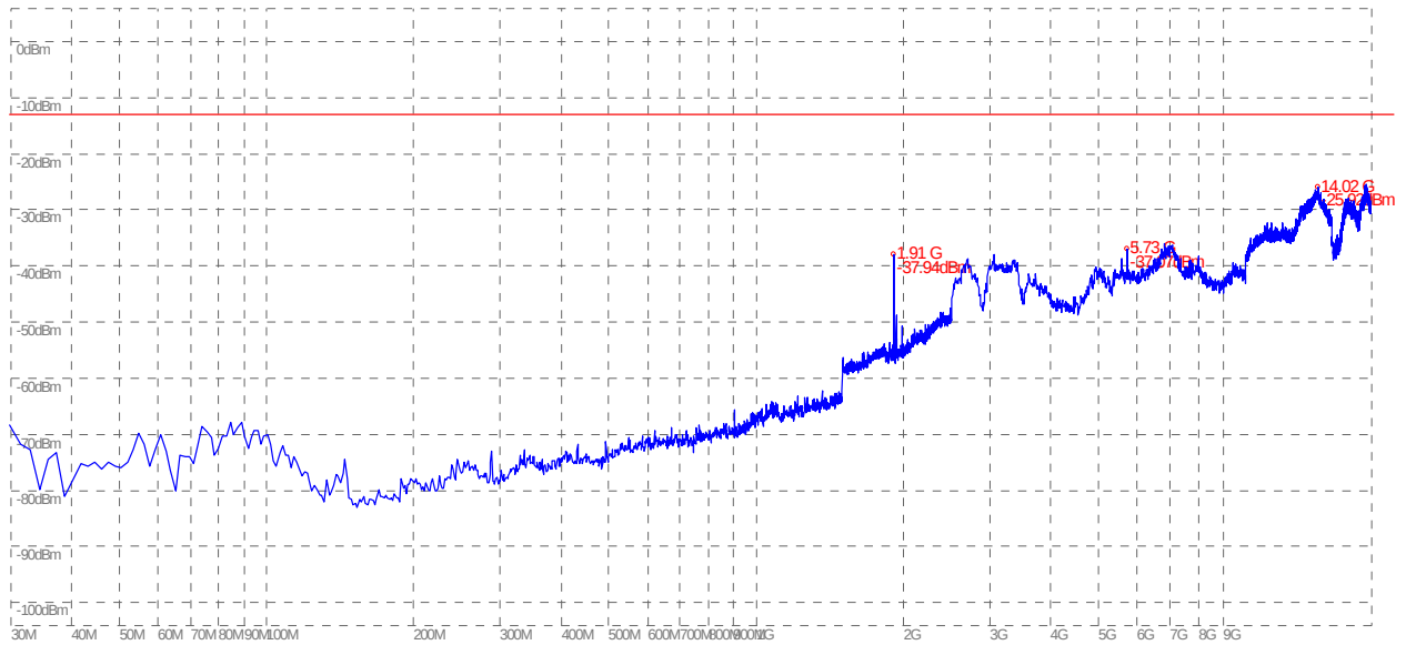
(PlotB.6: GSM 1900MHz Channel = 810, Test Antenna Vertical)
