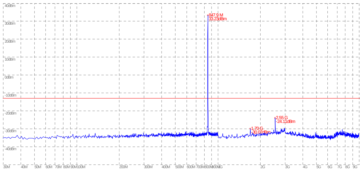
(Plot C3: EDGE 850MHz Channel = 251, 30MHz to 10GHz)
