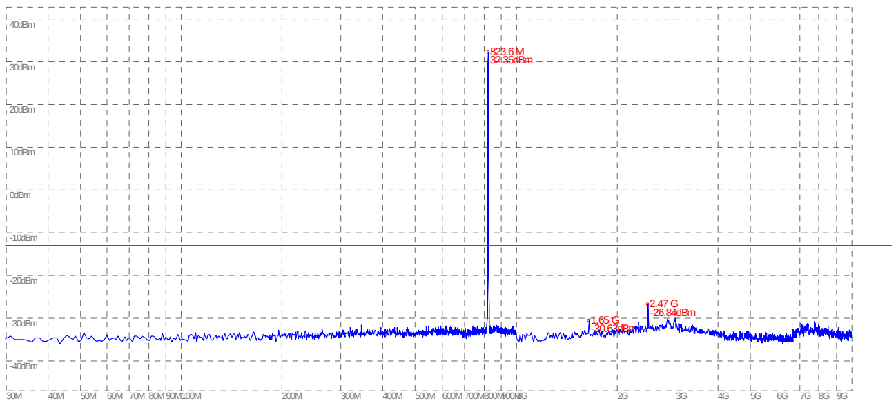
(Plot C1: EDGE 850MHz Channel = 128, 30MHz to 10GHz)
