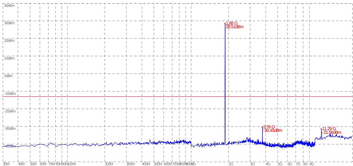
(Plot D2: EDGE 1900MHz Channel = 661, 30MHz to 20GHz)
