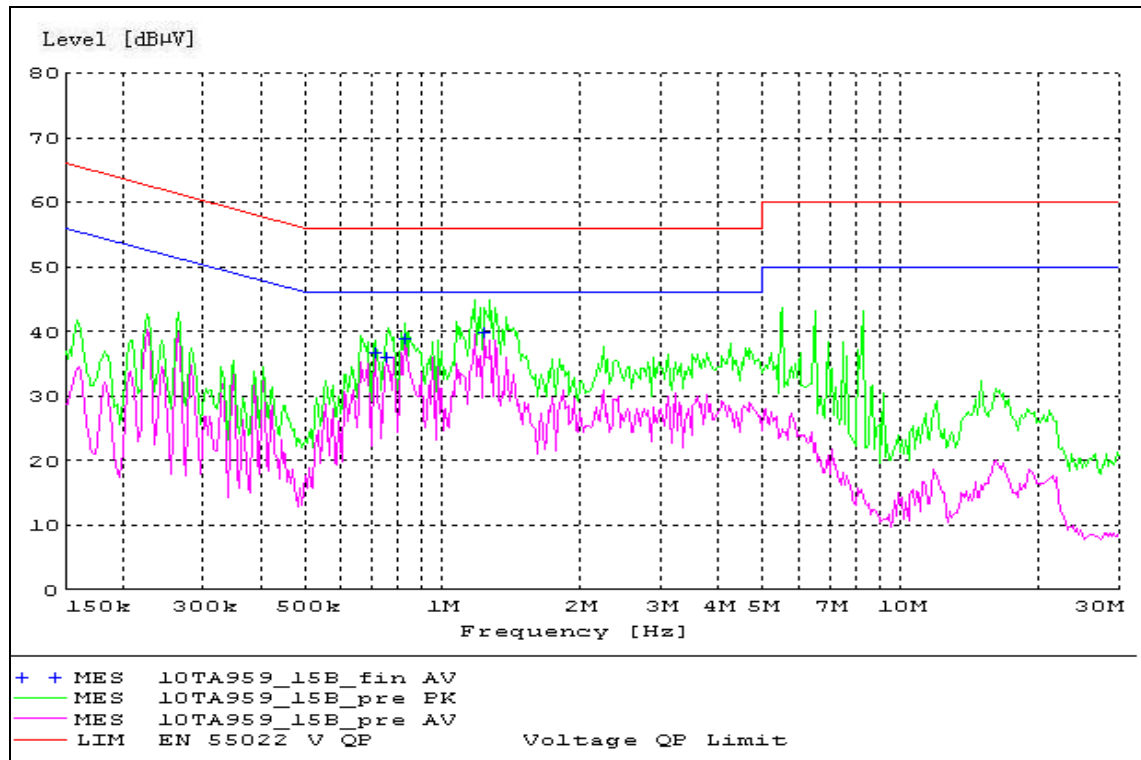
Figure A.9 Conducted Emission
