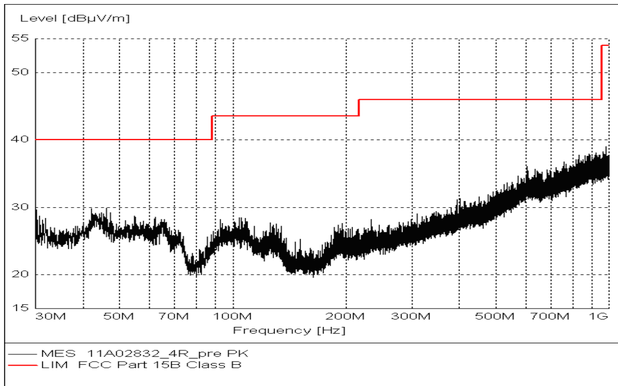
Figure A.5 Radiated Emission from 30MHz to 1GHz (set.3)
