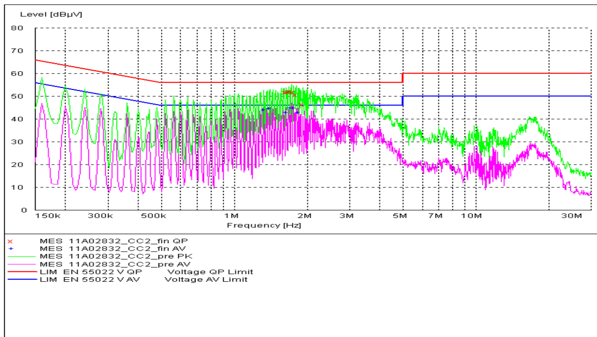
Figure A.10 Conducted Emission(set.2)
