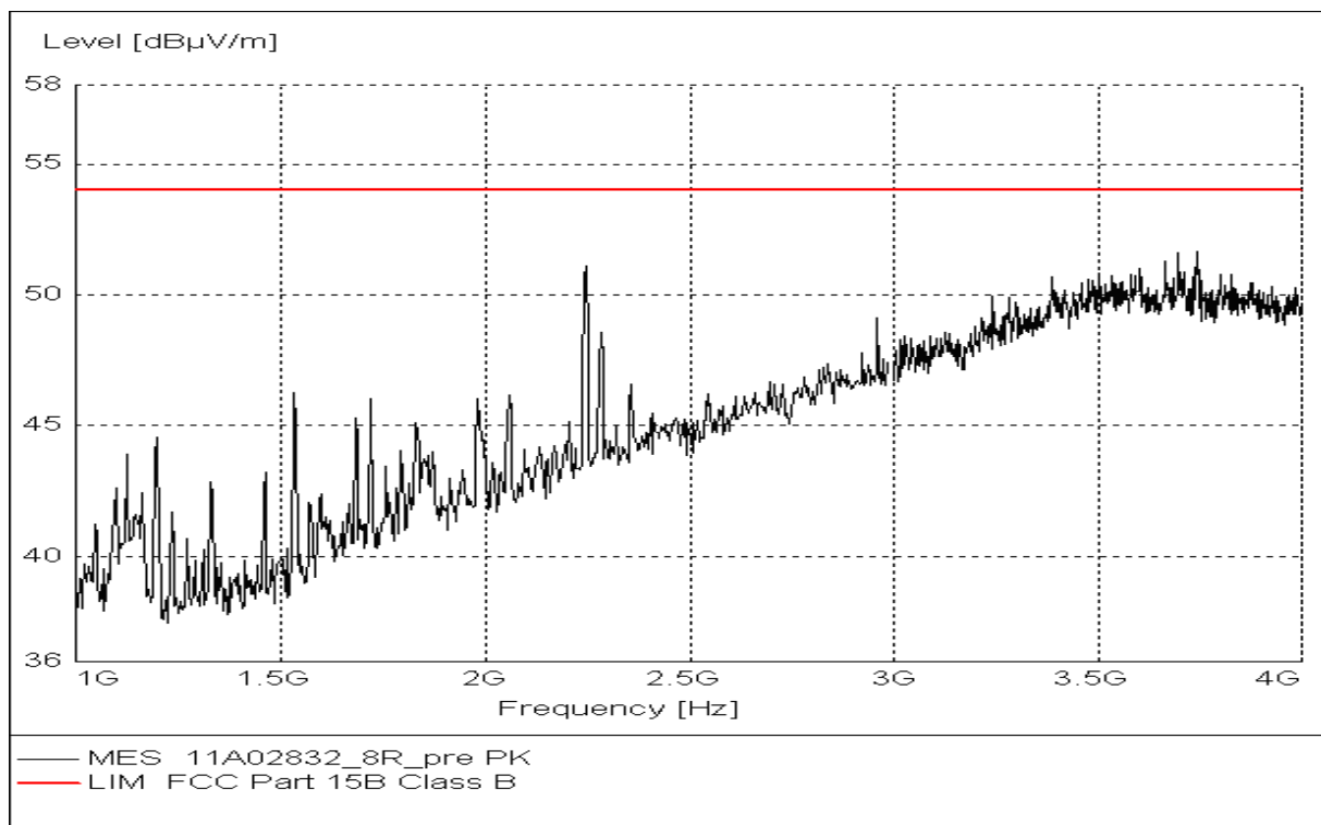
Figure A.8 Radiated Emission from 1GHz to 4GHz
