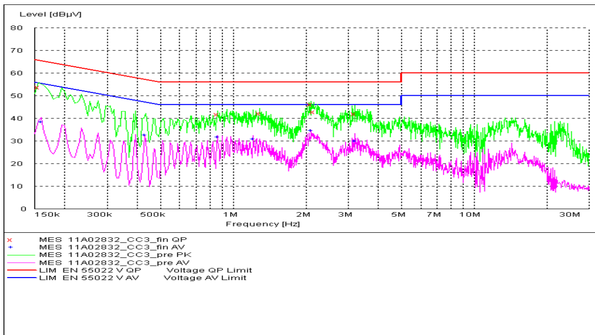
Figure A.11 Conducted Emission(set.3)
