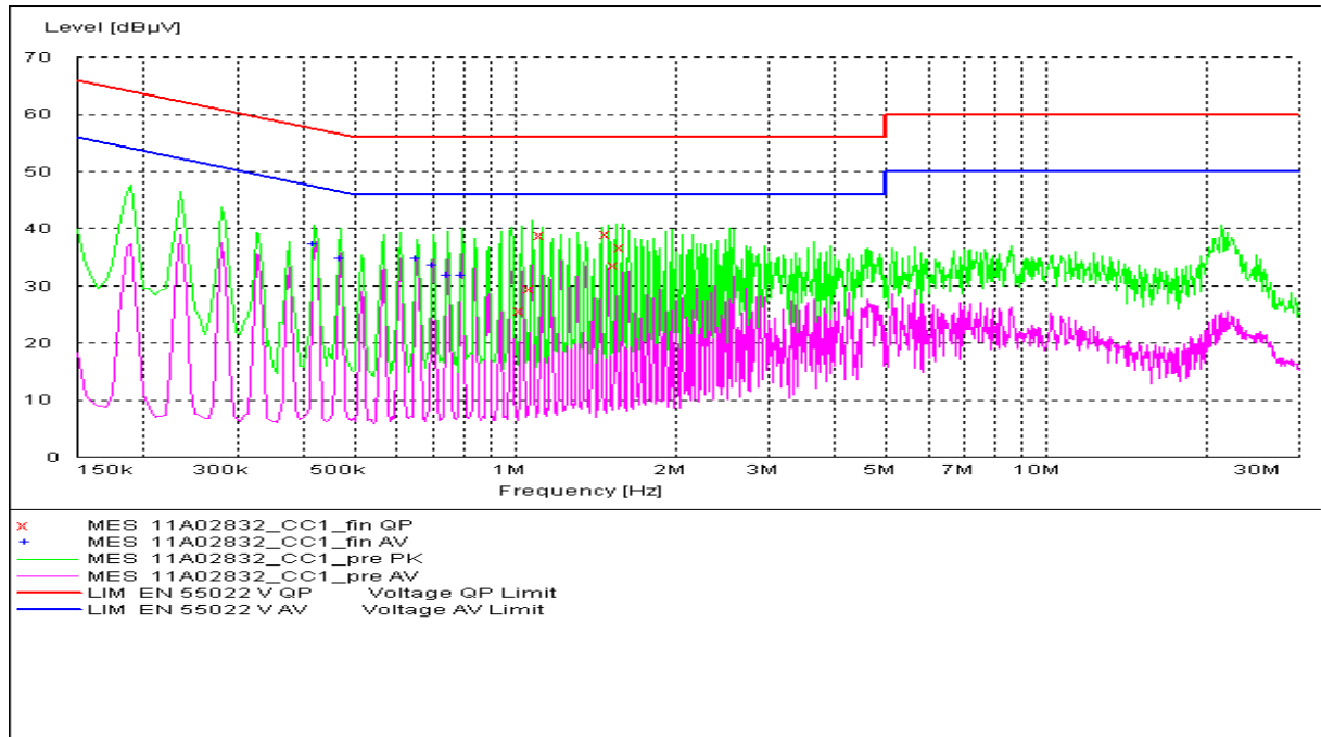
Figure A.9 Conducted Emission(set.1)
