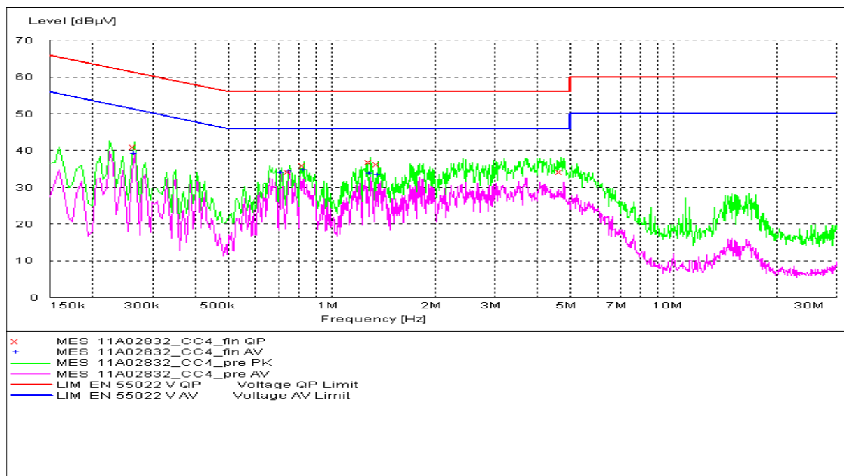
Figure A.12 Conducted Emission
