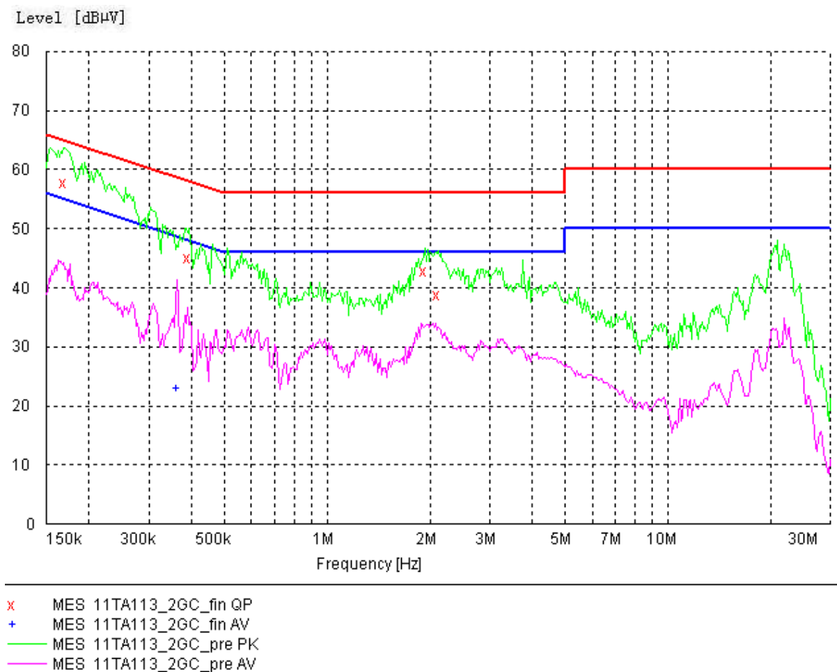
Figure A.8 Conducted Emission(AE4 CBA3001AG0C1)
