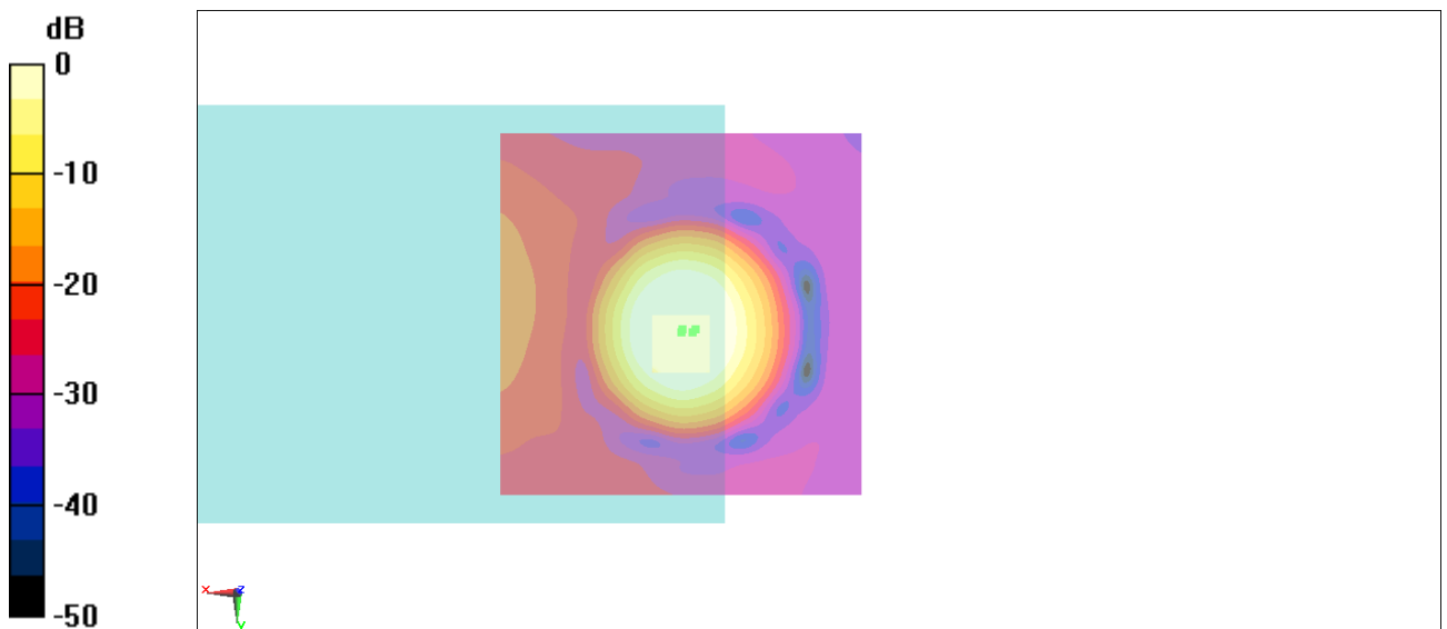
Fig B.9 T-Coil GSM 850 Channel 128
