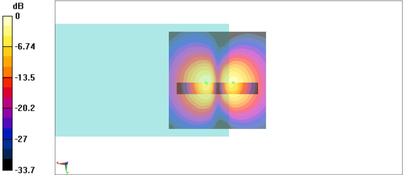
Fig B.7 T-Coil GSM 850 Channel 128
