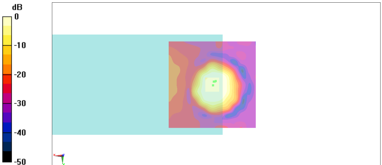
Fig B.6 T-Coil GSM 850 Channel 190
