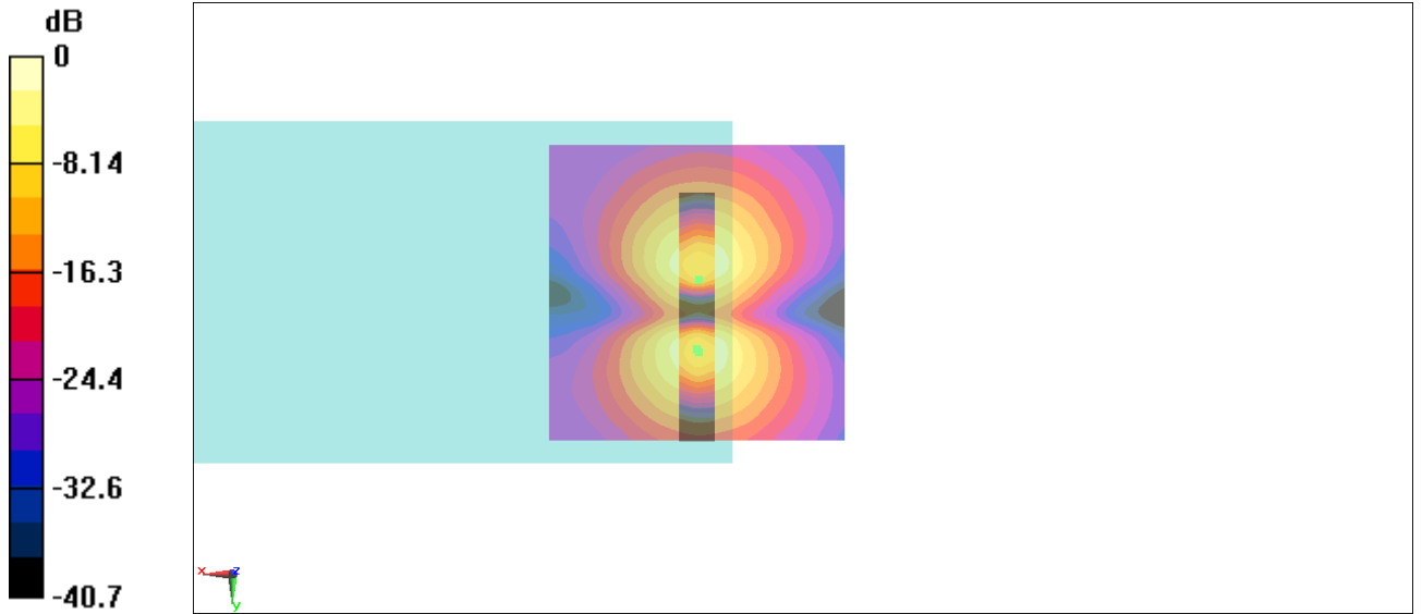
Fig B.2 T-Coil GSM 850 Channel 251
