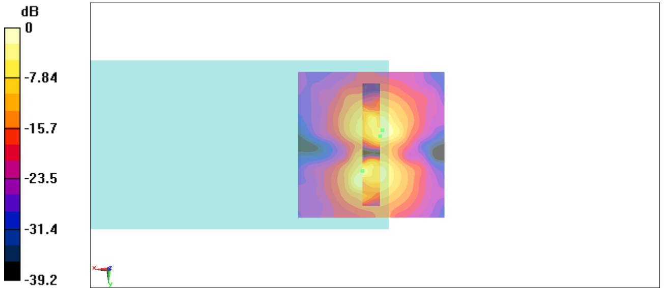
Fig B.5 T-Coil GSM 850 Channel 190
