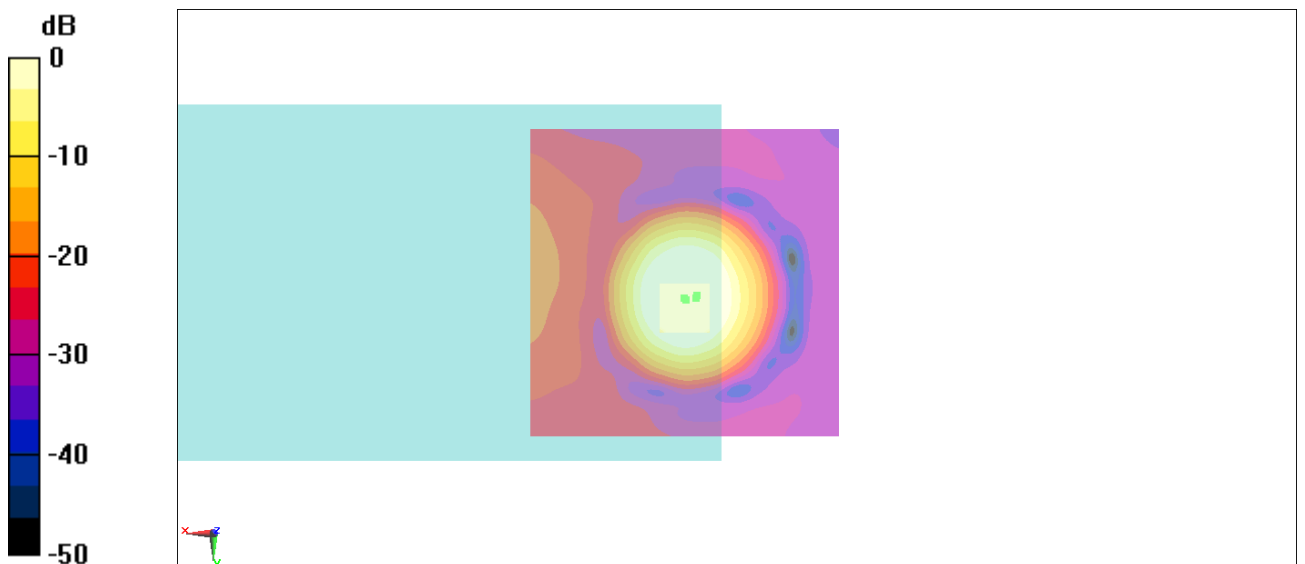
Fig B.3 T-Coil GSM 850 Channel 251
