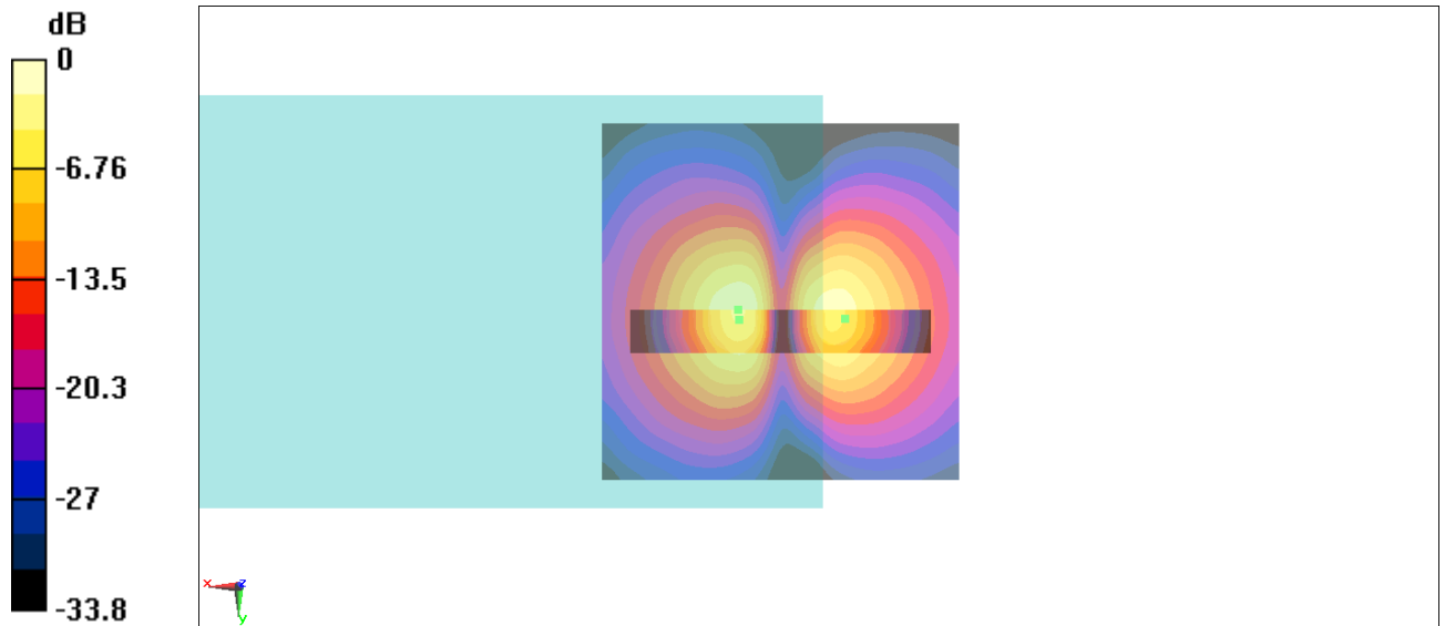
Fig B.1 T-Coil GSM 850 Channel 251
