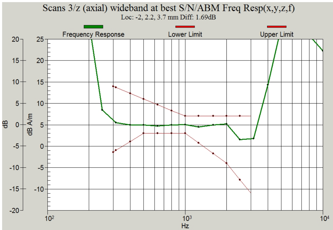
Figure C.3 Frequency Response of GSM 850 Channel 128
