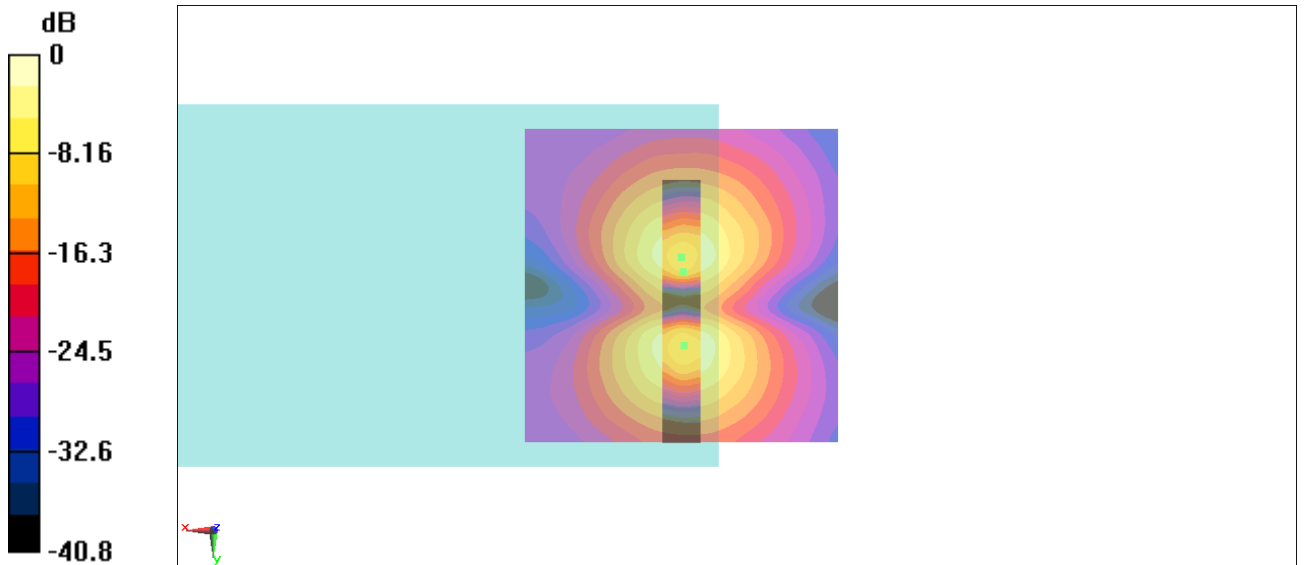
Fig B.8 T-Coil GSM 850 Channel 128
