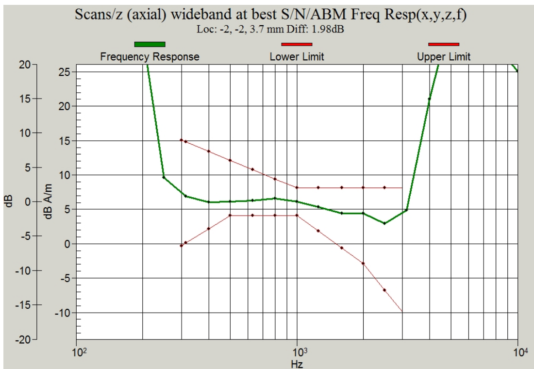
Figure C.2 Frequency Response of GSM 850 Channel 190
