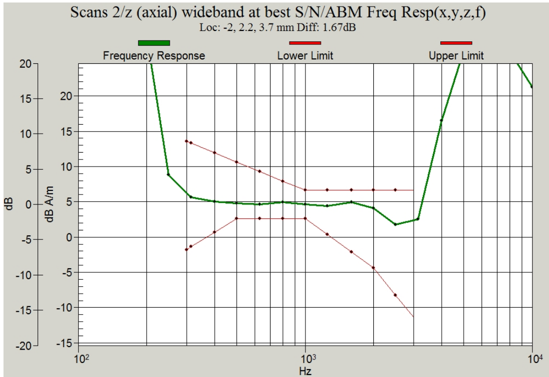
Figure C.1 Frequency Response of GSM 850 Channel 251
