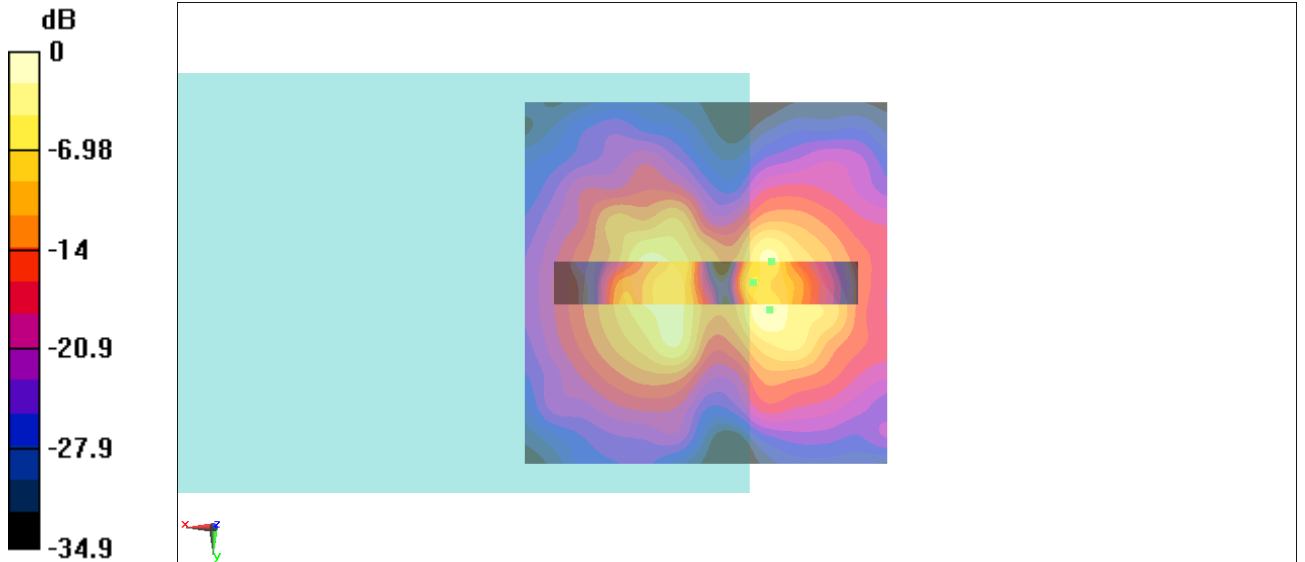
Fig B.4 T-Coil GSM 850 Channel 190
