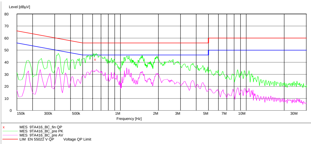
Fig. 34 AC Powerline Conducted Emission
