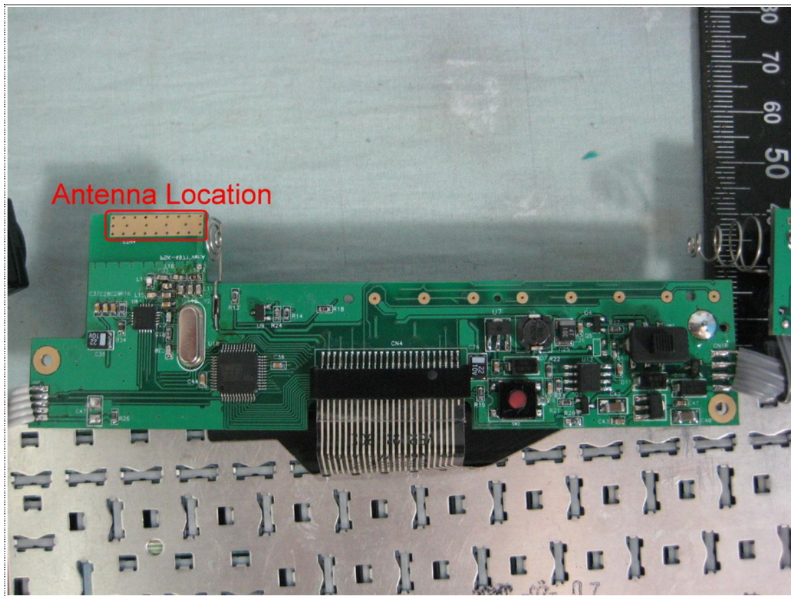
Antenna Location
