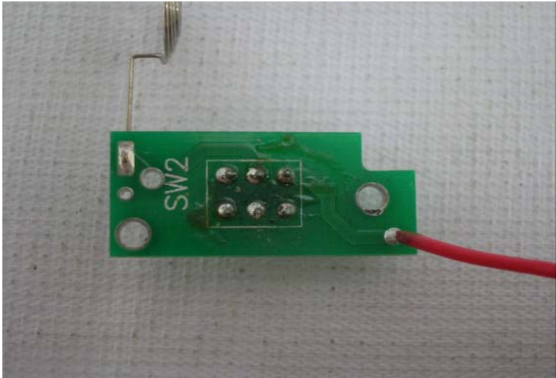
PHOTO. 14. EUT (TX) SOLDERING SIDE VIEW
