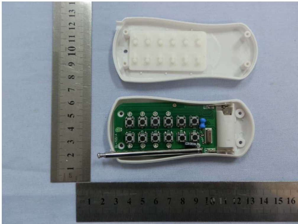
EUT - Open View (transmitter DL-1251A)
