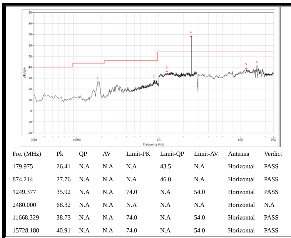
(Plot C.2: Antenna Horizontal, 30MHz to 25GHz)
