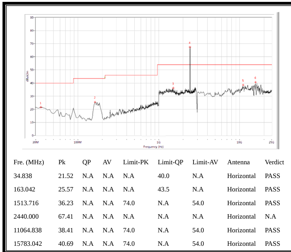
(Plot B.2: Antenna Horizontal, 30MHz to 25GHz)
