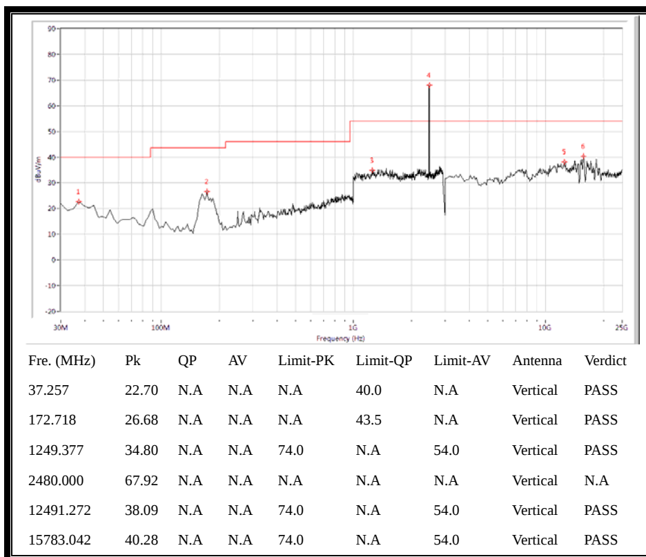
(Plot C.3: Antenna Vertical, 30MHz to 25GHz)
