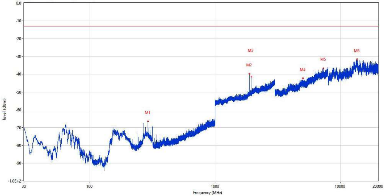
RSE(5G SA FCC)_RSE(5G FCC)_5G N2 & 25_1830-1920_30MHz-20GHz
