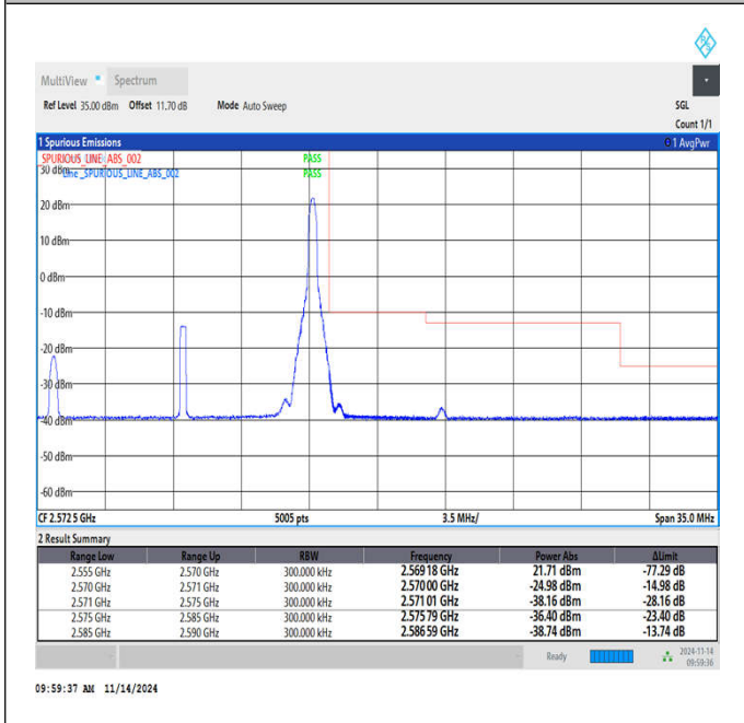
Band7_15MHz_64QAM_21375_1RB#74
