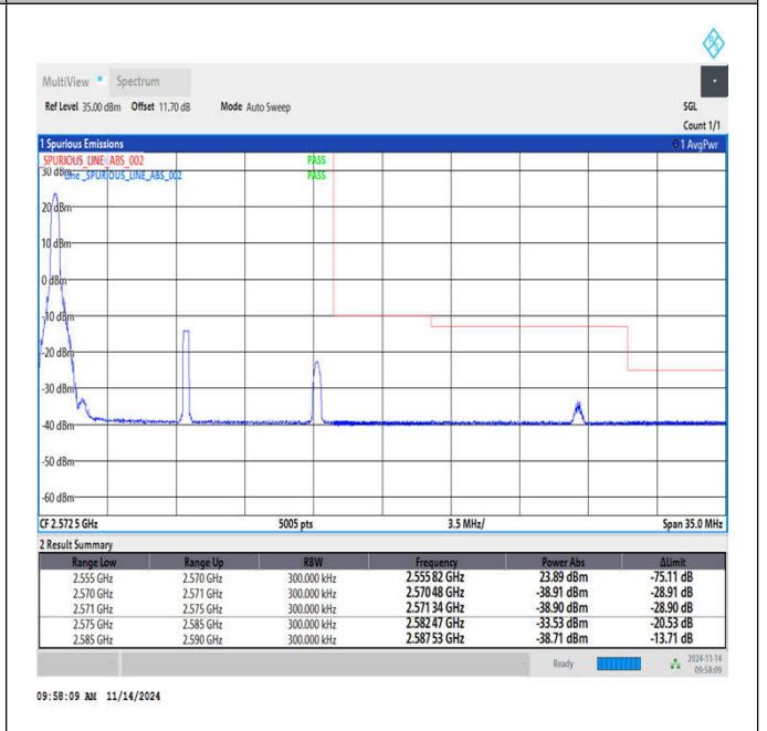
Band7_15MHz_16QAM_21375_1RB#0
