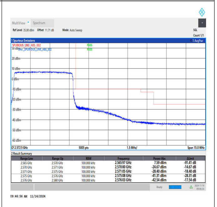
Band7_5MHz_64QAM_21425_25RB#0
