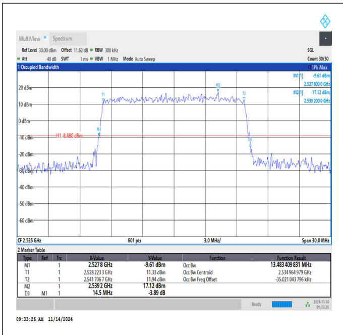
Band7-15MHz-16QAM-21100-75RB#0-PASS
