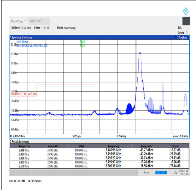
Band7_5MHz_64QAM_20775_1RB#0
