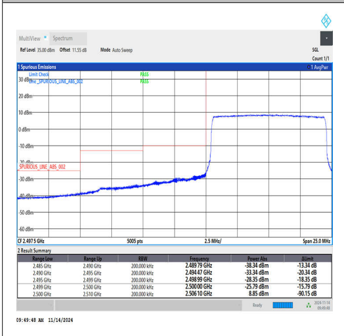
Band7_10MHz_QPSK_20800_50RB#0
