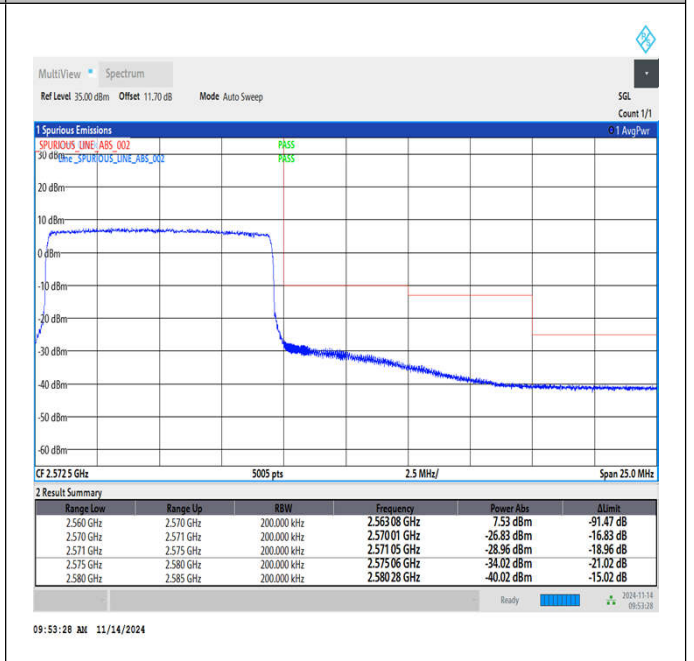
Band7_10MHz_16QAM_21400_50RB#0
