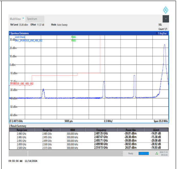
Band7_15MHz_16QAM_20825_1RB#74
