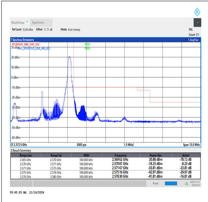
Band7_5MHz_16QAM_21425_1RB#24
