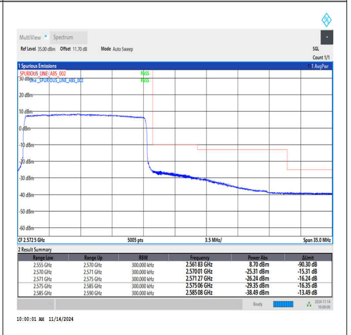
Band7_15MHz_QPSK_21375_75RB#0
