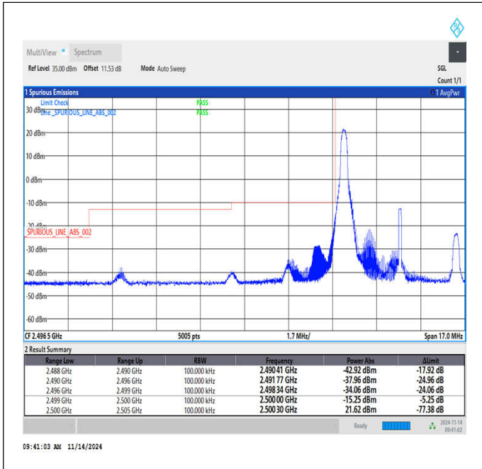
Band7_5MHz_16QAM_20775_1RB#0
