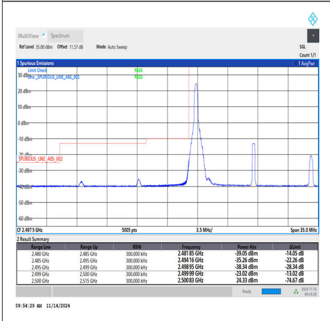
Band7_15MHz_QPSK_20825_1RB#0
