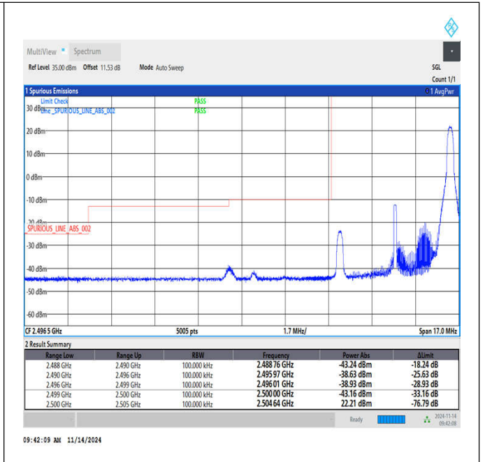
Band7_5MHz_16QAM_20775_1RB#0
