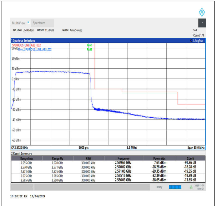
Band7_15MHz_16QAM_21375_75RB#0
