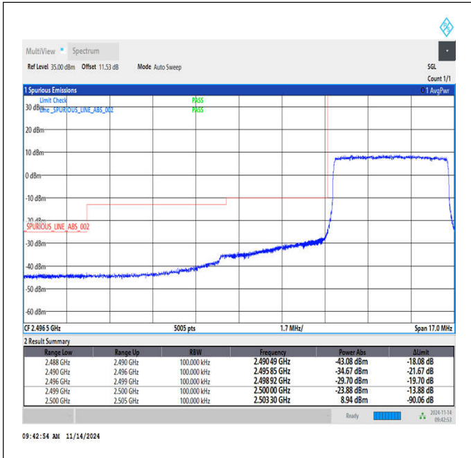
Band7_5MHz_QPSK_20775_25RB#0
