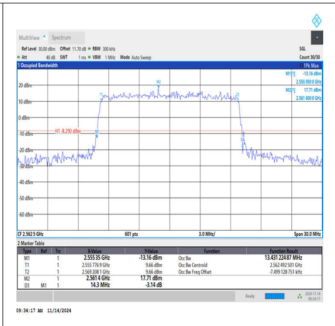
Band7-15MHz-16QAM-21375-75RB#0-PASS
