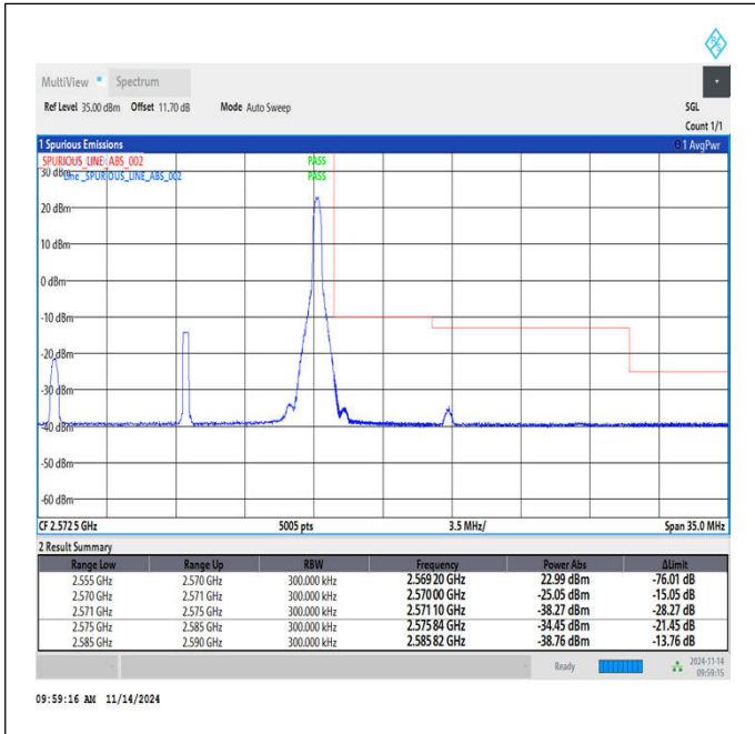
Band7_15MHz_16QAM_21375_1RB#74
