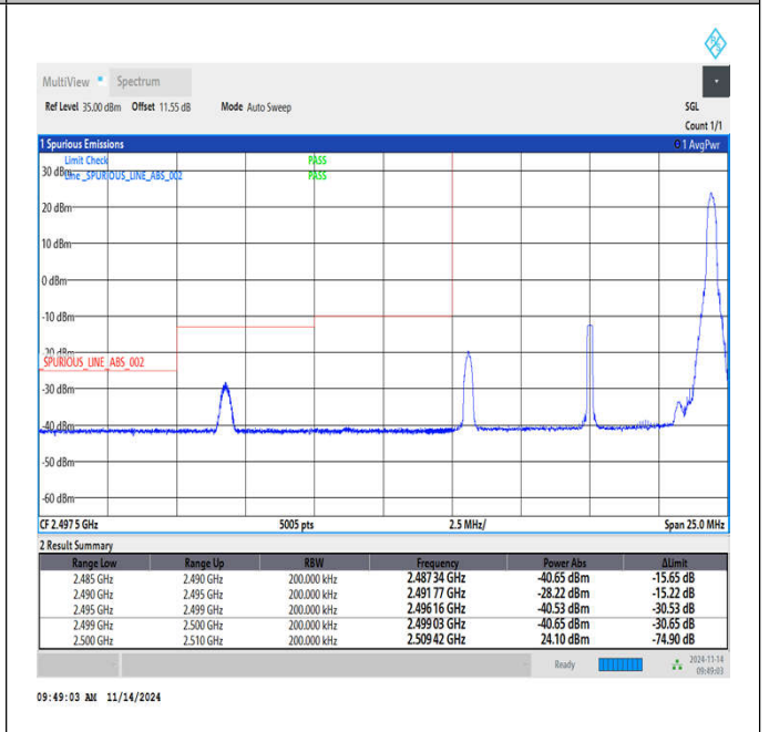
Band7_10MHz_16QAM_20800_1RB#49
