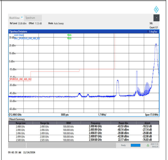
Band7_5MHz_64QAM_20775_1RB#24
