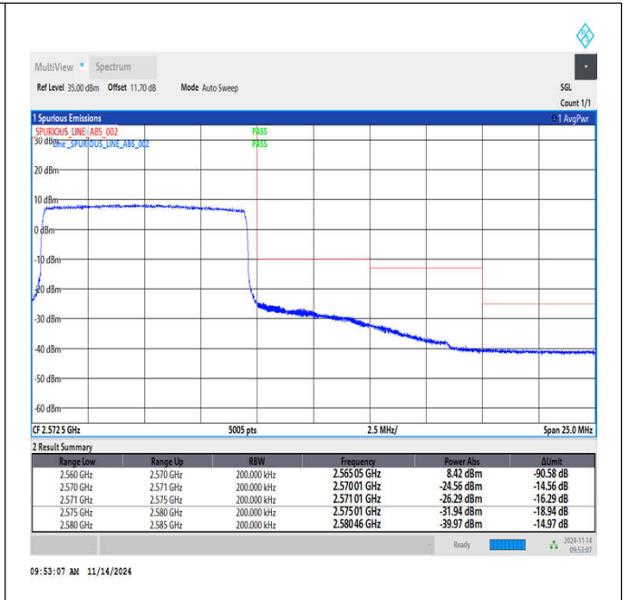
Band7_10MHz_QPSK_21400_50RB#0
