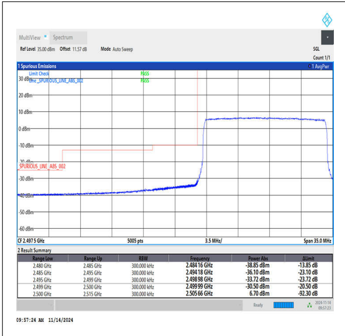
Band7_15MHz_64QAM_20825_75RB#0
