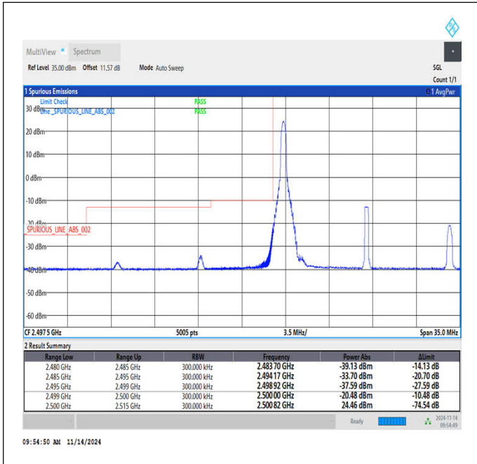
Band7_15MHz_16QAM_20825_1RB#0
