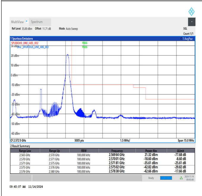
Band7_5MHz_QPSK_21425_1RB#24
