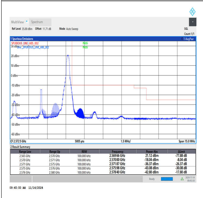
Band7_5MHz_64QAM_21425_1RB#24
