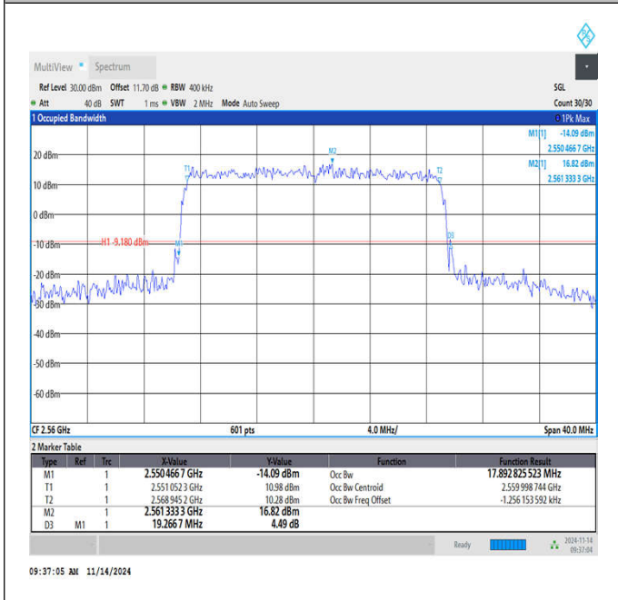
Band7-20MHz-16QAM-21350-100RB#0-PASS
