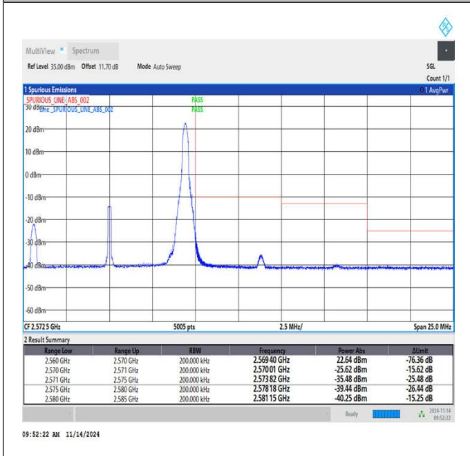
Band7_10MHz_16QAM_21400_1RB#49
