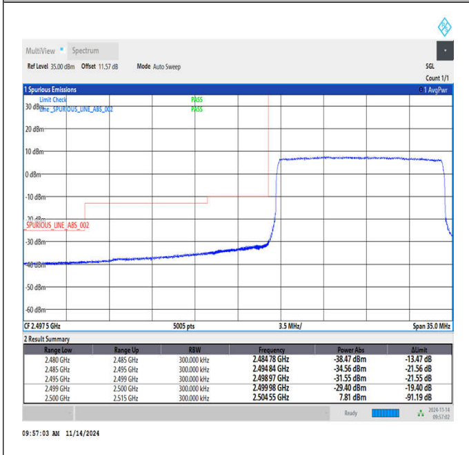
Band7_15MHz_16QAM_20825_75RB#0
