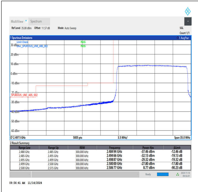
Band7_15MHz_QPSK_20825_75RB#0
