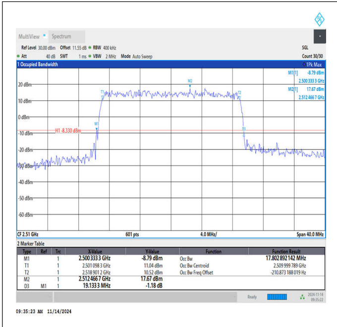
Band7-20MHz-16QAM-20850-100RB#0-PASS
