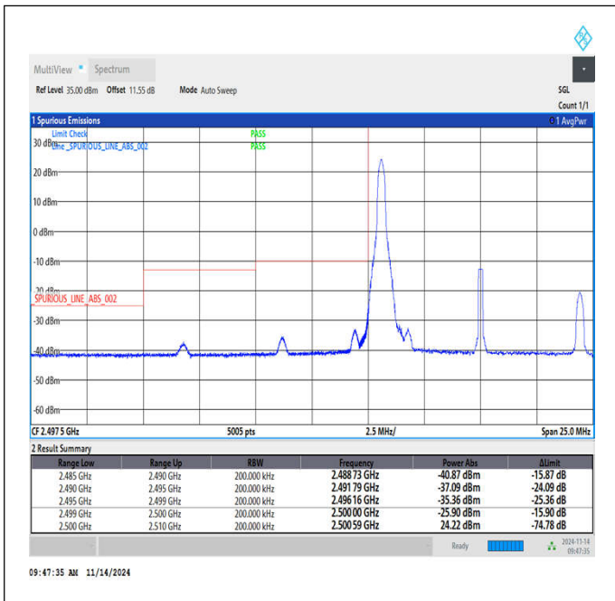
Band7_10MHz_QPSK_20800_1RB#0
