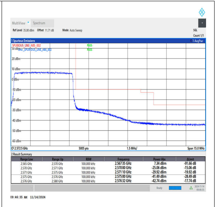
Band7_5MHz_16QAM_21425_25RB#0
