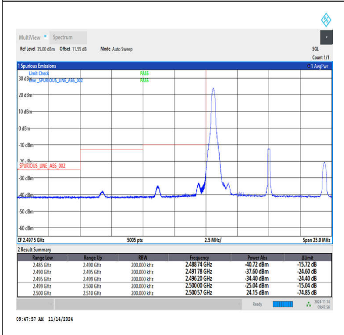
Band7_10MHz_16QAM_20800_1RB#0
