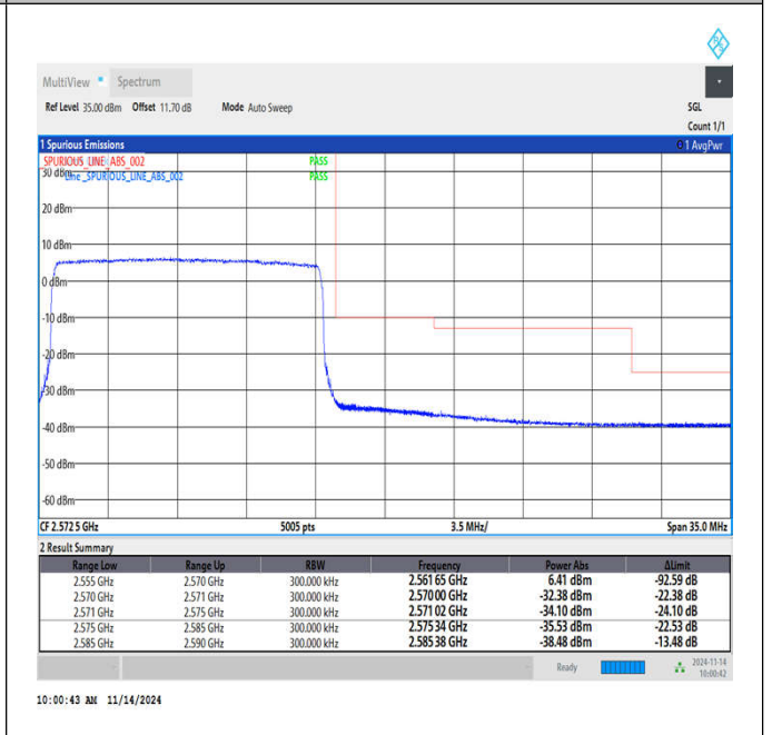
Band7_15MHz_64QAM_21375_75RB#0
