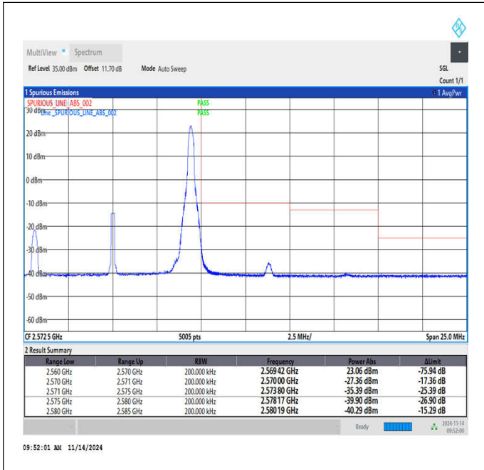
Band7_10MHz_QPSK_21400_1RB#49
