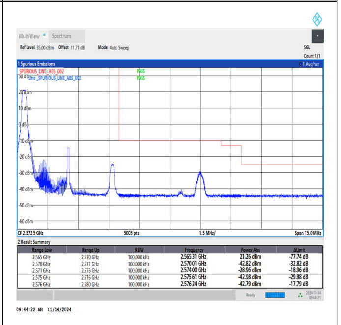
Band7_5MHz_16QAM_21425_1RB#0
