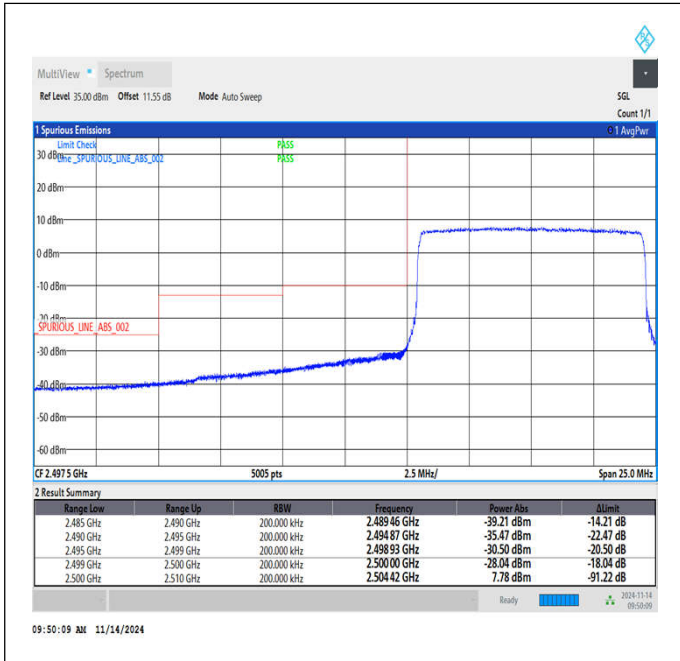
Band7_10MHz_16QAM_20800_50RB#0
