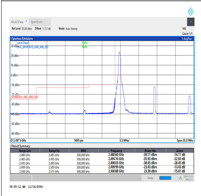
Band7_15MHz_64QAM_20825_1RB#0
