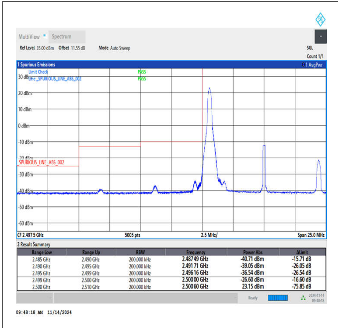
Band7_10MHz_64QAM_20800_1RB#0
