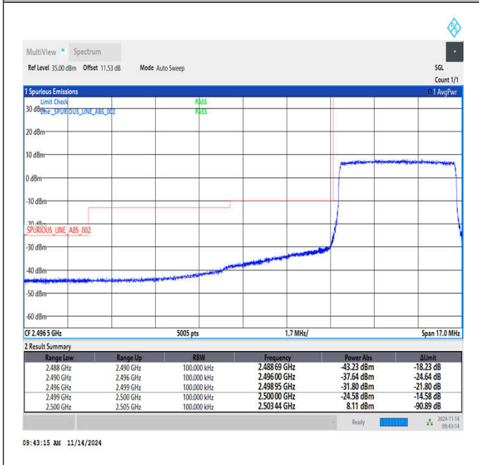
Band7_5MHz_16QAM_20775_25RB#0
