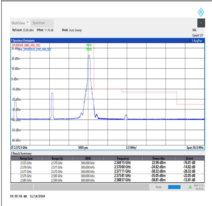
Band7_15MHz_QPSK_21375_1RB#74
