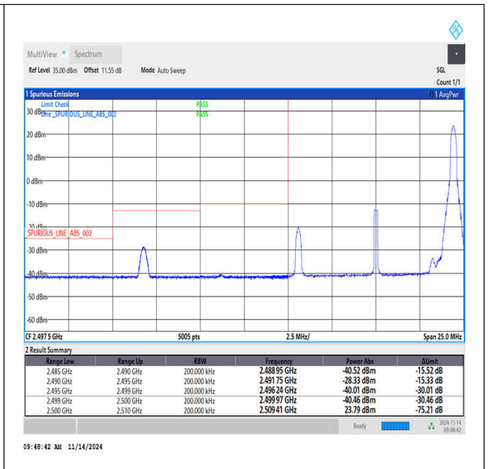
Band7_10MHz_QPSK_20800_1RB#49
