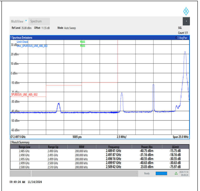
Band7_10MHz_64QAM_20800_1RB#49
