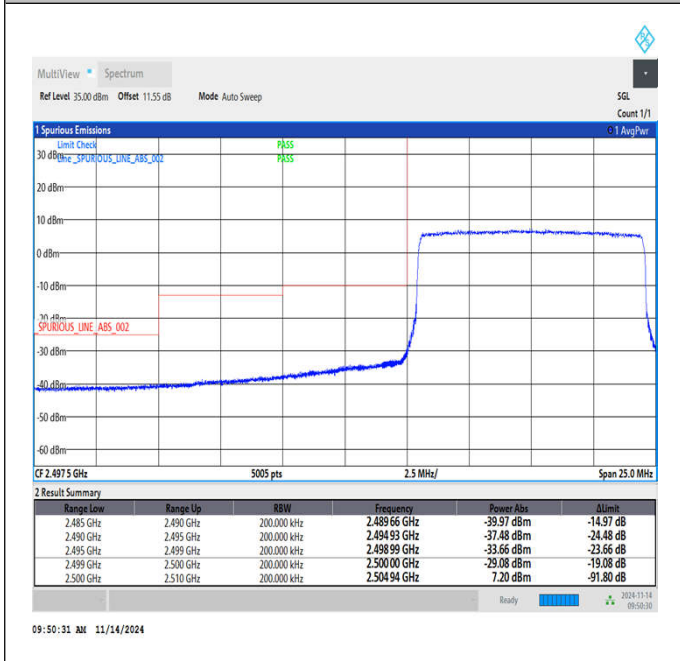
Band7_10MHz_64QAM_20800_50RB#0
