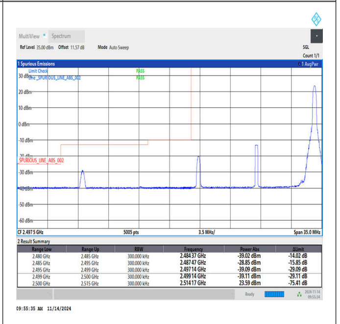
Band7_15MHz_QPSK_20825_1RB#74
