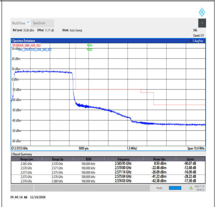
Band7_5MHz_QPSK_21425_25RB#0
