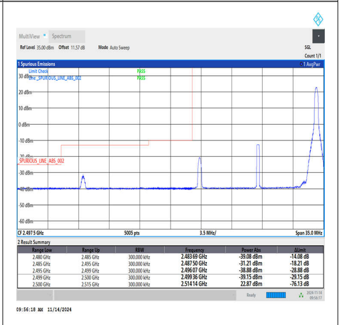
Band7_15MHz_64QAM_20825_1RB#74
