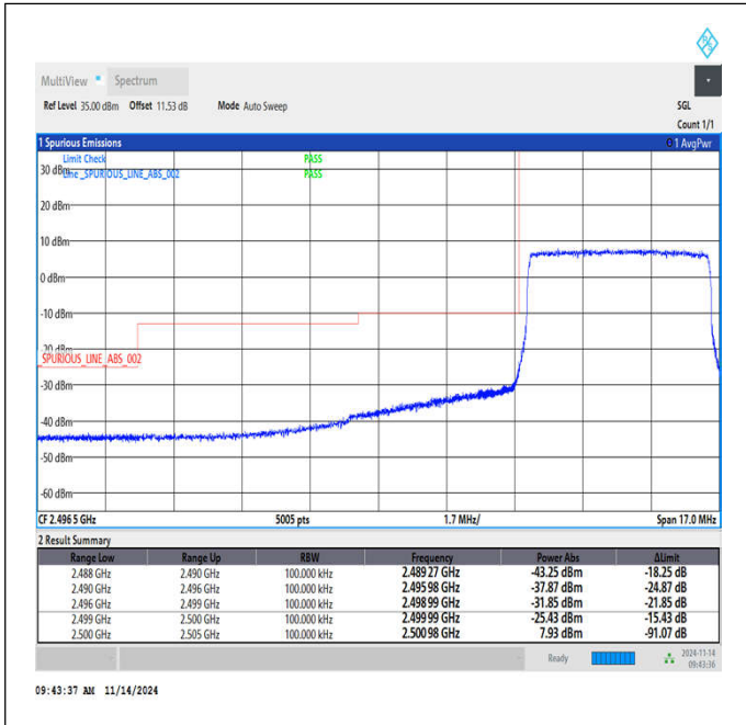
Band7_5MHz_64QAM_20775_25RB#0
