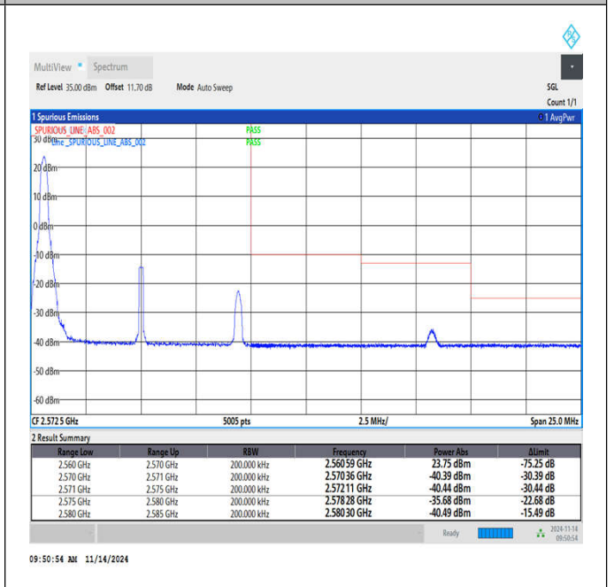
Band7_10MHz_QPSK_21400_1RB#0
