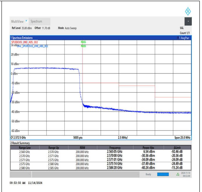
Band7_10MHz_64QAM_21400_50RB#0
