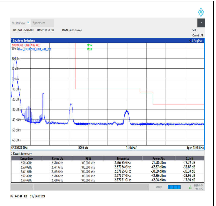
Band7_5MHz_64QAM_21425_1RB#0
