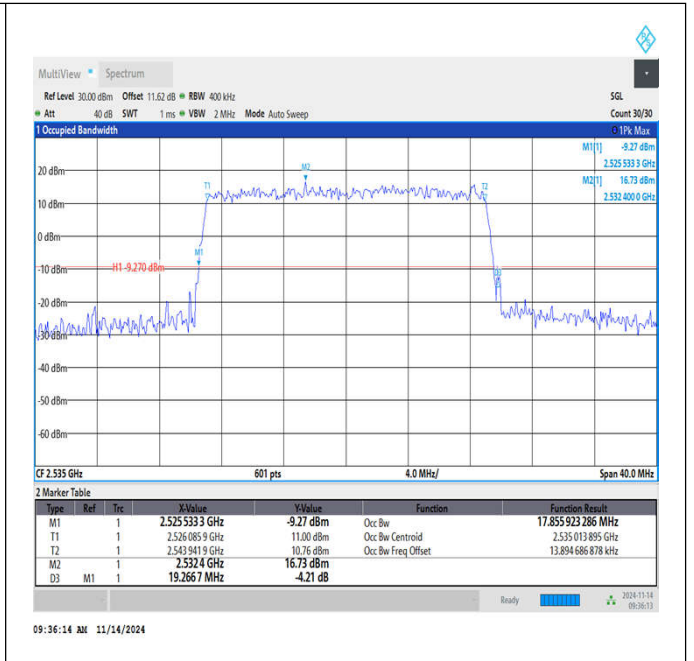
Band7-20MHz-16QAM-21100-100RB#0-PASS
