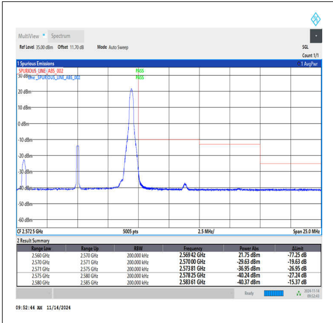
Band7_10MHz_64QAM_21400_1RB#49
