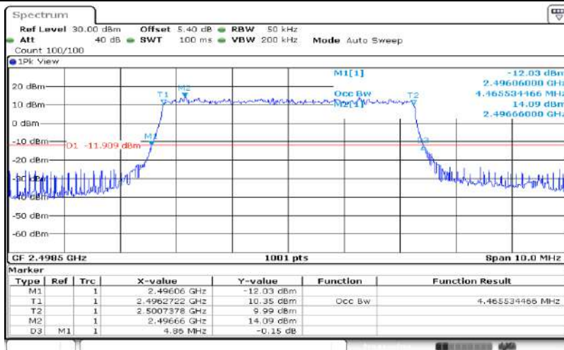
Band41-5MHz-QPSK-39675-25RB#0-4.466
