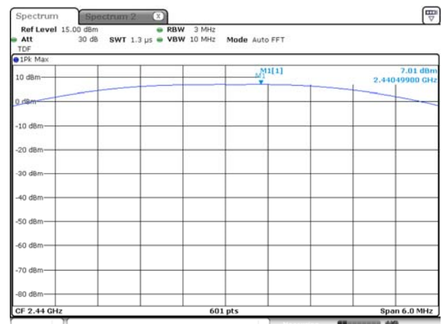
GFSK (BLE 2Mbps) MIDDLE CHANNEL
