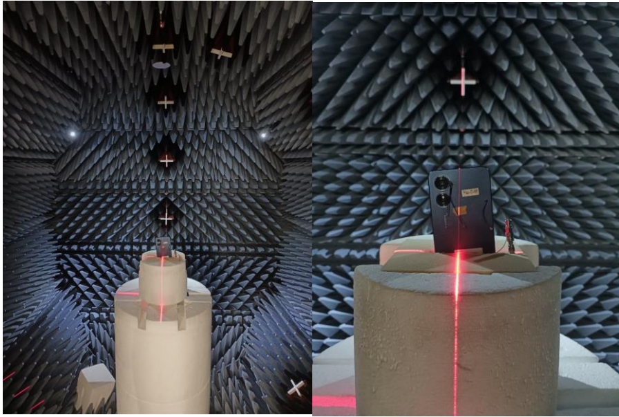
Fig.1. The DUT in the fully anechoic chamber
