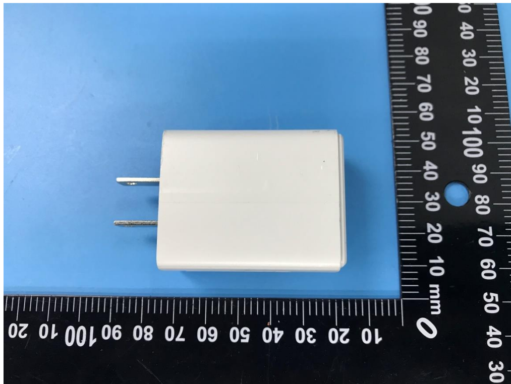
Photo 7 Appearance of adapter (OP52YAUH)
