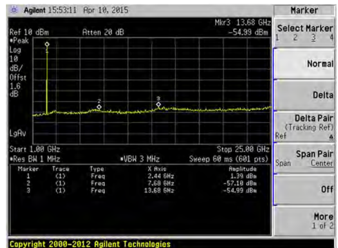
MIDDLE CHANNEL, SPURIOUS 1 GHz ~ 25 GHz
