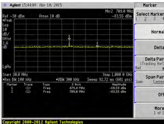
MIDDLE CHANNEL, SPURIOUS 30 MHz ~ 1 GHz
