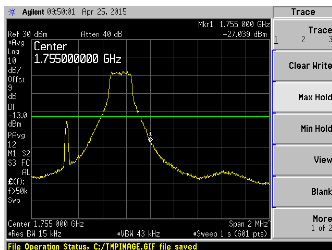
Band 4 16-QAM 1.4 MHz RB1#5 HCH
