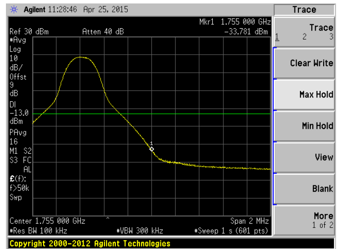
Band 4 16-QAM 10 MHz RB1#49 HCH
