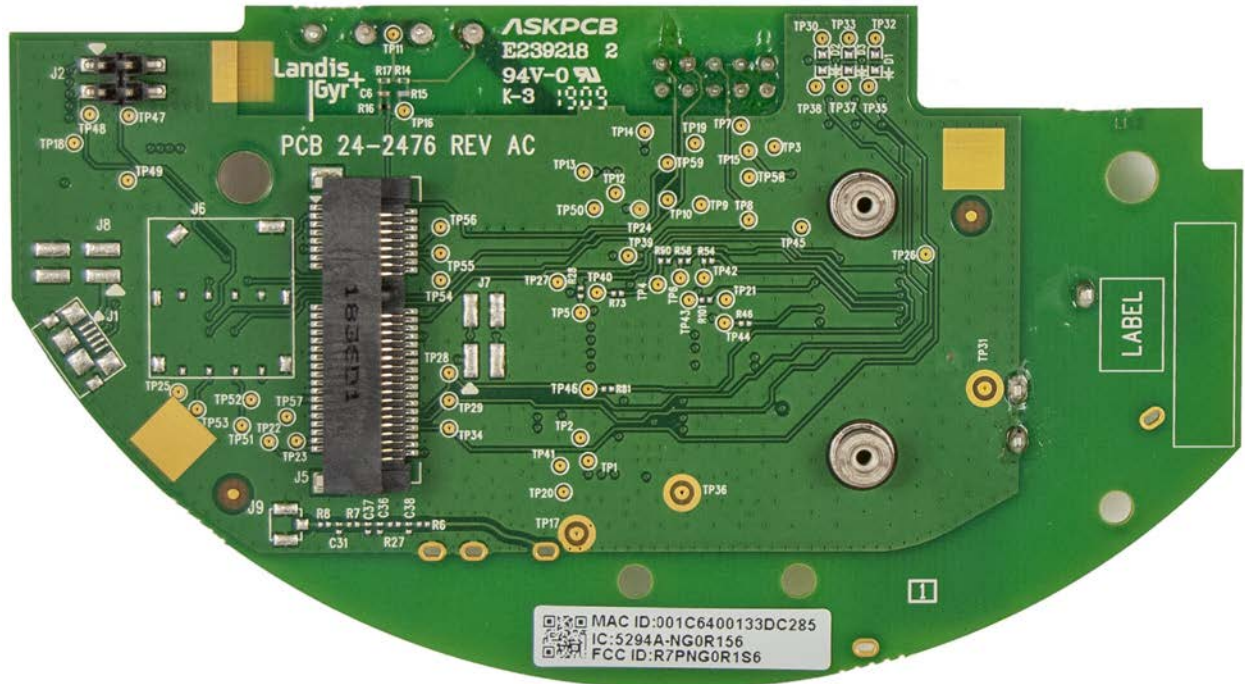
Figure 3: Bottom View
