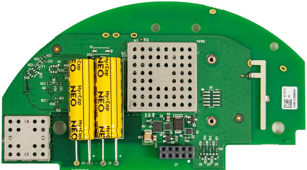
Figure 1: Top View with Shields
