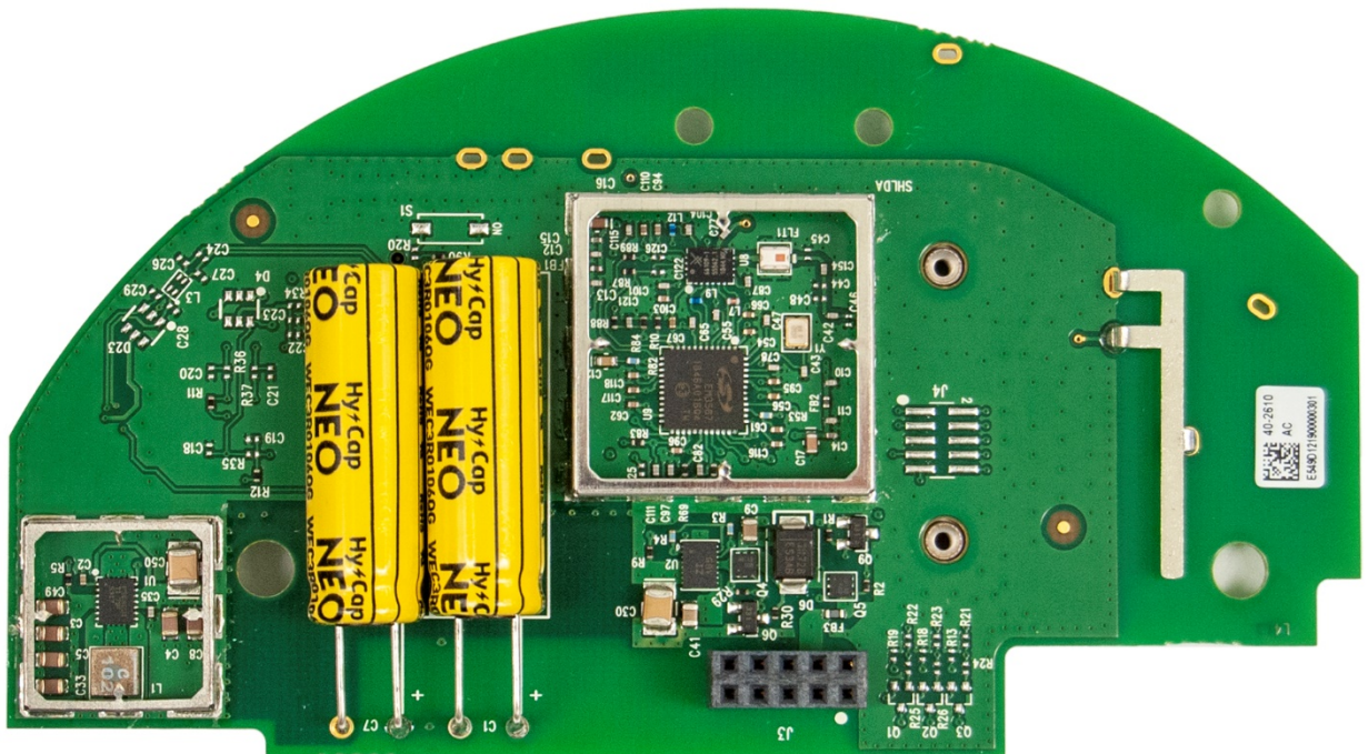
Figure 2: Top View without Shields
