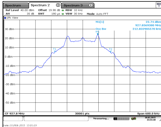
Figure 7.4.4.2-40: 99% BW High Channel – 115.2kbps
