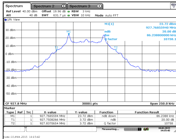
Figure 7.4.4.2-18: 20dB BW High Channel – 50.0kbps
