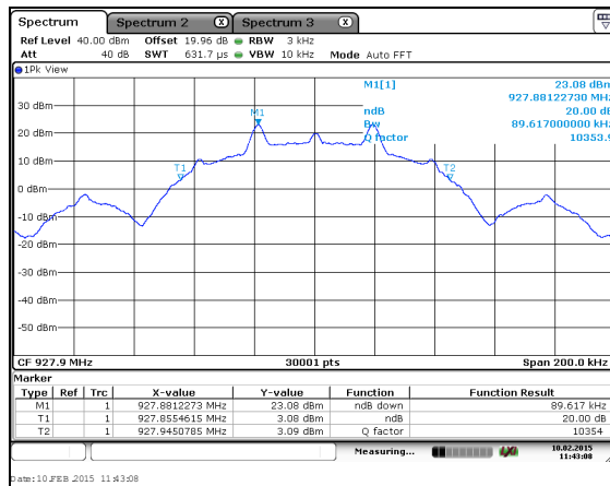
Figure 7.4.4.2-17: 20dB BW High Channel – 38.4kbps
