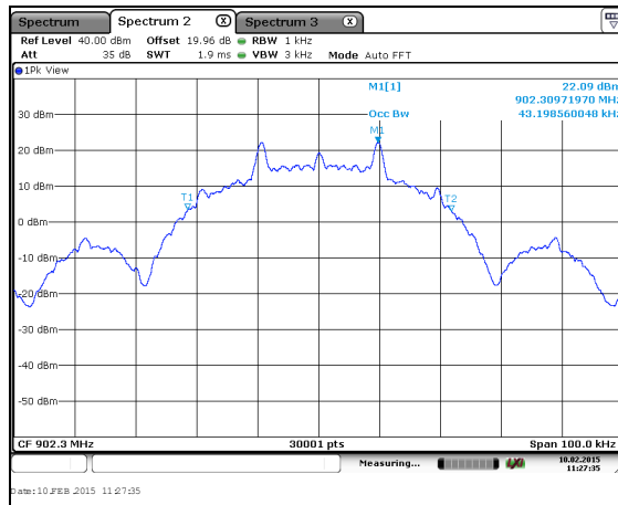
Figure 7.4.4.2-23: 99% BW Low Channel – 19.2kbps
