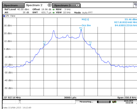
Figure 7.4.4.2-39: 99% BW High Channel – 50.0kbps
