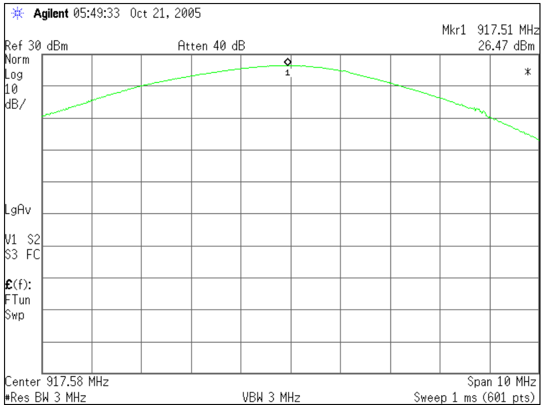
Figure 7.5.2-1: Output power
