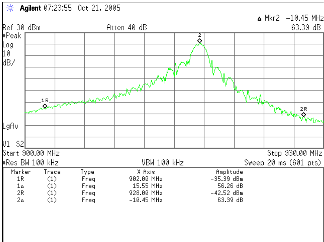
Figure 7.6.1.2-1: Band-edge
