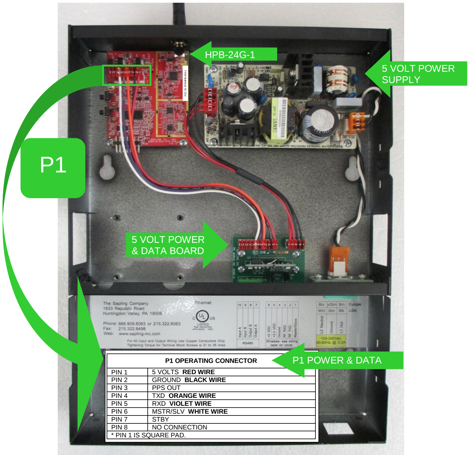
Repeater
