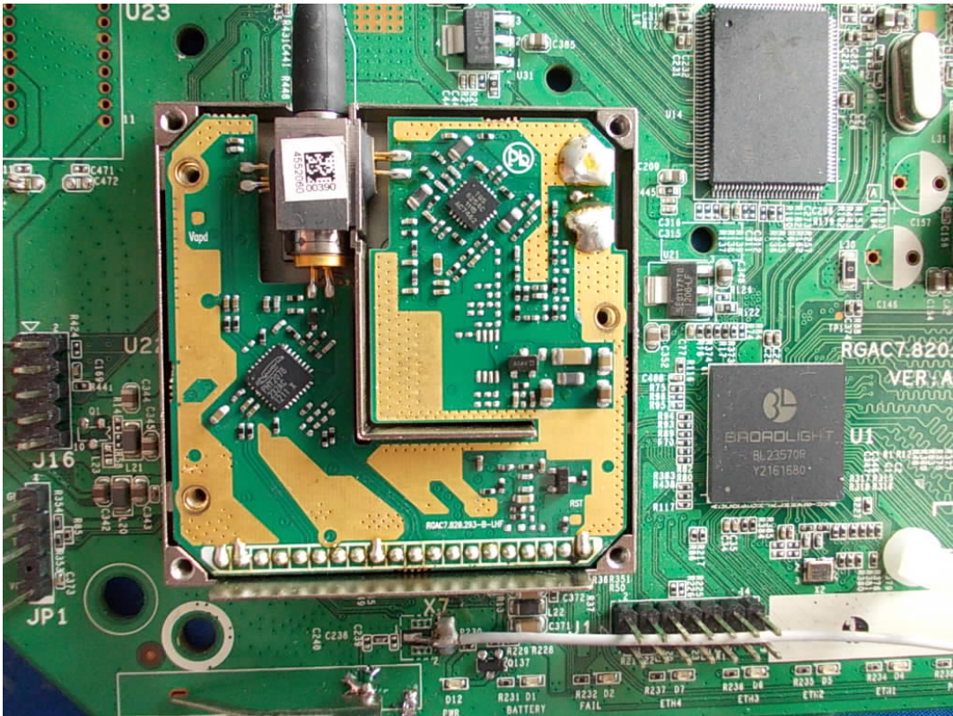
FIGURE 14 GPON SFU (M/N: 7259G) OPTICAL MODULE (COVER REMOVED)
