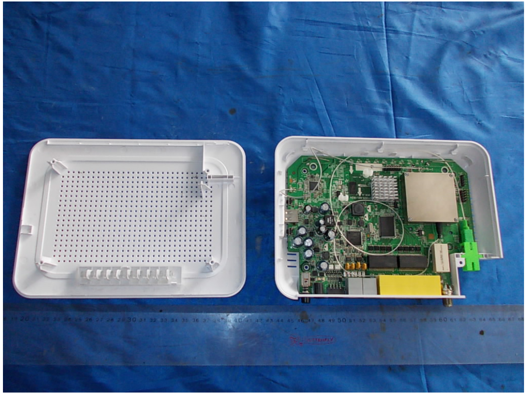
FIGURE 5 GPON SFU (M/N: 7259G) COVER REMOVED
