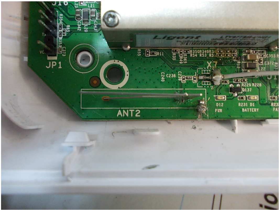
FIGURE 12 GPON SFU (M/N: 7259G) ANT2
