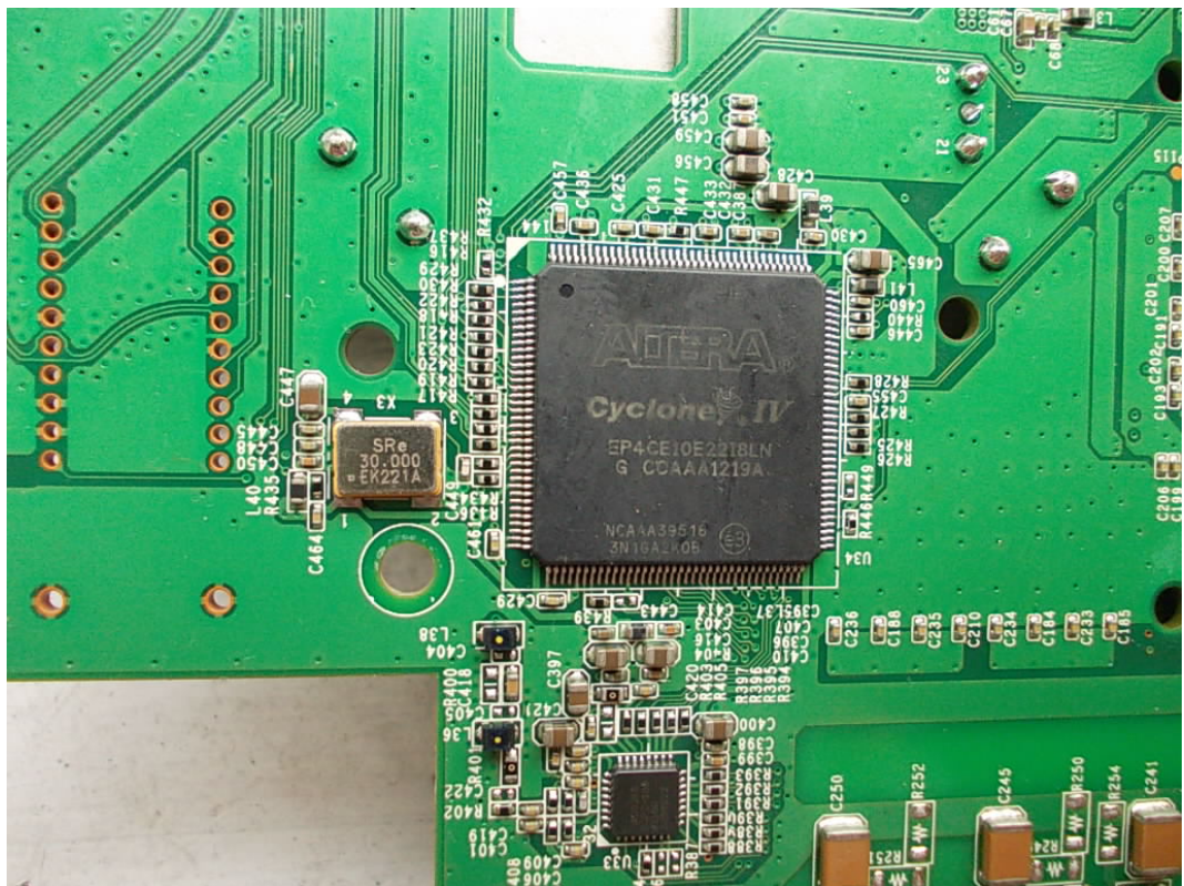
FIGURE 9 GPON SFU (M/N: 7259G) CHIPS AND CRYSTAL #2 ON MAIN BOARD
