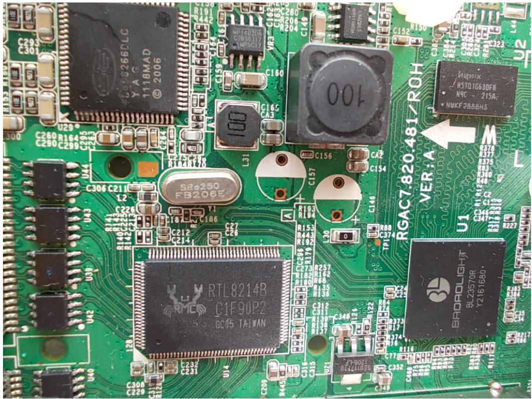
FIGURE 8 GPON SFU (M/N: 7259G) CHIPS AND CRYSTAL #1 ON MAIN BOARD
