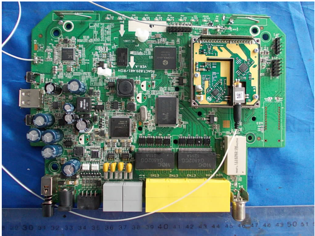
FIGURE 6 GPON SFU (M/N: 7259G) MAIN BOARD (COMPONENT SIDE)
