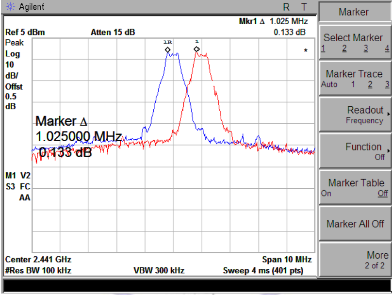
Channel 39 (2441MHz)
