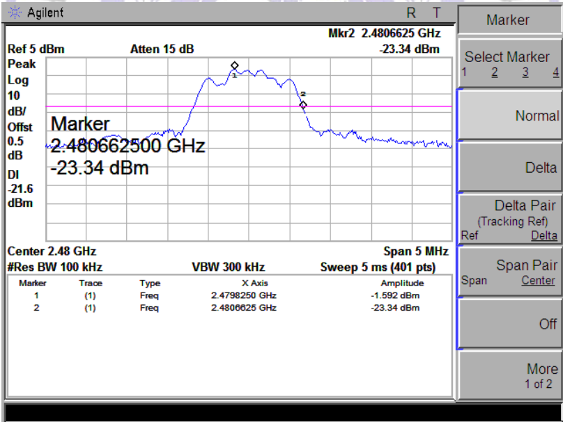
Channel 78 (2480MHz)
