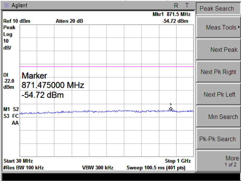
Channel 00 (2402MHz)
