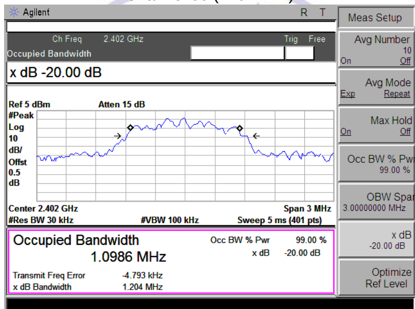
Channel 00 (2402MHz)
