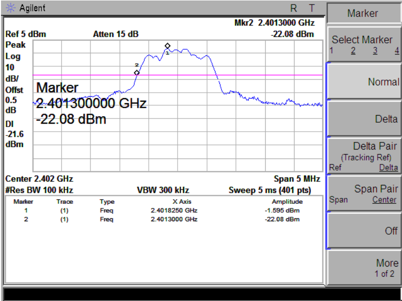
Channel 00 (2402MHz)
