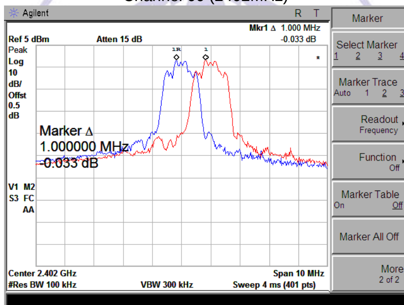
Channel 00 (2402MHz)
