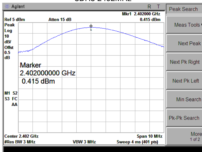
3DH5 2402MHz
