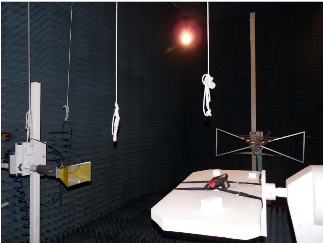
Photo 1: (Part 15c) Test setup for radiated measurements (Enclosure, above 1 GHz)
