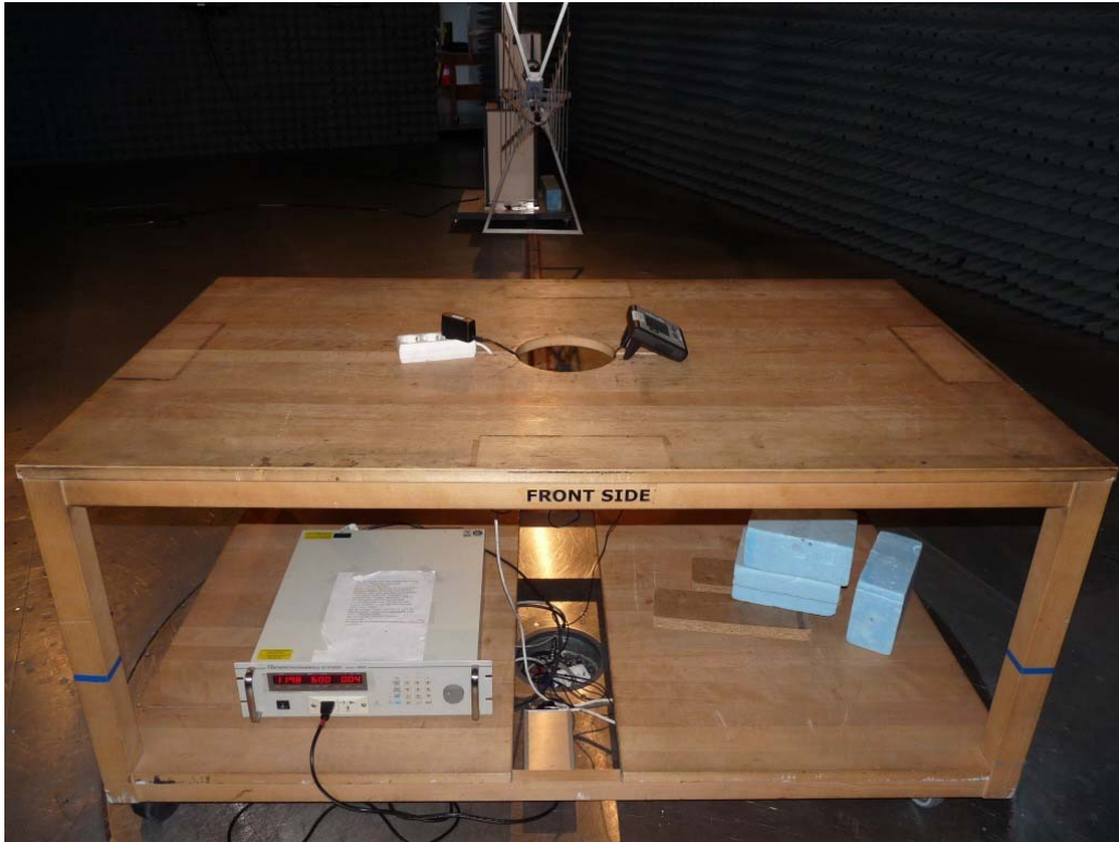
Photo 2: (Part 15c) Test setup for radiated measurements (Enclosure, below 1 GHz)
