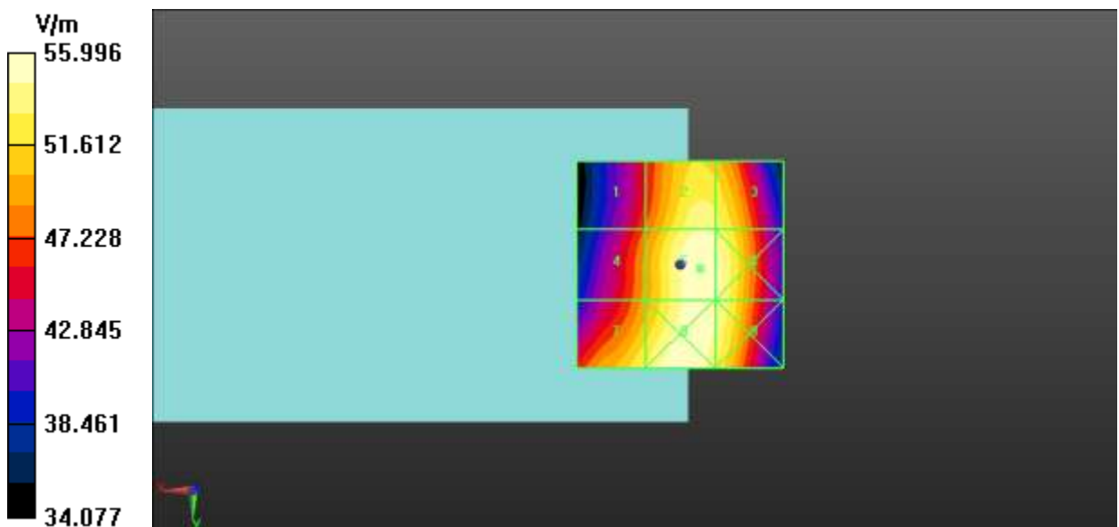
Fig A.15 HAC RF E-Field CDMA BC10
