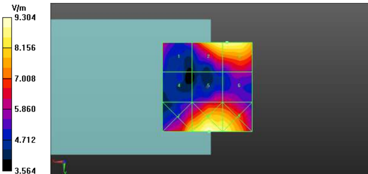
Fig A.20 HAC RF E-Field LTE-Band 41 Low
