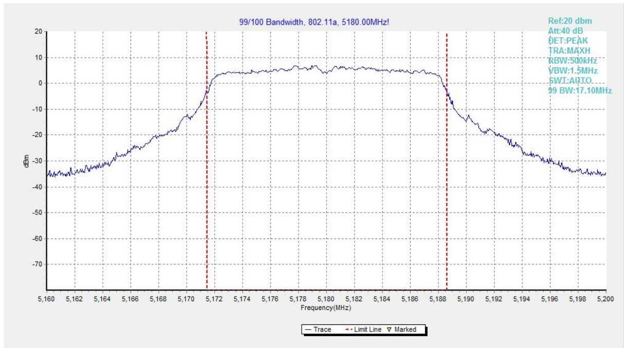
Fig. 39 99% Occupied Bandwidth (802.11a, 5180MHz)
