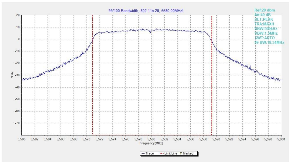
Fig. 55 99% Occupied Bandwidth (802.11n-HT20, 5580MHz)
