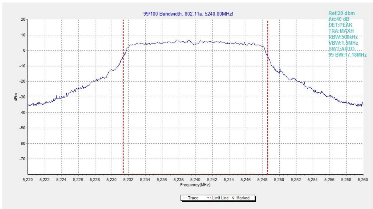
Fig. 41 99% Occupied Bandwidth (802.11a, 5240MHz)
