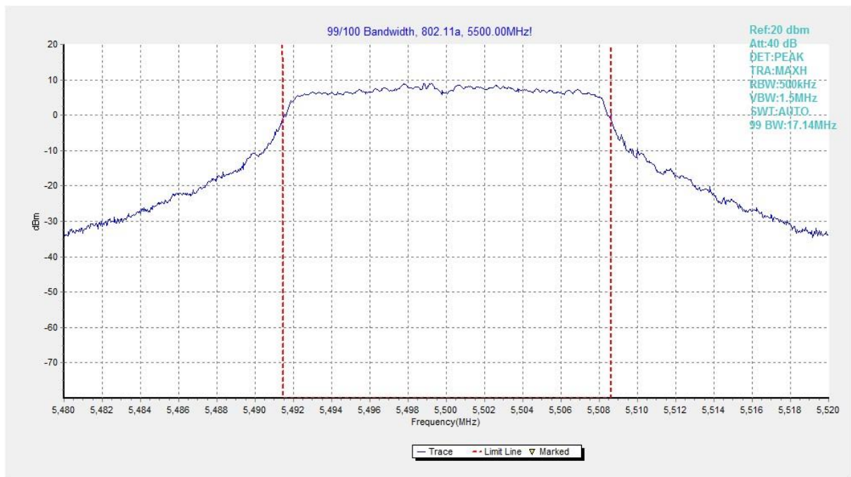
Fig. 45 99% Occupied Bandwidth (802. 11a, 5500MHz)
