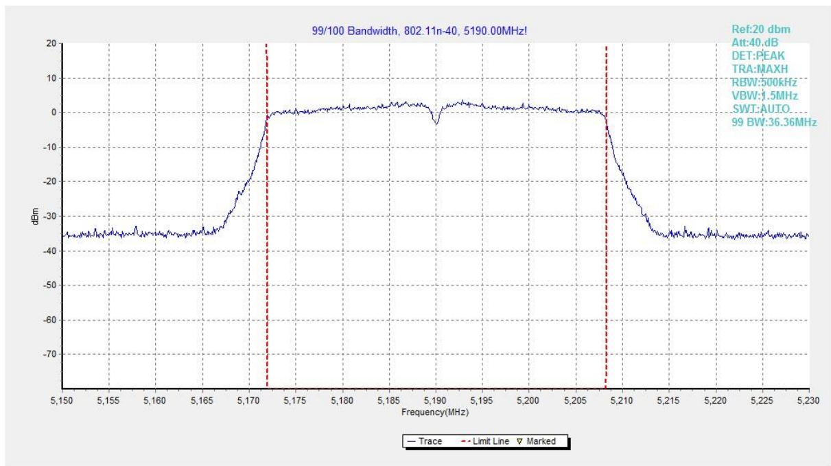
Fig. 57 99% Occupied Bandwidth (802.11n-HT40, 5190MHz)
