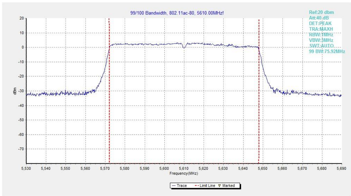
Fig. 67 99% Occupied Bandwidth (802.11ac-VHT80, 5610MHz)
