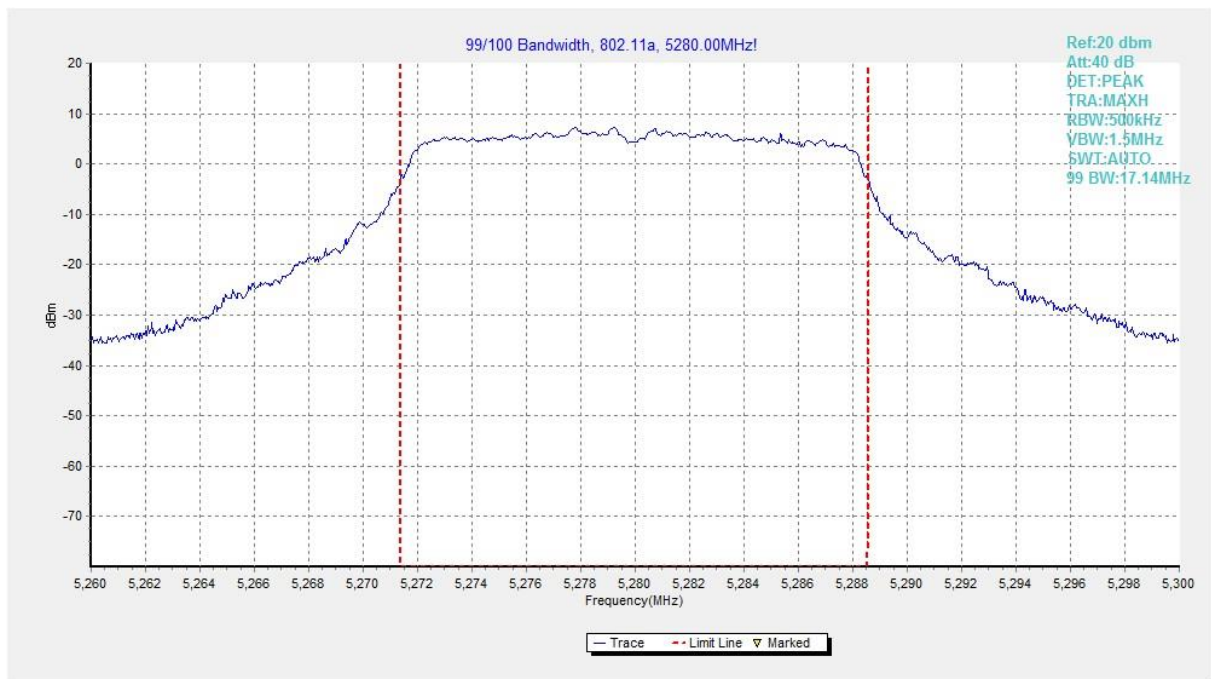
Fig. 43 99% Occupied Bandwidth (802.11a, 5280MHz)
