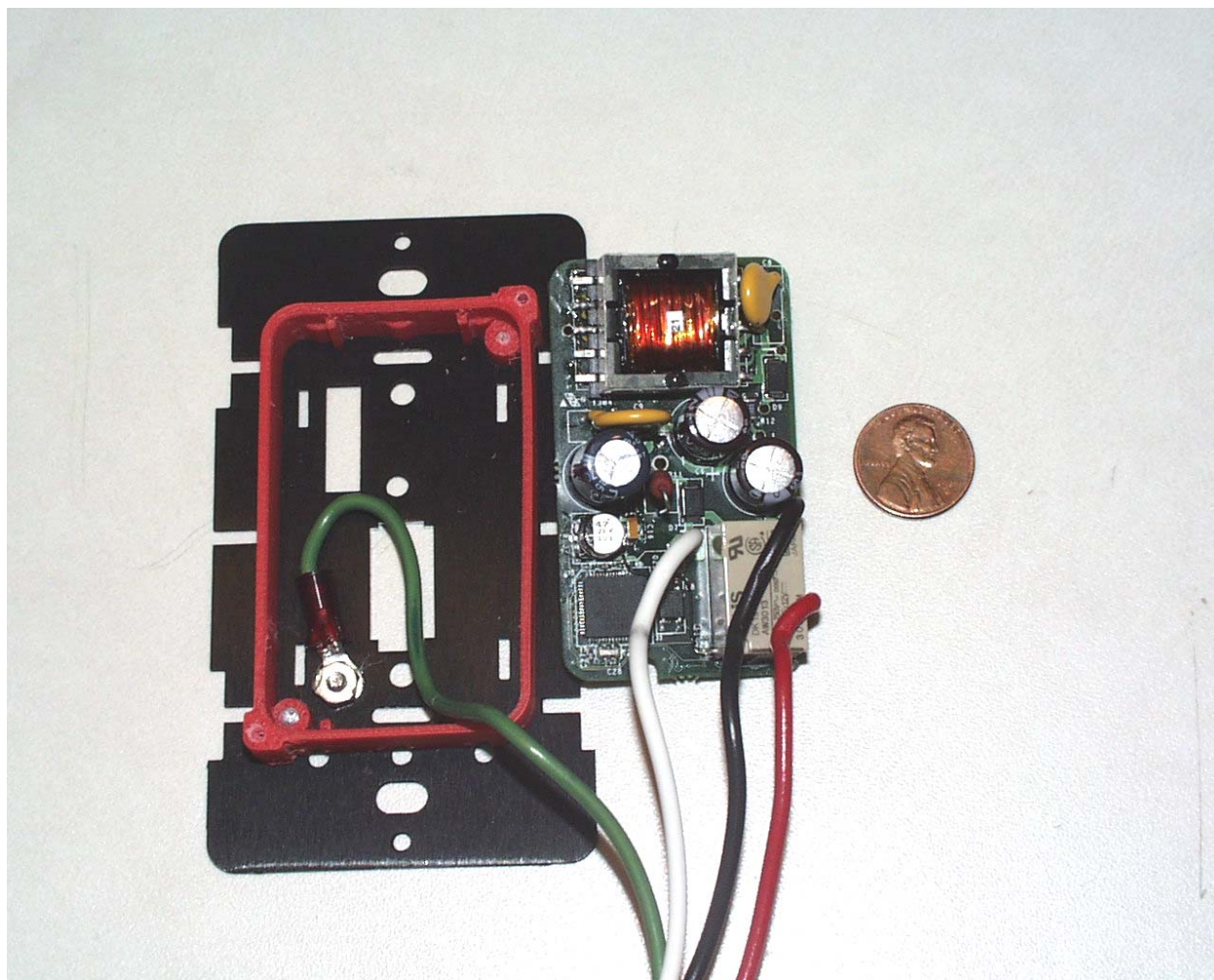
Photograph 7 - View of the Component Side of the Host Card
