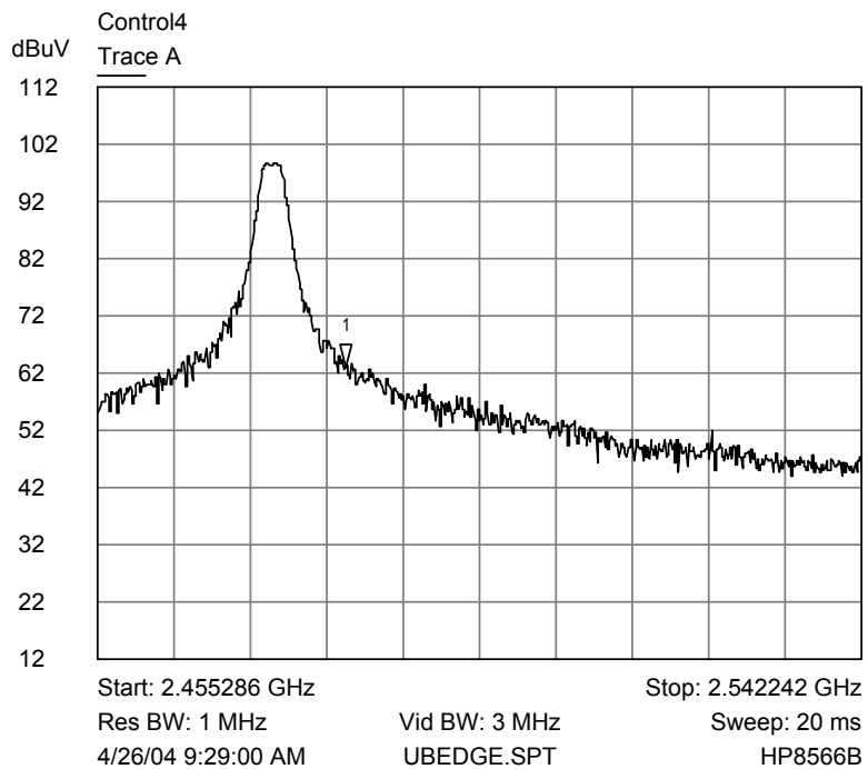
Upper Band Edge, Peak Measurement
