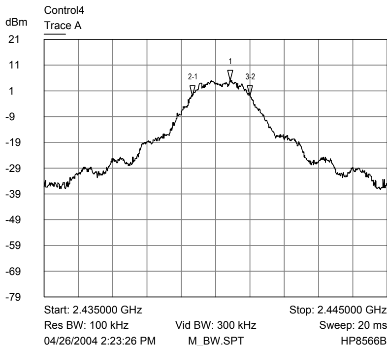
Middle channel bandwidth
