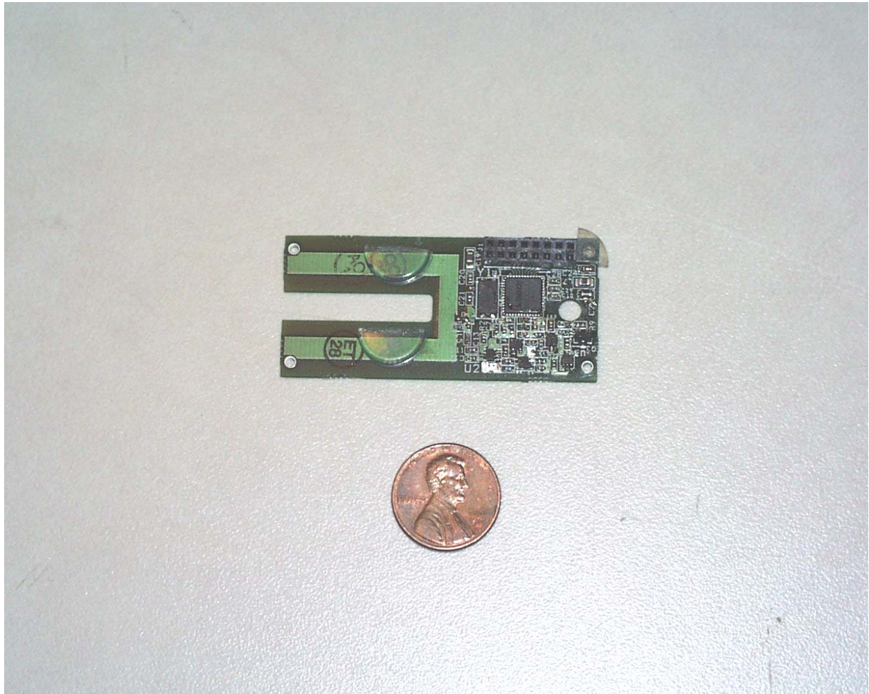
Photograph 9 - View of the Component Side of the Transceiver Card
