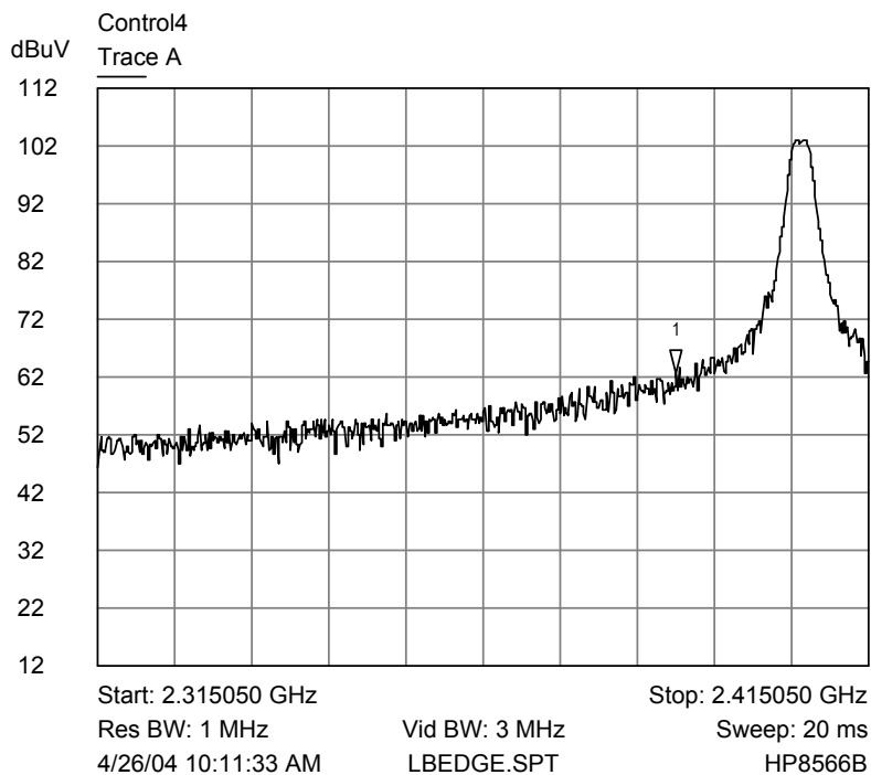
Lower Band Edge, Peak Measurement
