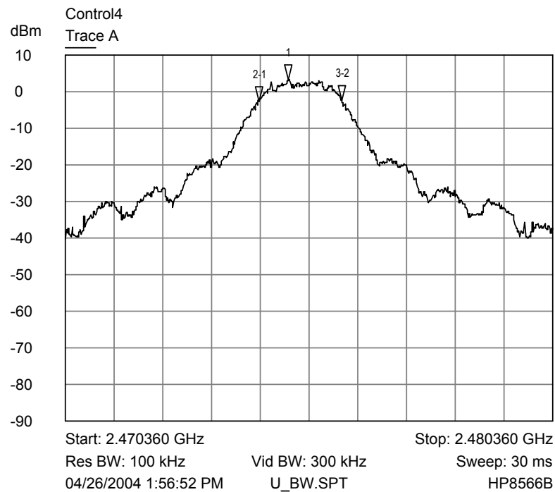
Upper channel bandwidth
