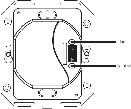
Figure 1. Keypad wiring
