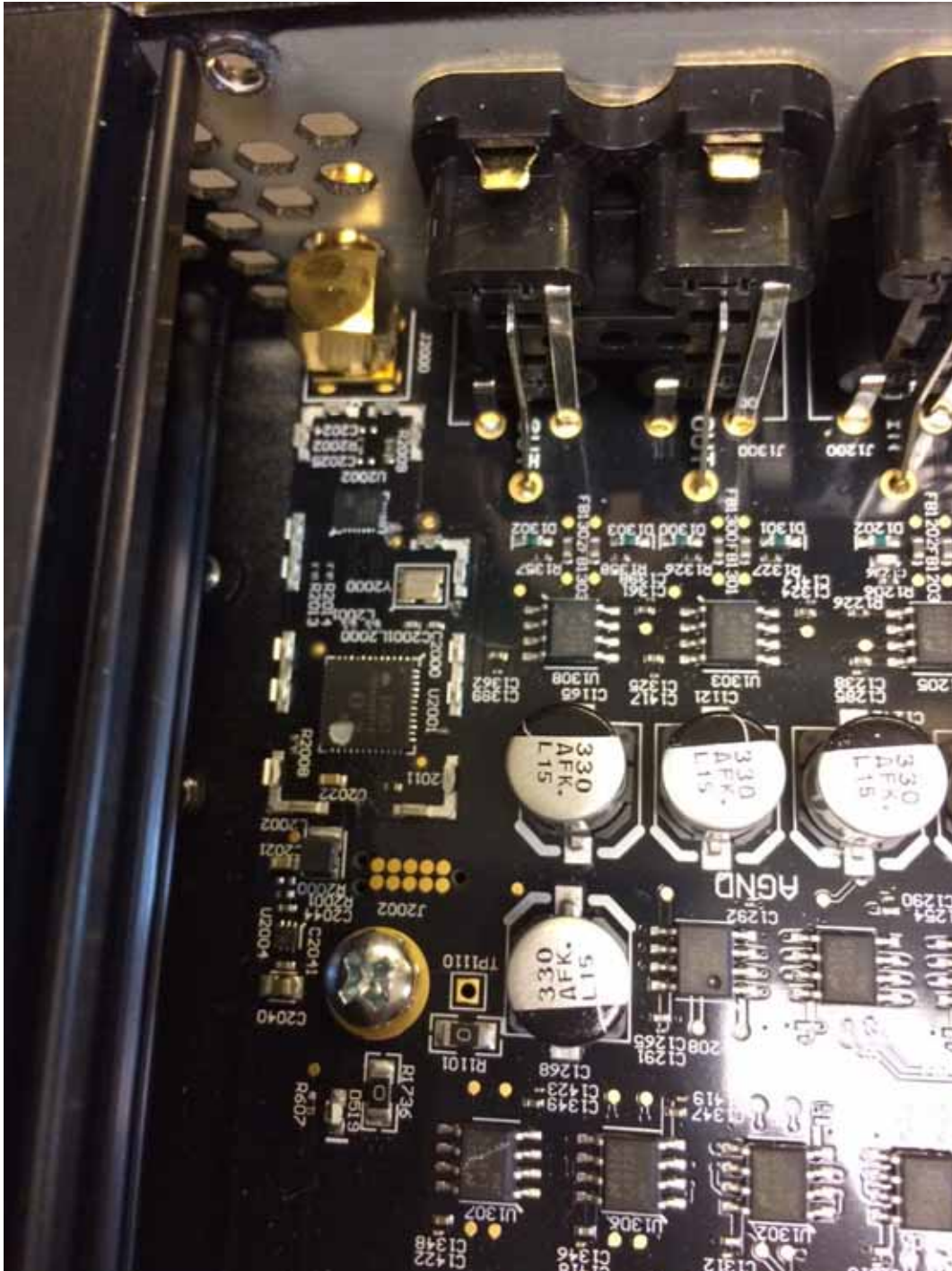
Photograph 10 – View of the Circuitry of the 802.15.4 Transceiver with RF Shield Removed
