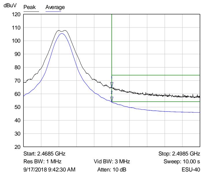
Graph 2: Radiated Upper Band Edge Plot (2470 MHz)
