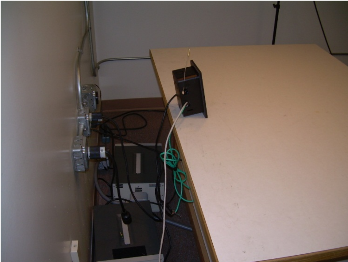
Photograph 11 – Back View Conducted Disturbance – AC Power
