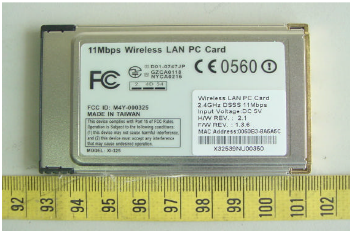
Bottom View of Wireless LAN Card
