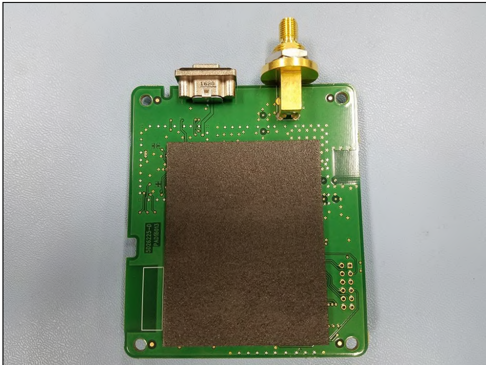
Figure 3: PCB - Back
