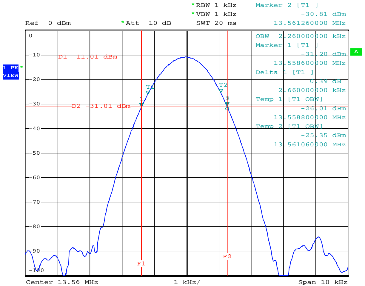
20 dB Bandwidth Plot on 13.56 MHz
