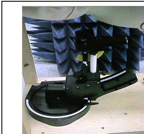
Figure 3. Device Holder
